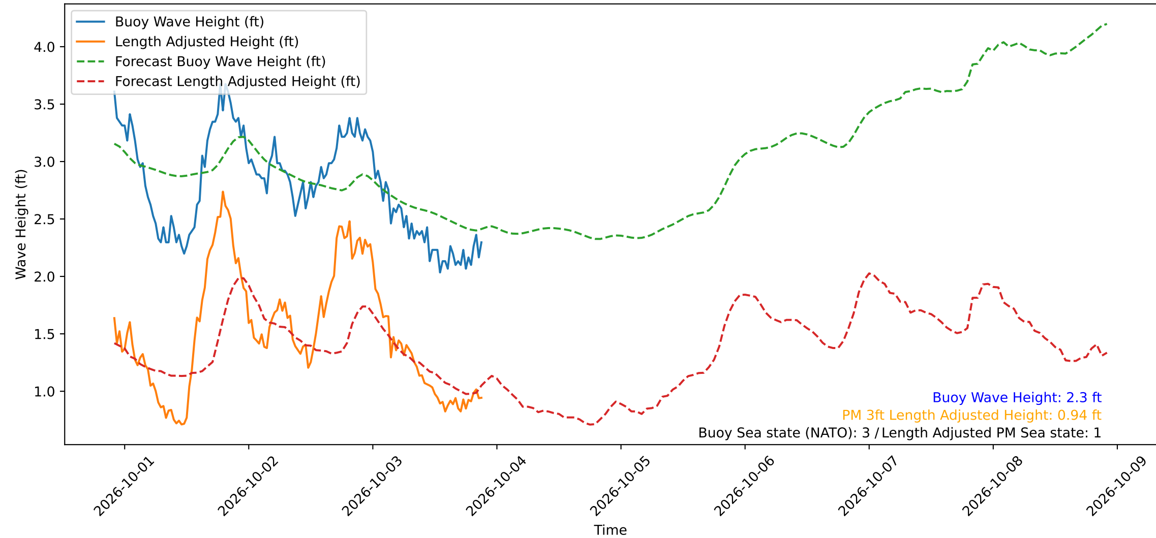
Wave Heights over Time for Green Beach at 2026-10-03 21:41:11
