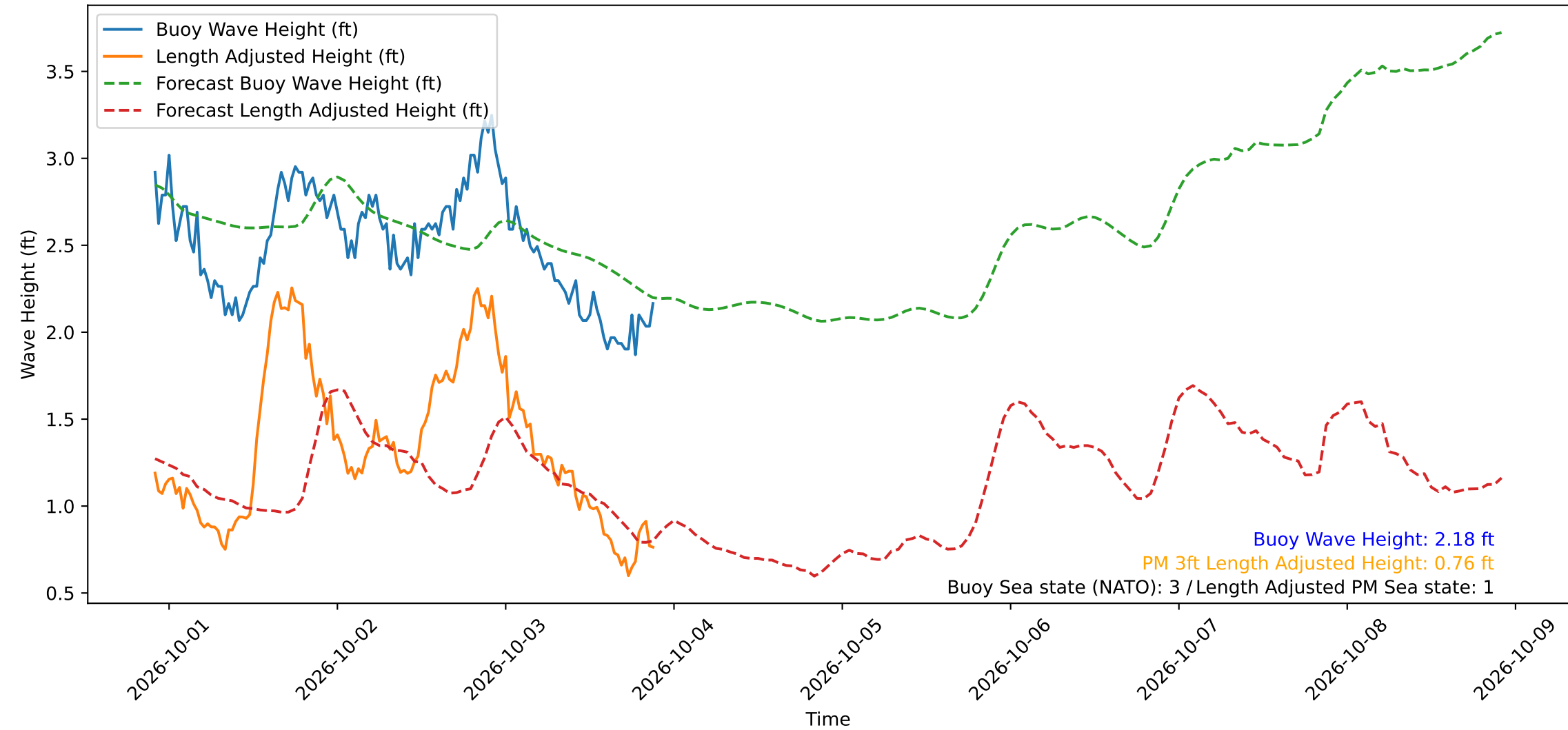
Wave Heights over Time for Red Beach at 2026-10-03 21:40:49
