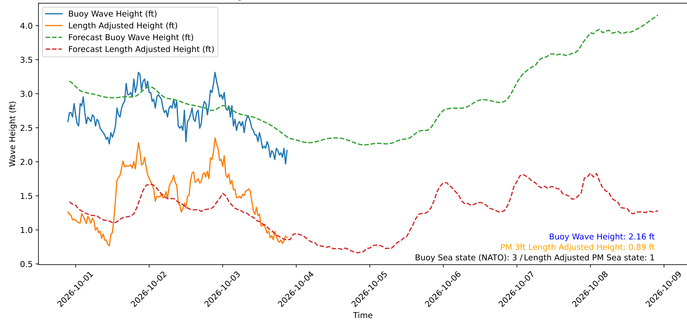
Wave Heights over Time for Oceanside Harbor at 2026-10-03 21:40:29
