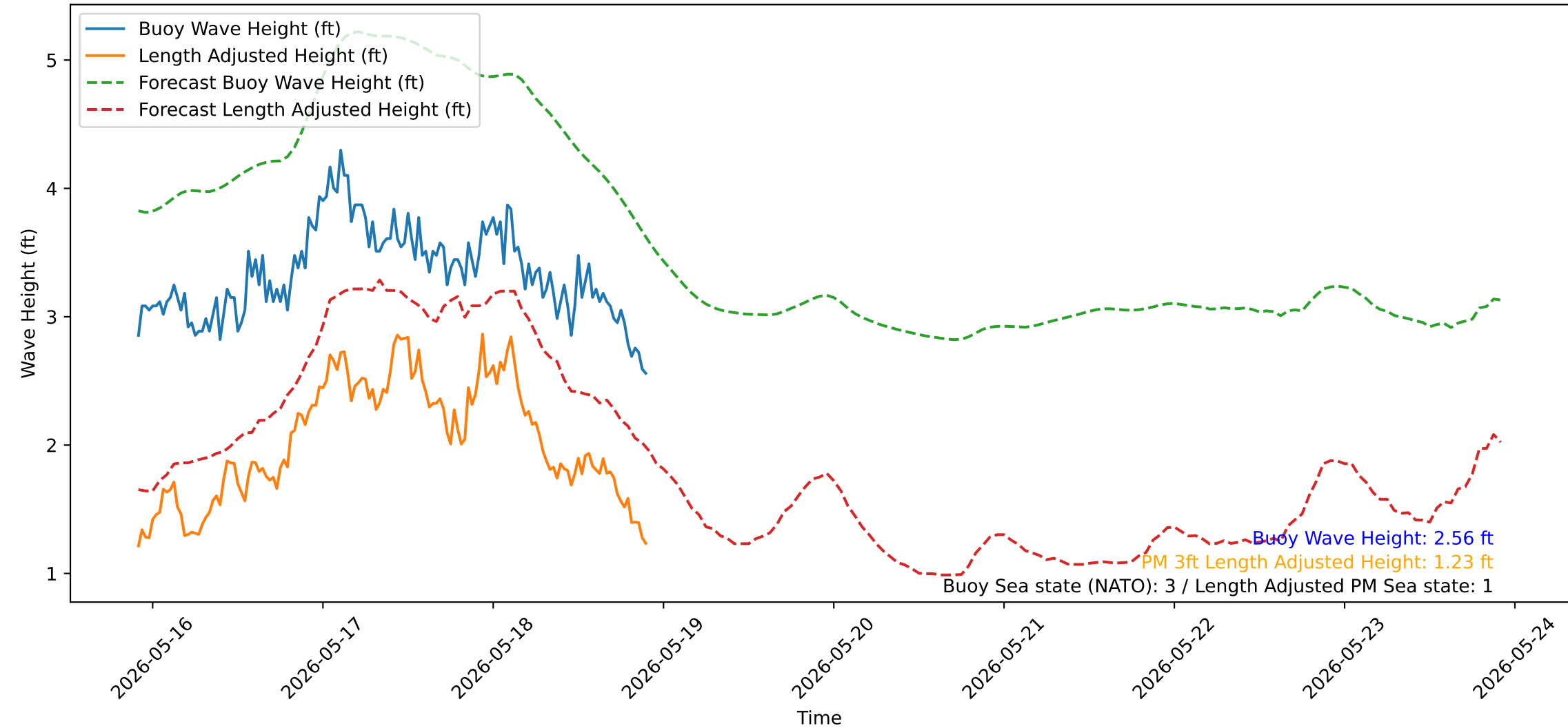
Wave Heights over Time for Oceanside Harbor at 2026-05-18 22:10:32
