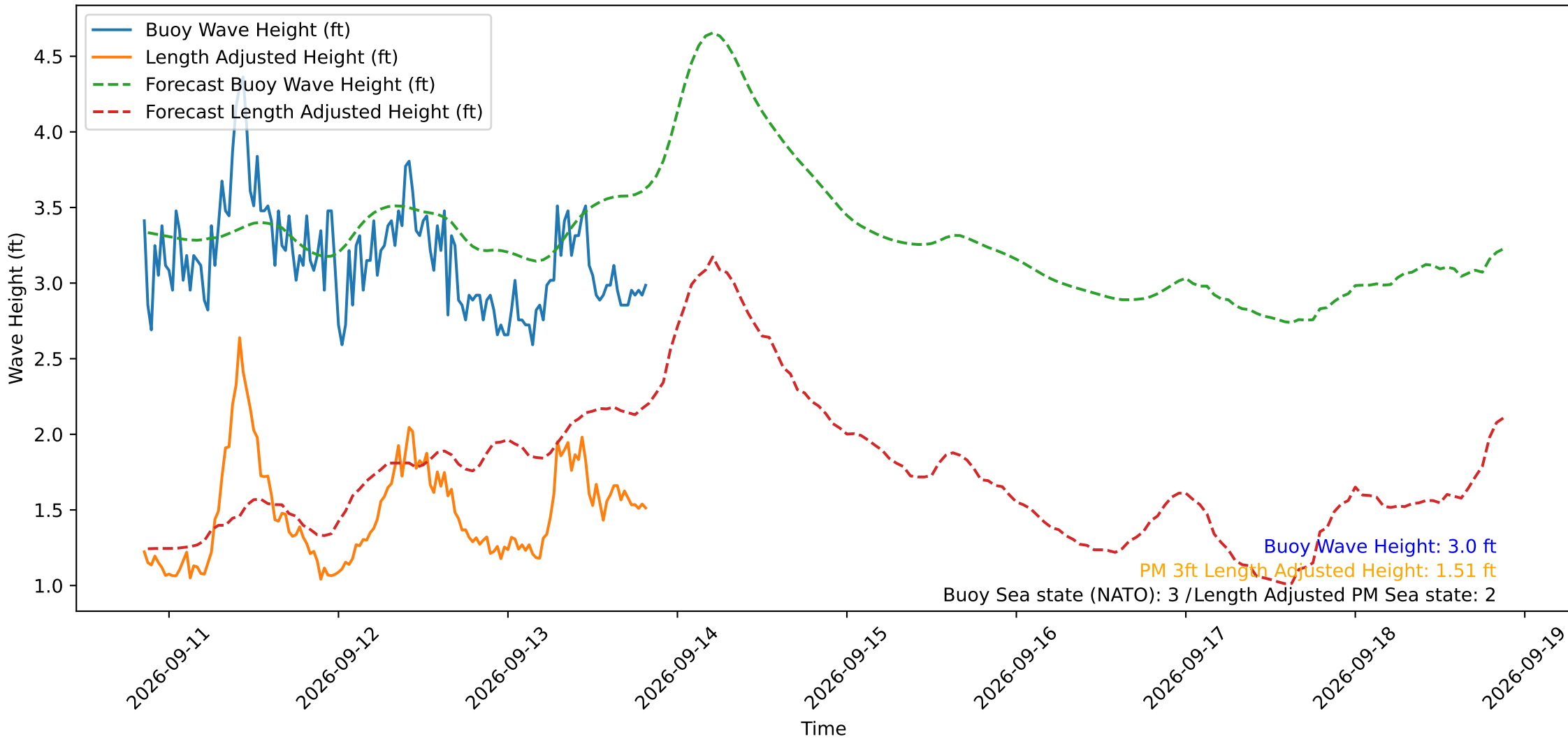
Wave Heights over Time for Oceanside Harbor at 2026-09-13 20:30:29
