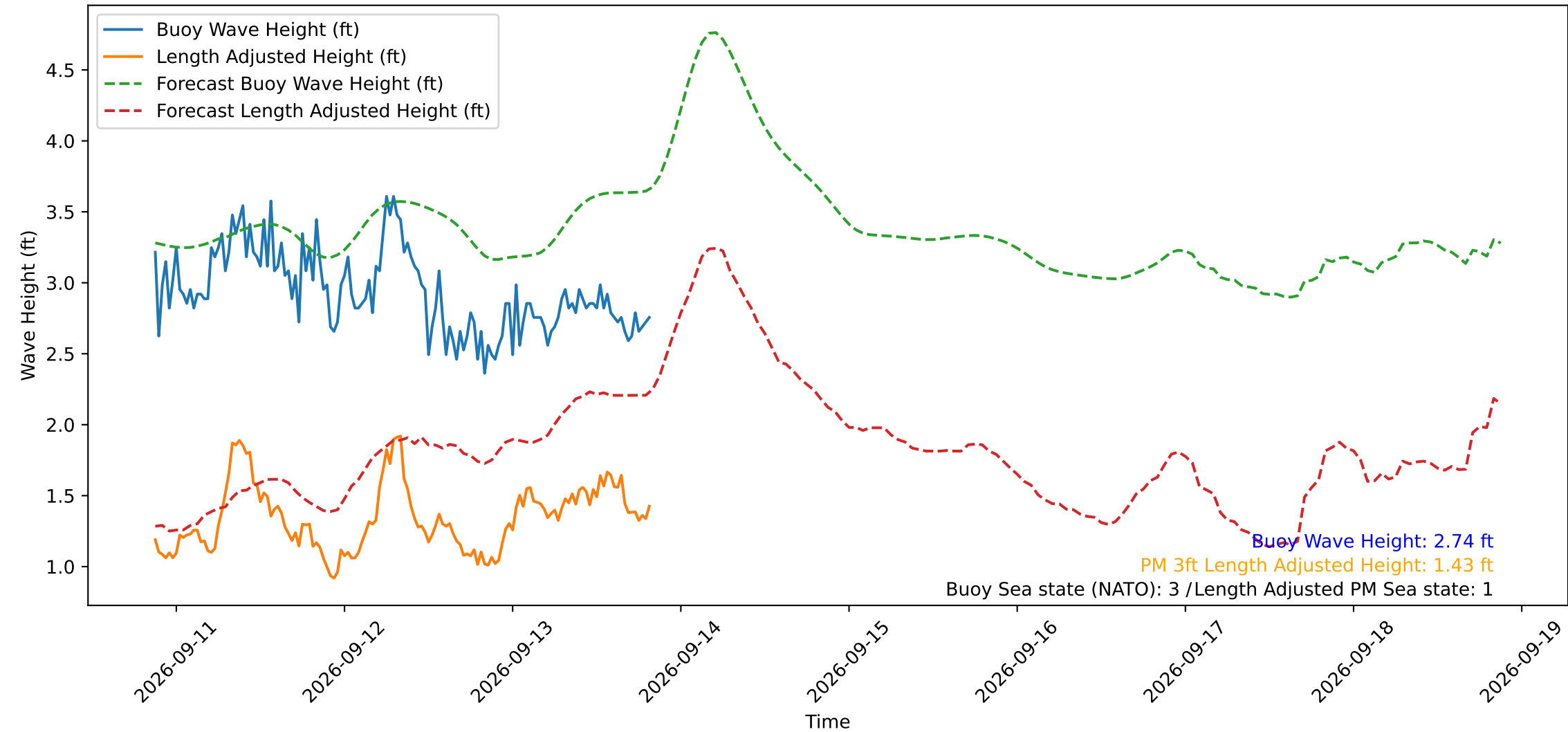
Wave Heights over Time for Green Beach at 2026-09-13 20:31:11
