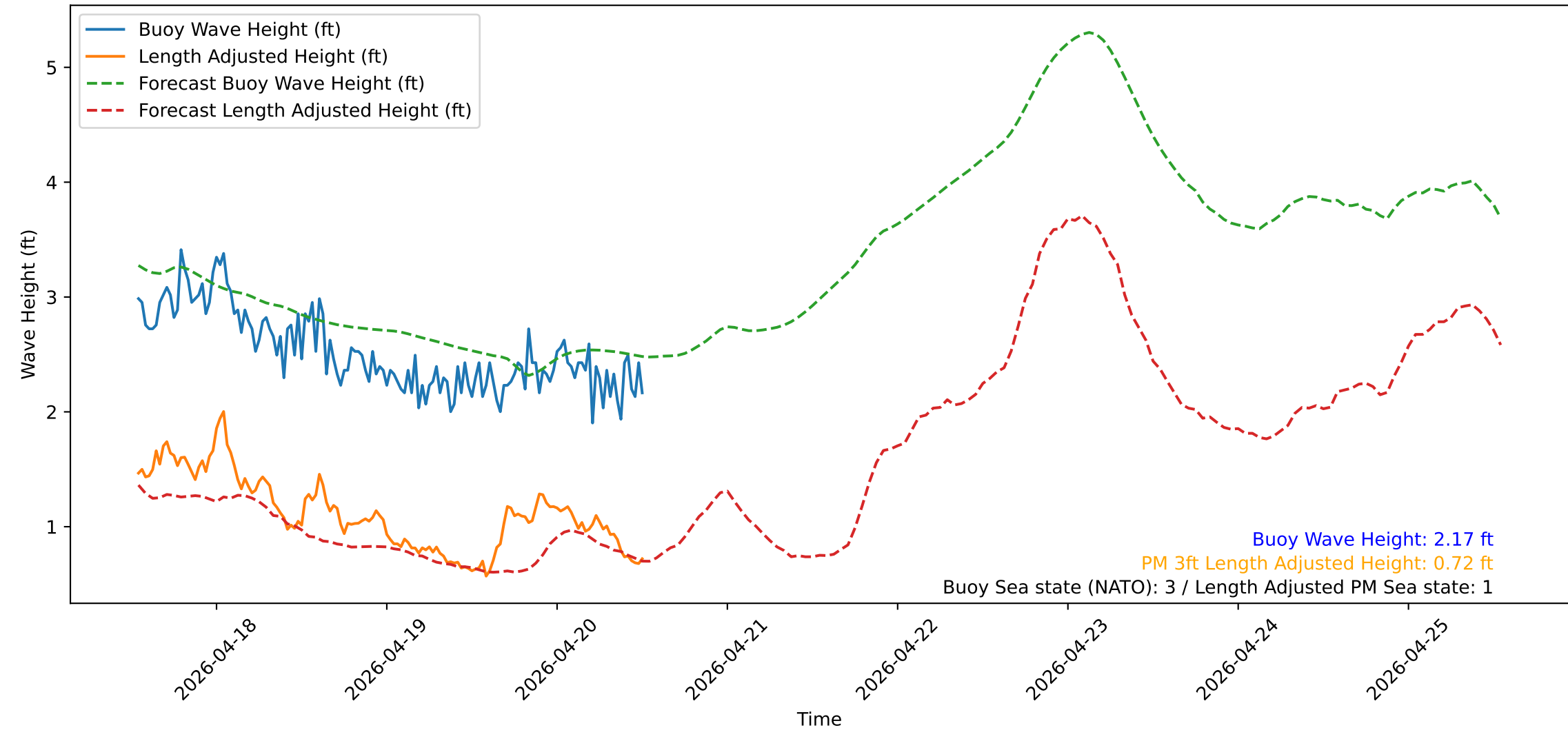
Wave Heights over Time for Oceanside Harbor at 2026-04-20 13:00:31
