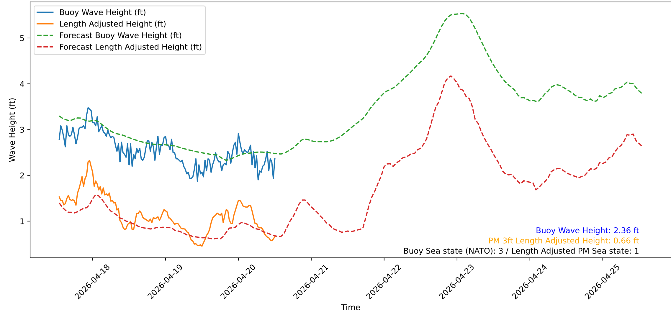
Wave Heights over Time for Green Beach at 2026-04-20 13:01:13
