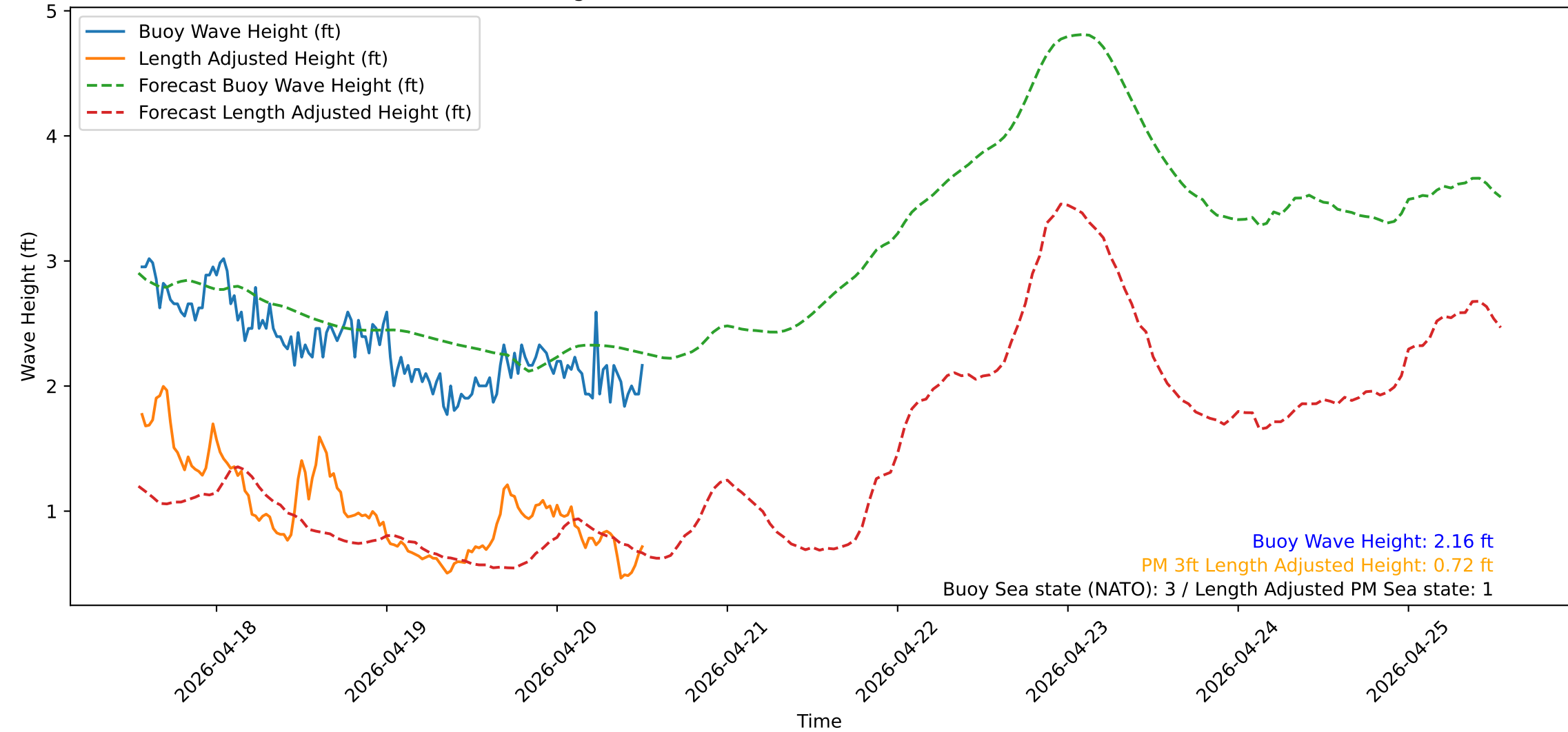
Wave Heights over Time for Red Beach at 2026-04-20 13:00:50
