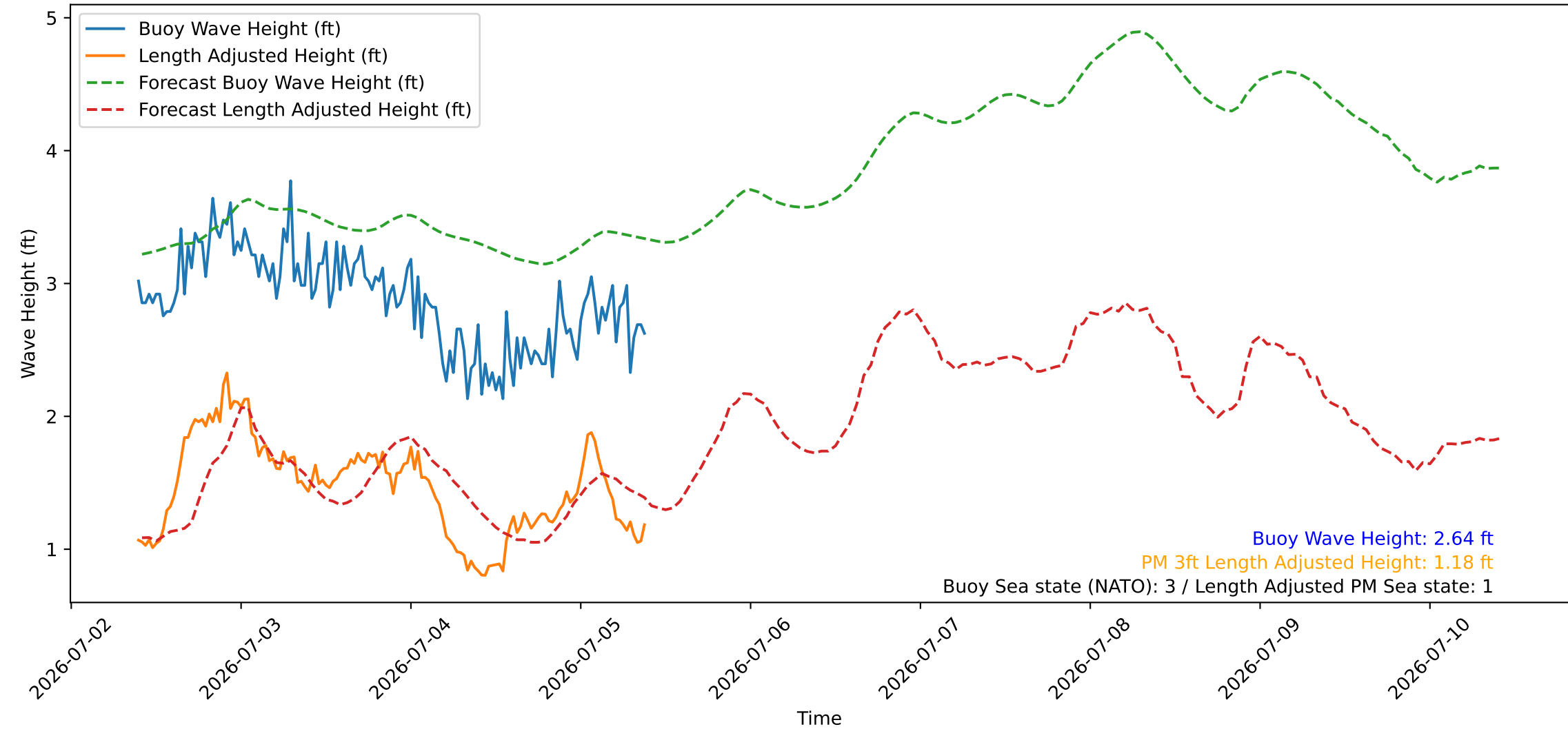
Wave Heights over Time for Oceanside Harbor at 2026-07-05 09:30:27
