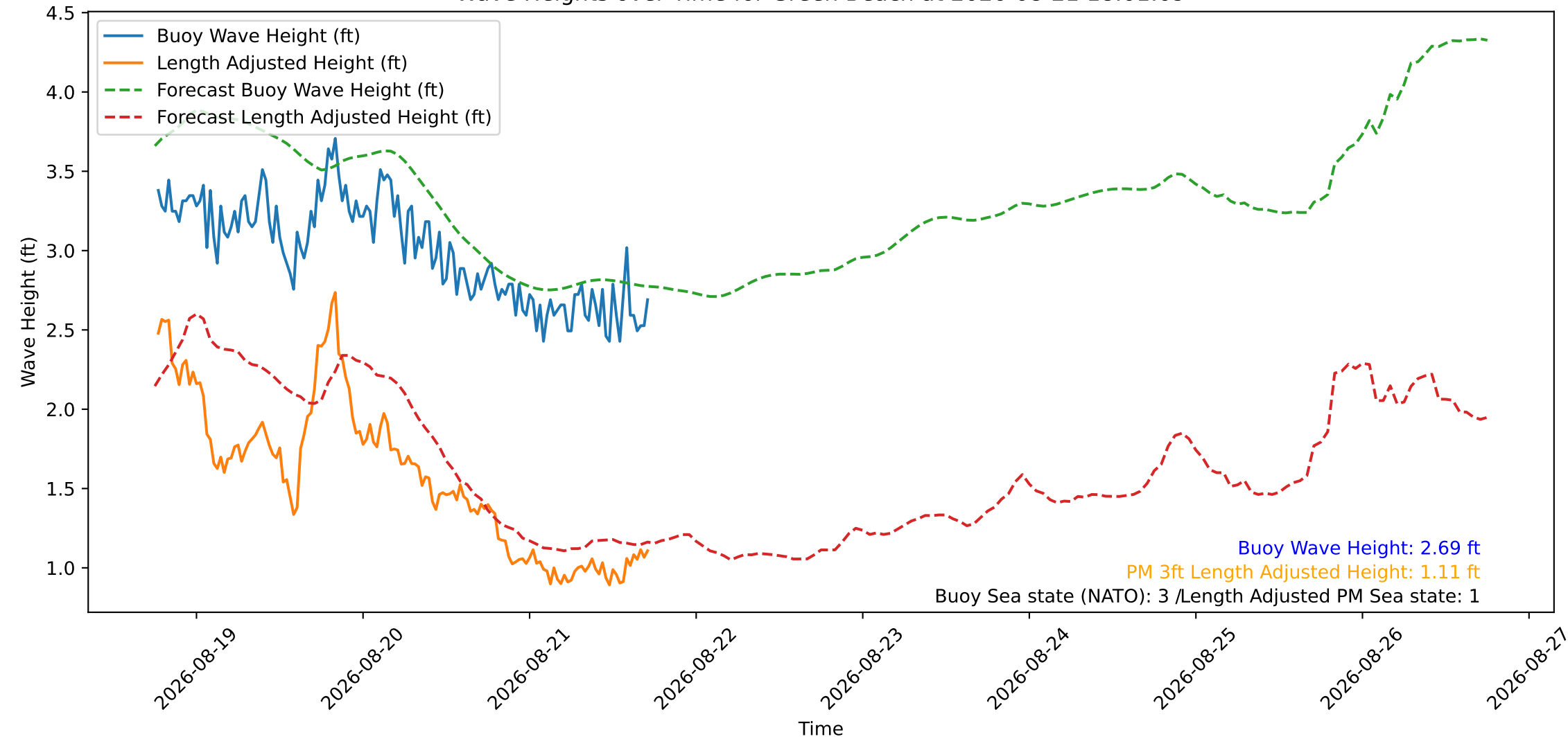
Wave Heights over Time for Green Beach at 2026-08-21 18:01:09
