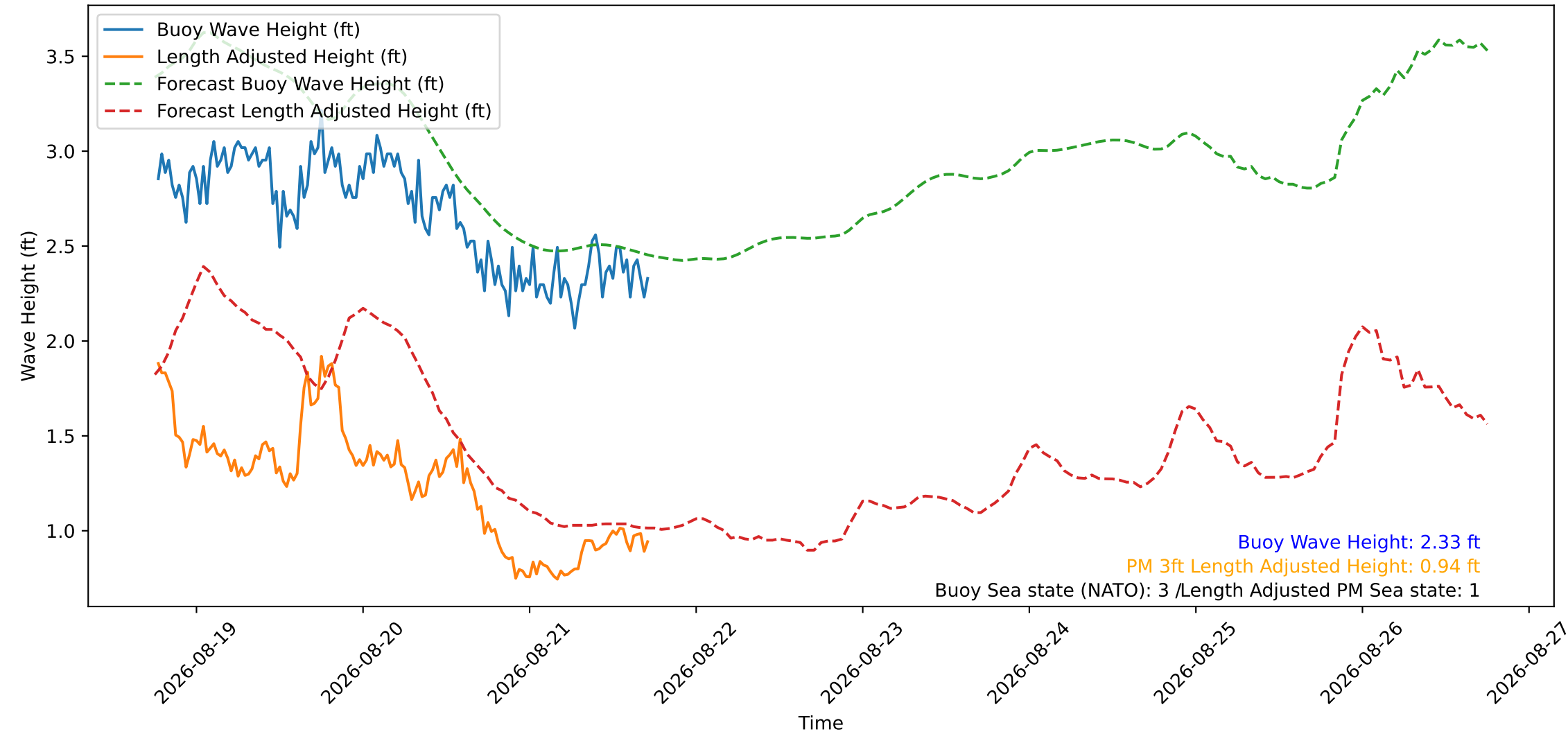
Wave Heights over Time for Red Beach at 2026-08-21 18:00:46
