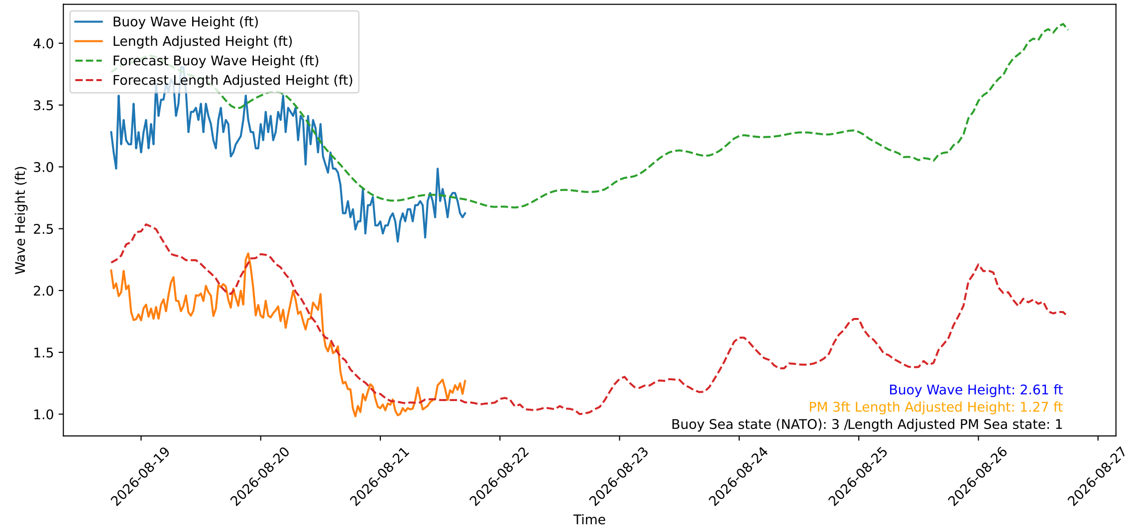
Wave Heights over Time for Oceanside Harbor at 2026-08-21 18:00:26
