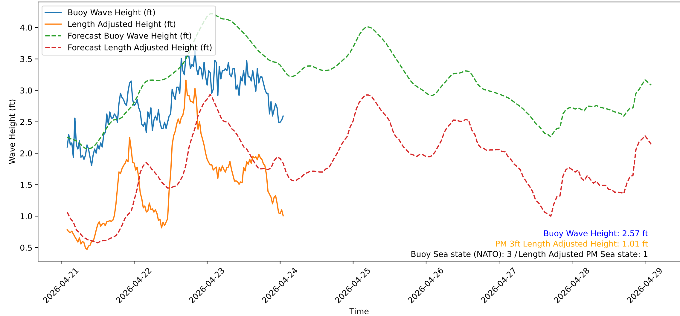
Wave Heights over Time for Red Beach at 2026-04-24 01:40:50
