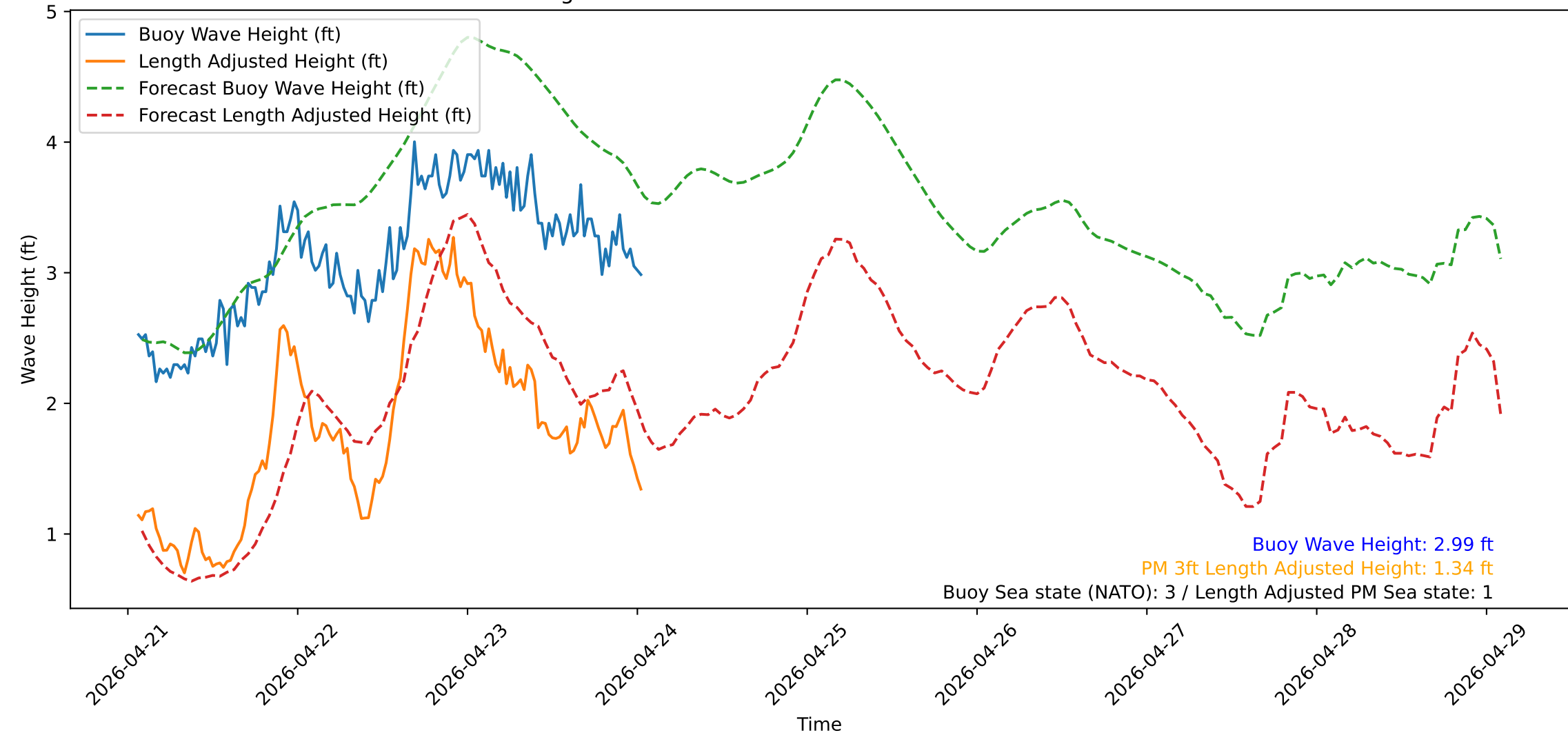
Wave Heights over Time for Green Beach at 2026-04-24 01:41:12
