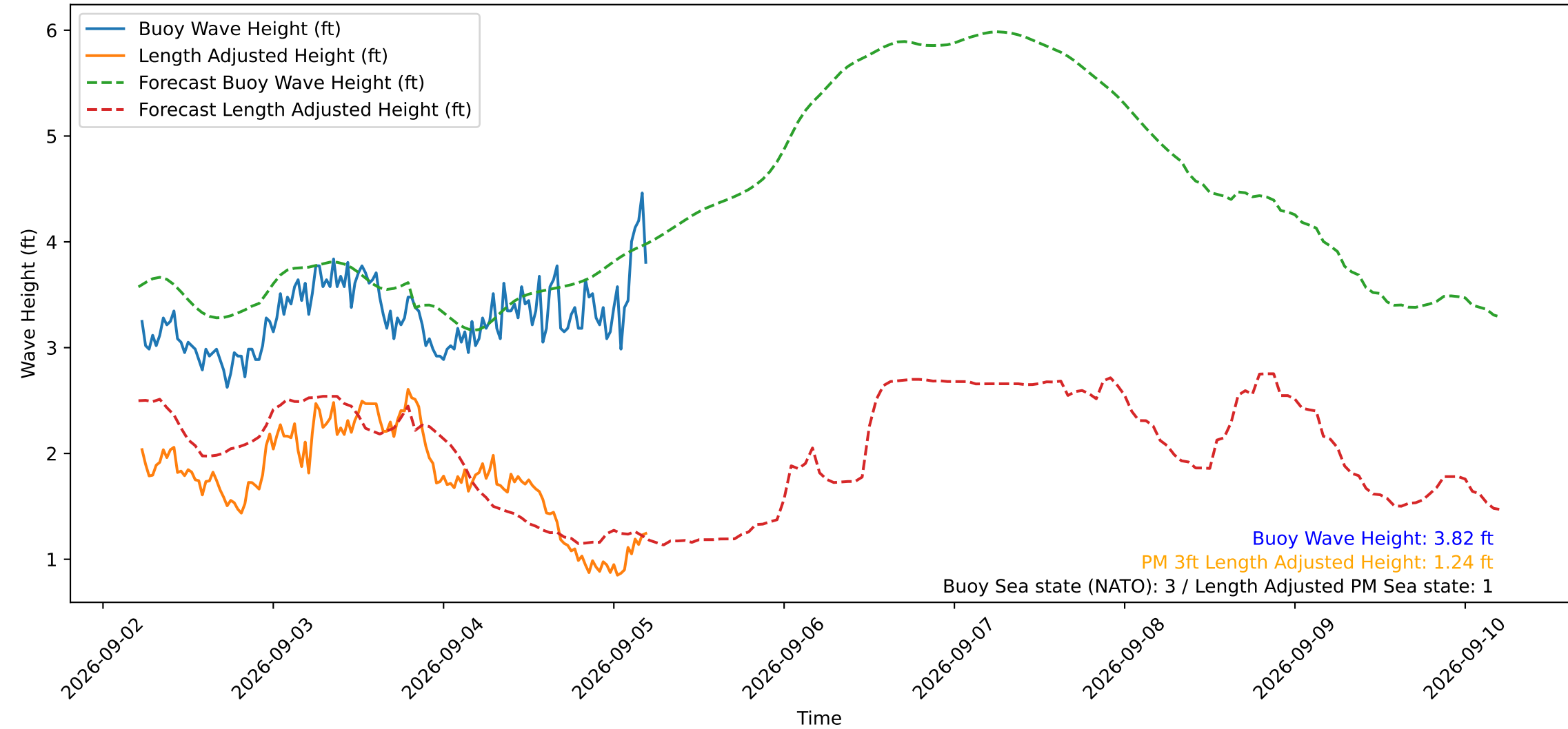
Wave Heights over Time for Oceanside Harbor at 2026-09-05 05:20:30
