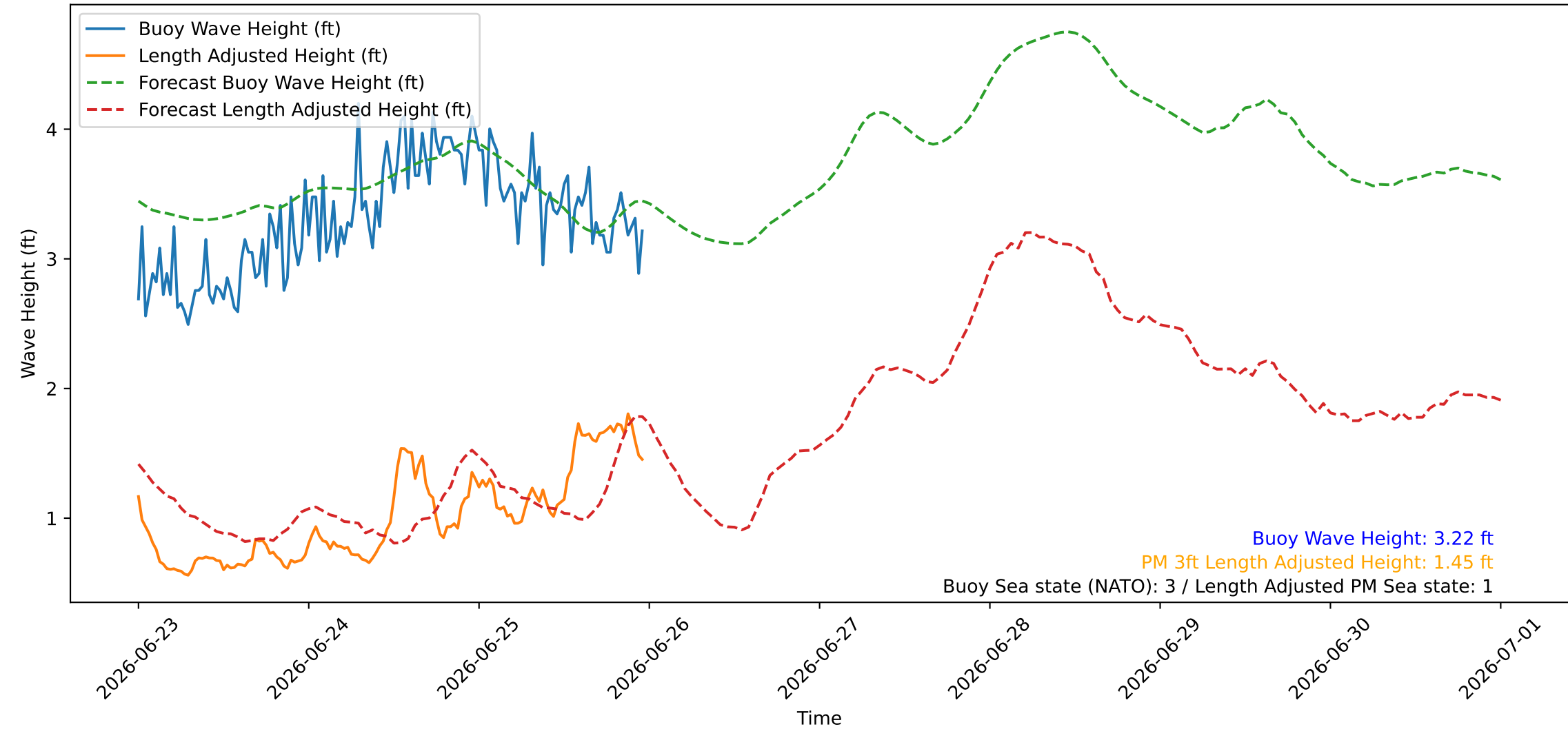
Wave Heights over Time for Green Beach at 2026-06-26 00:01:07
