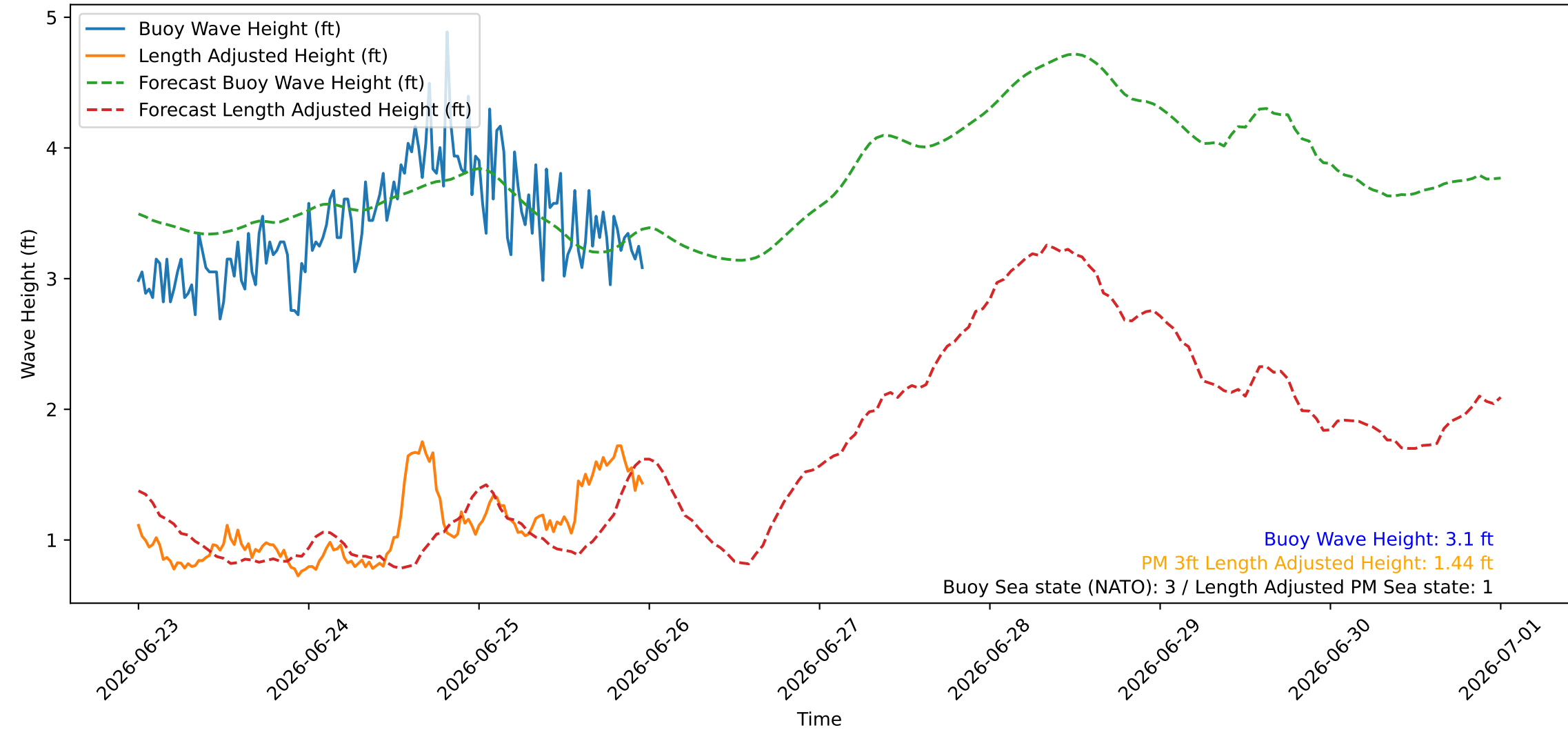
Wave Heights over Time for Oceanside Harbor at 2026-06-26 00:00:26
