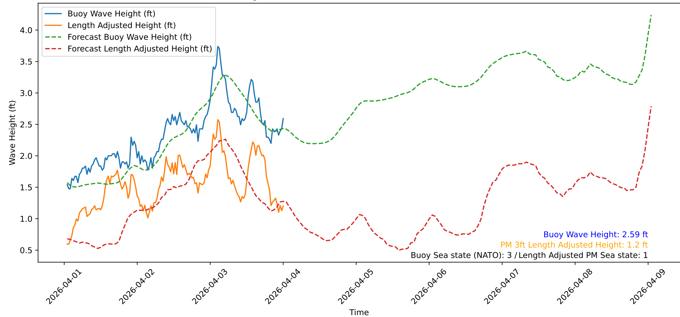
Wave Heights over Time for Red Beach at 2026-04-04 00:50:48
