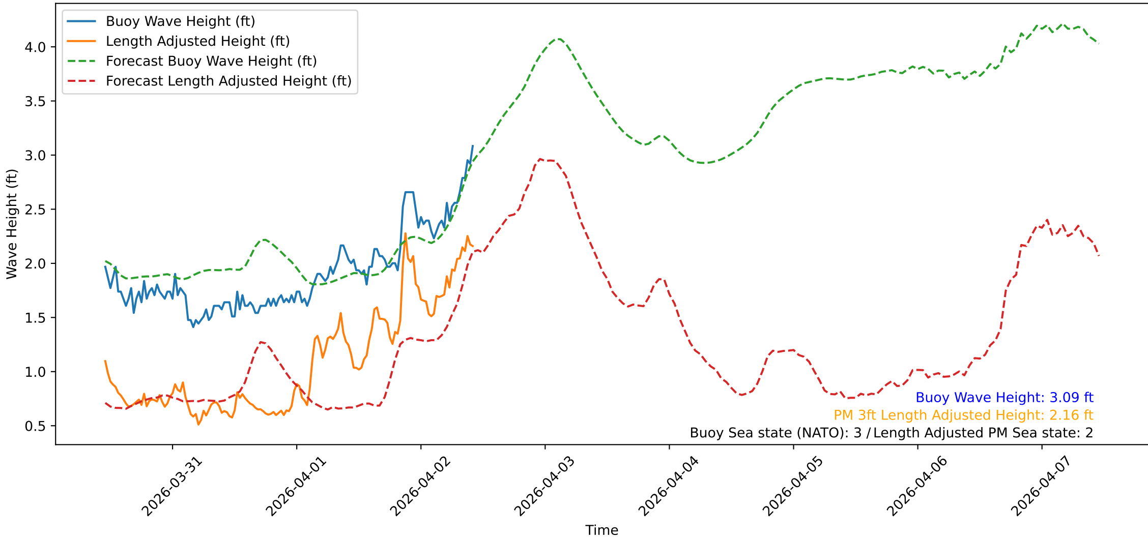
Wave Heights over Time for Green Beach at 2026-04-02 10:51:09
