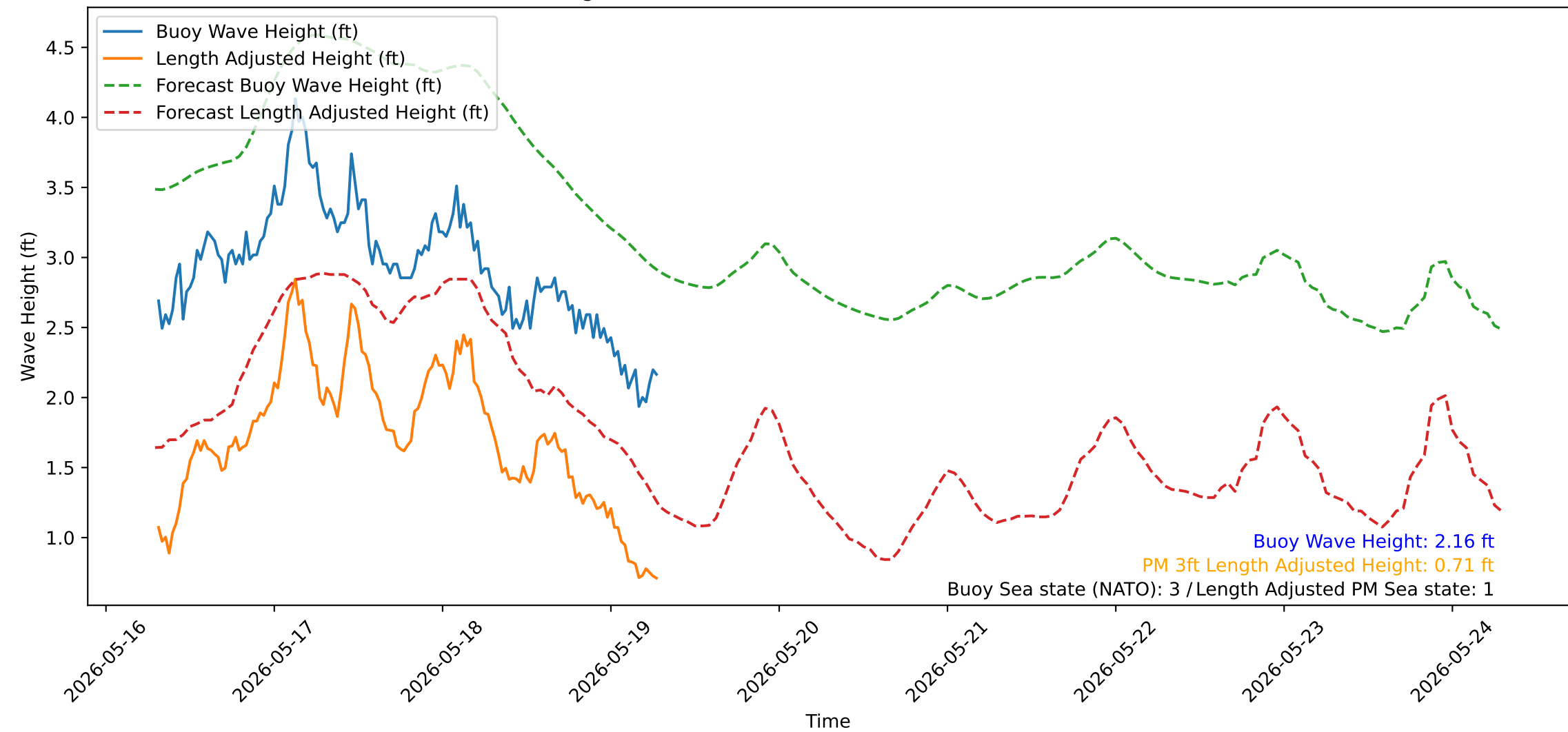
Wave Heights over Time for Red Beach at 2026-05-19 07:20:52
