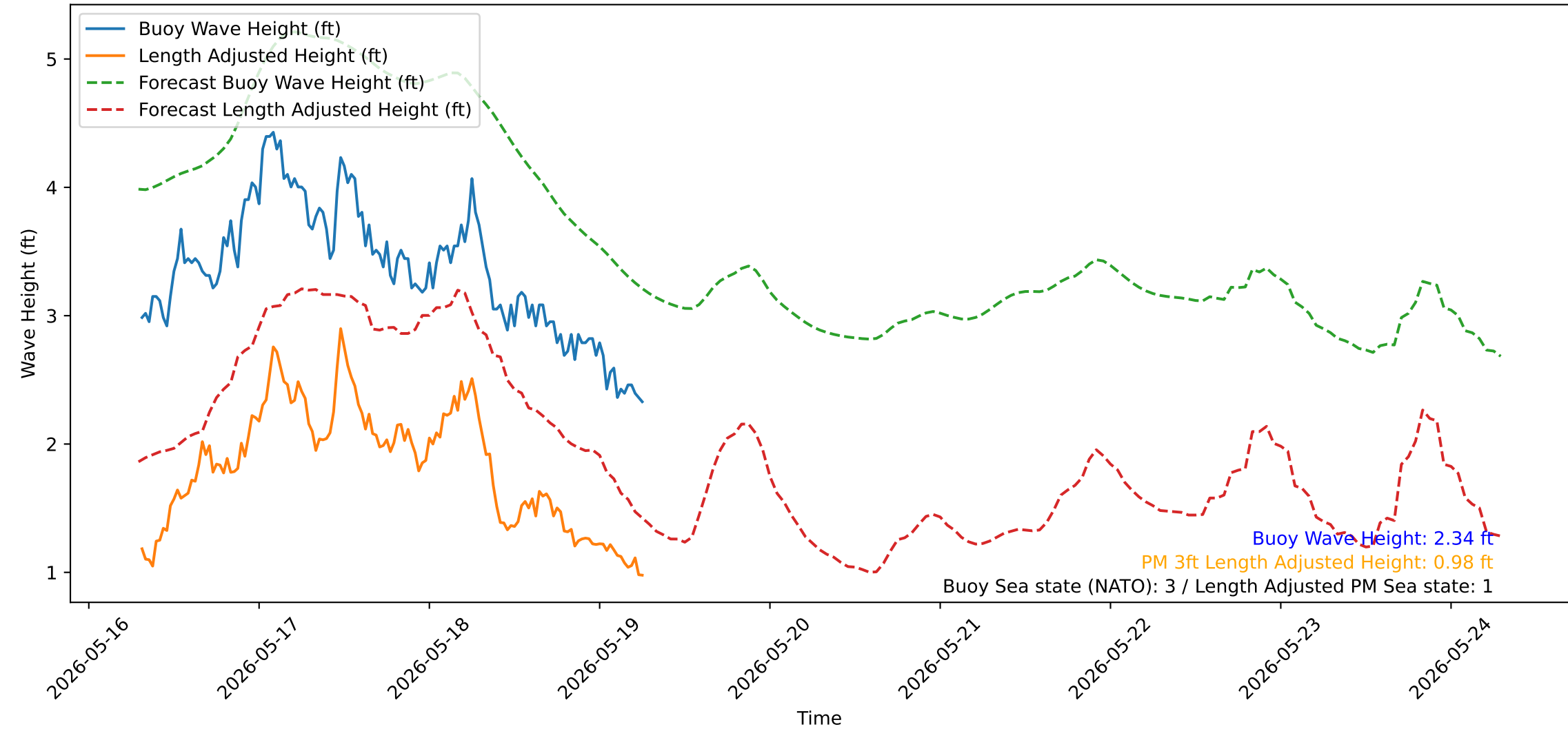
Wave Heights over Time for Green Beach at 2026-05-19 07:21:14
