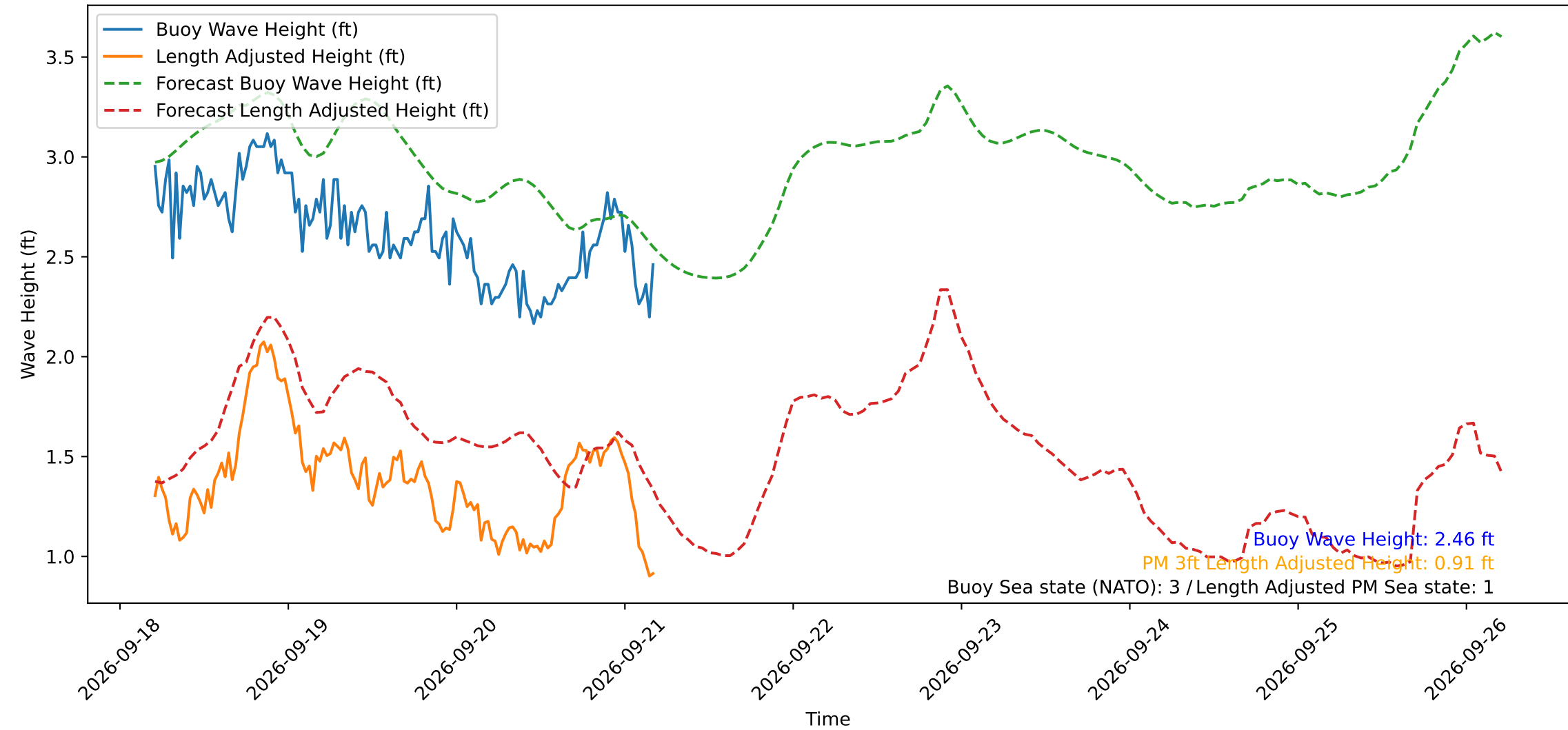
Wave Heights over Time for Green Beach at 2026-09-21 04:51:13
