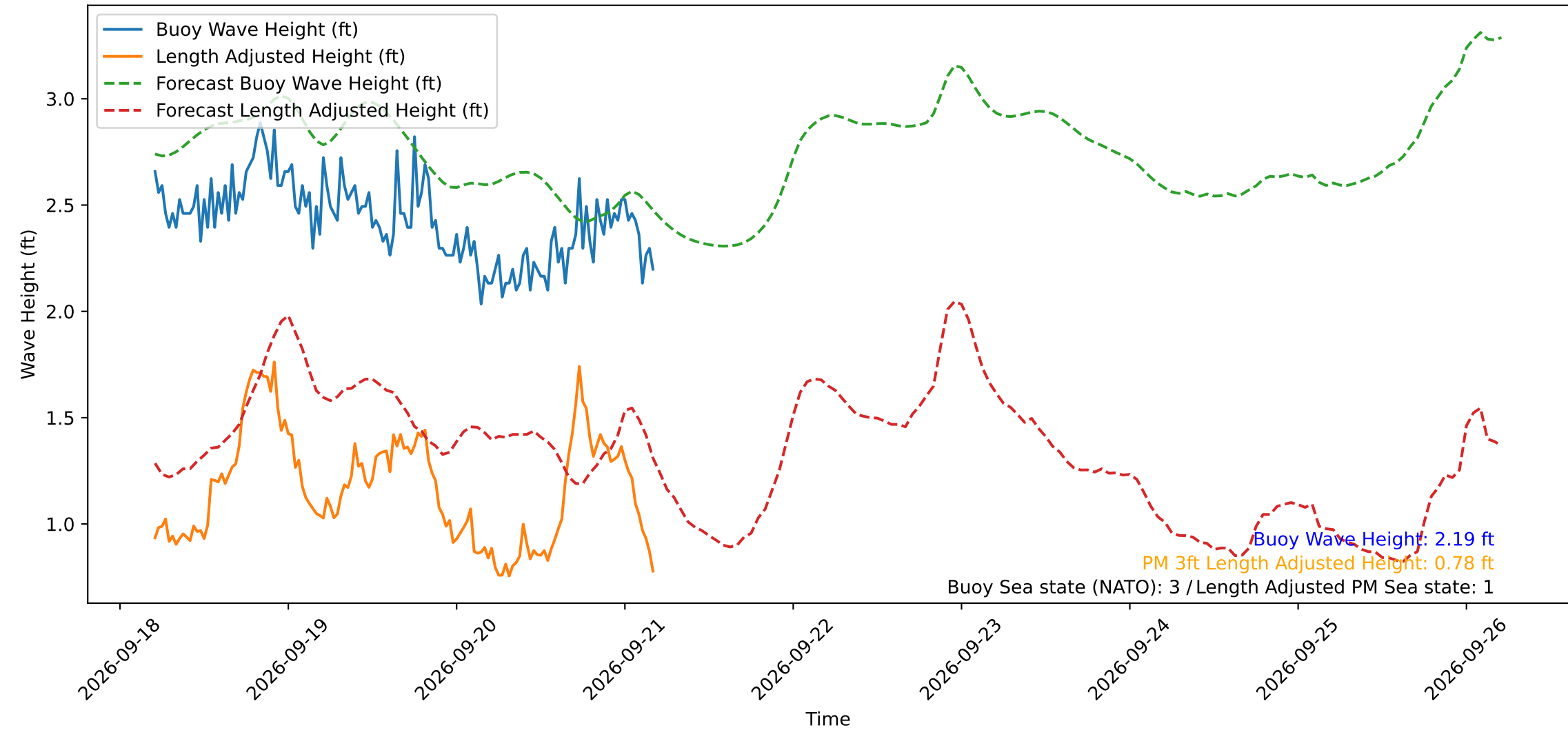
Wave Heights over Time for Red Beach at 2026-09-21 04:50:50
