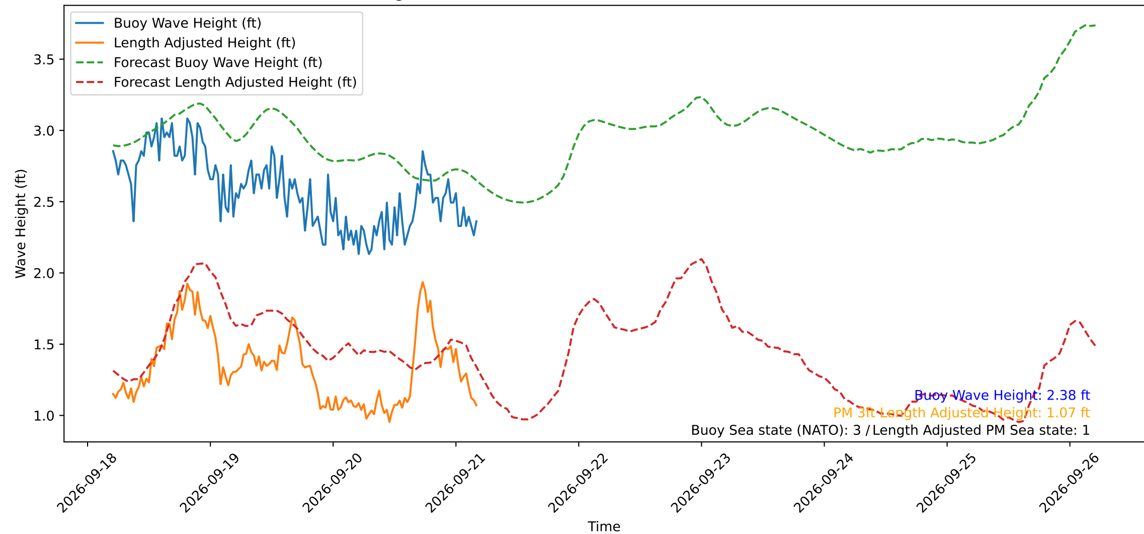
Wave Heights over Time for Oceanside Harbor at 2026-09-21 04:50:29
