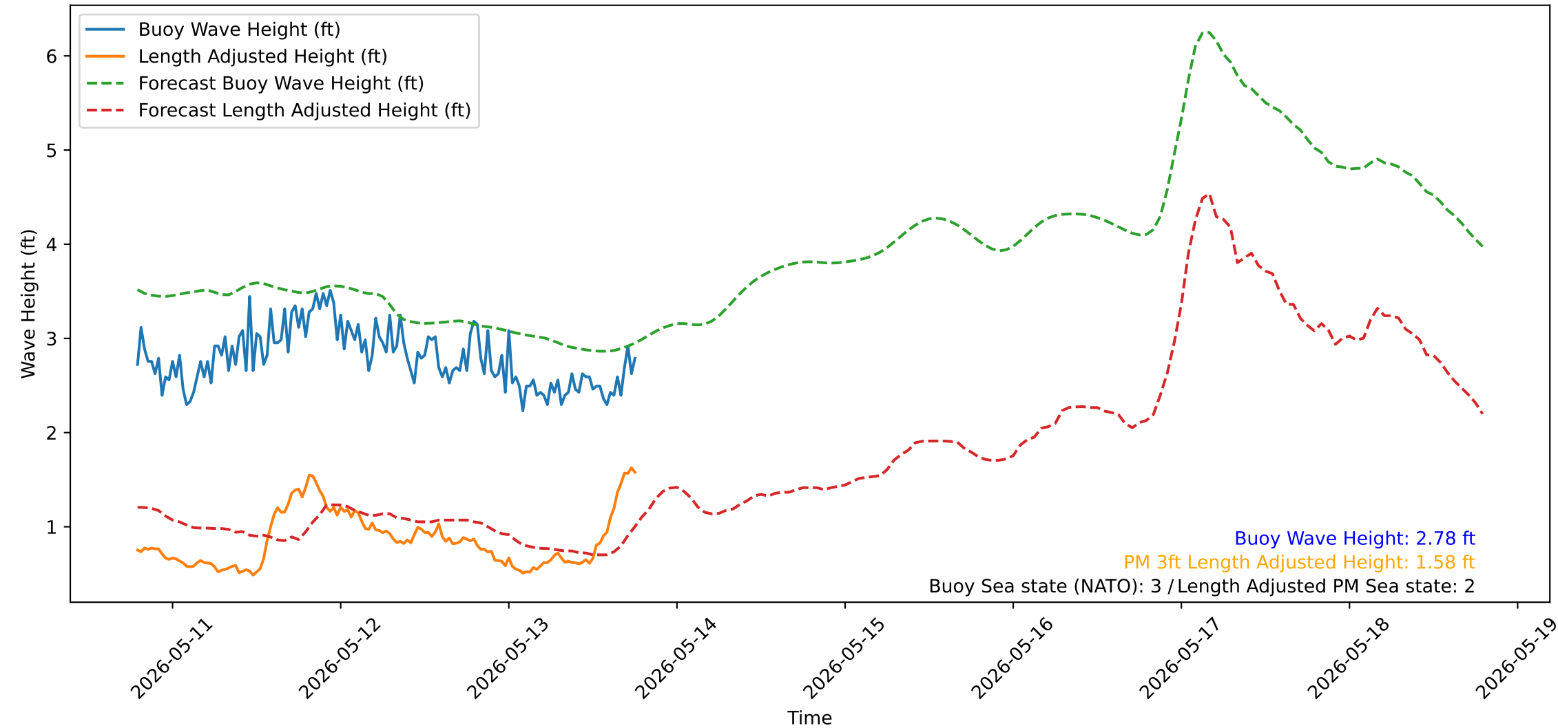
Wave Heights over Time for Green Beach at 2026-05-13 19:01:17
