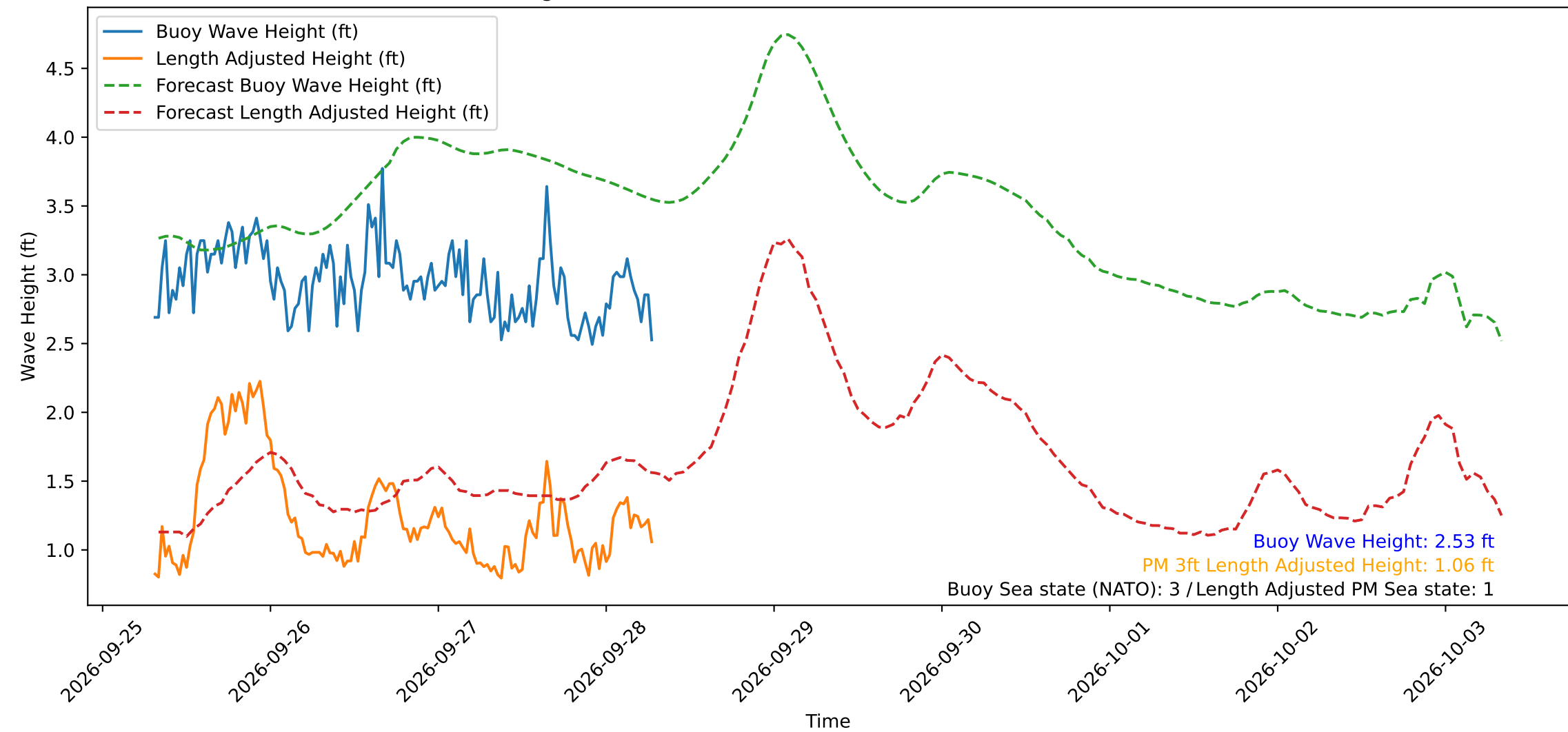
Wave Heights over Time for Oceanside Harbor at 2026-09-28 07:30:30
