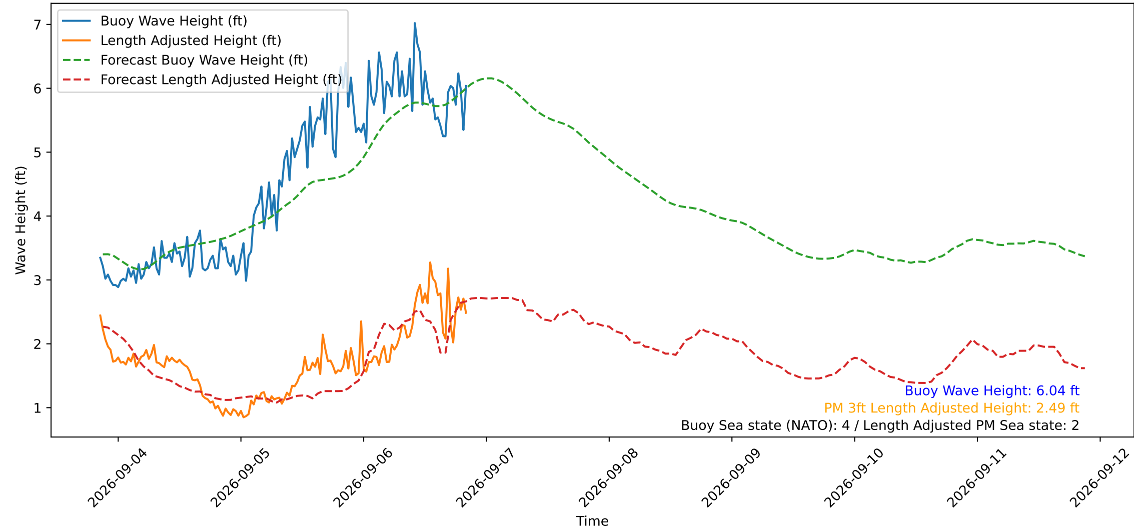
Wave Heights over Time for Oceanside Harbor at 2026-09-06 20:40:30
