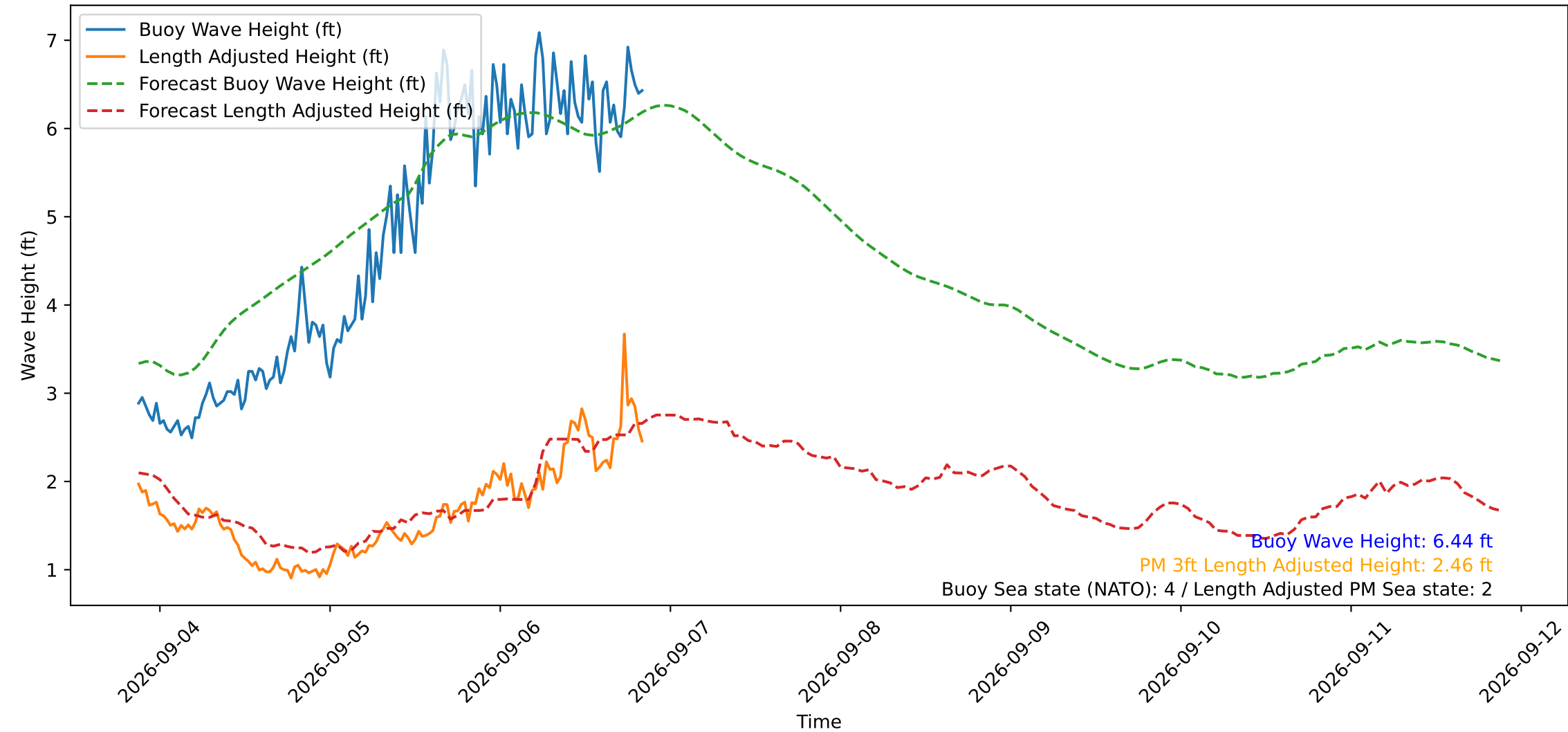
Wave Heights over Time for Green Beach at 2026-09-06 20:41:12
