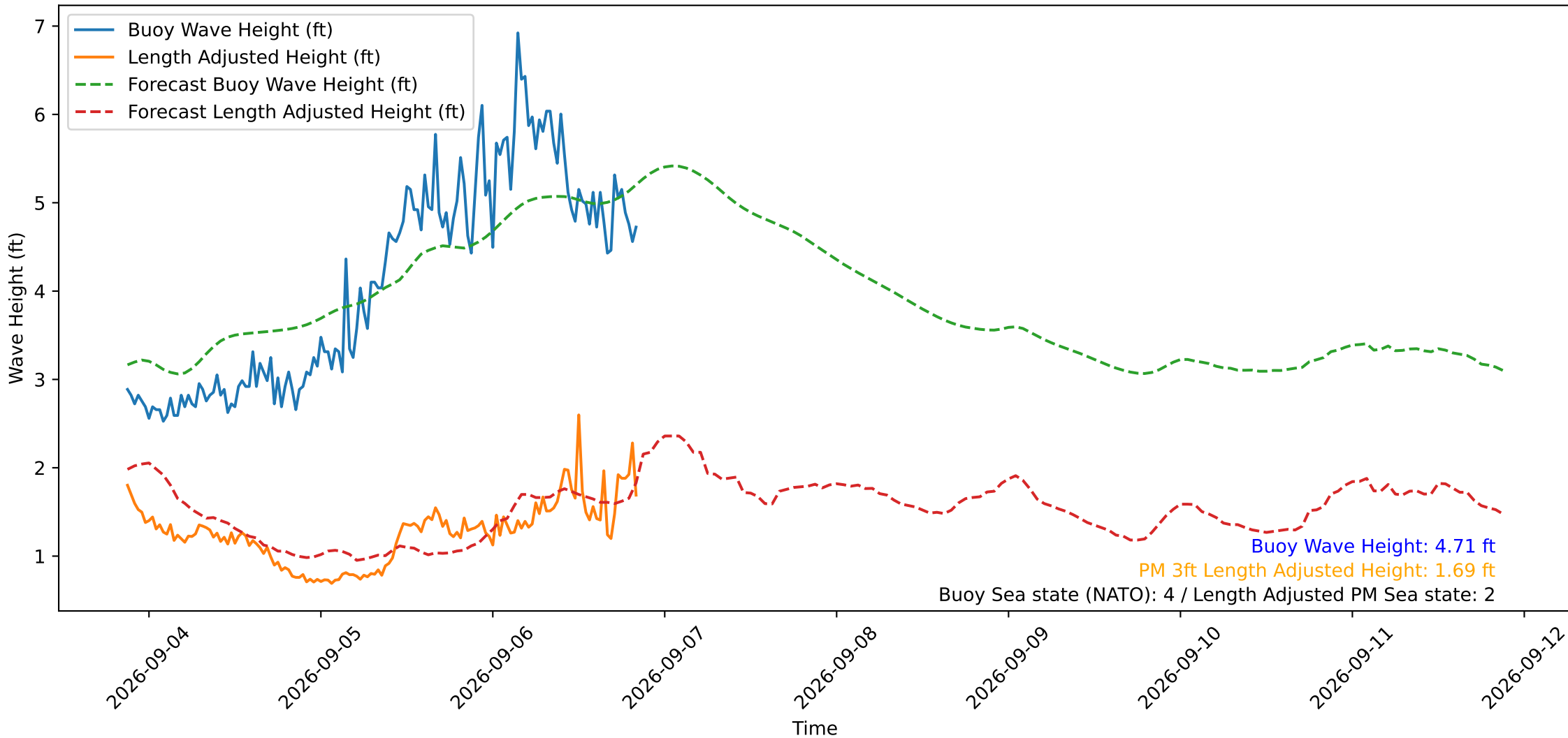
Wave Heights over Time for Red Beach at 2026-09-06 20:40:50
