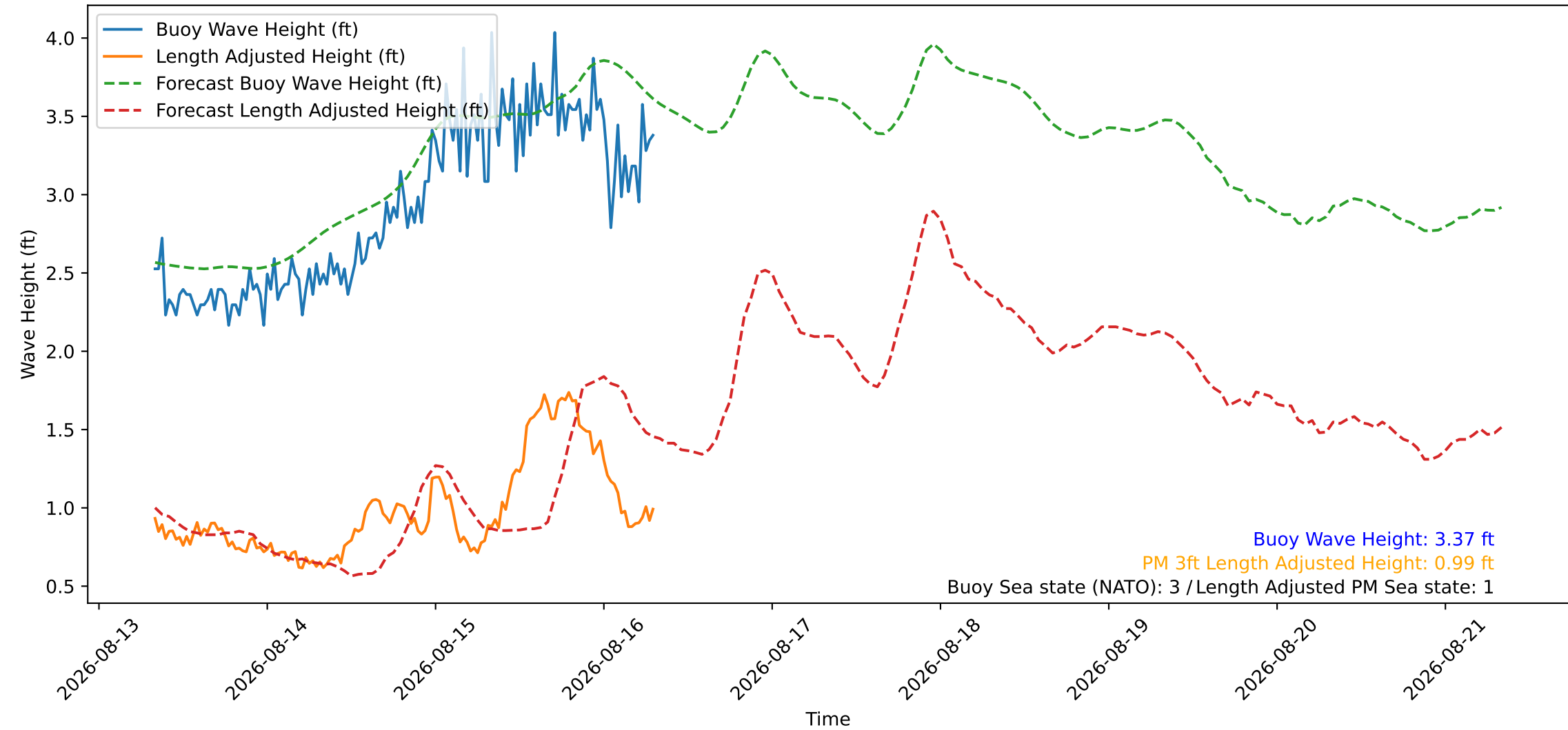
Wave Heights over Time for Red Beach at 2026-08-16 07:40:46
