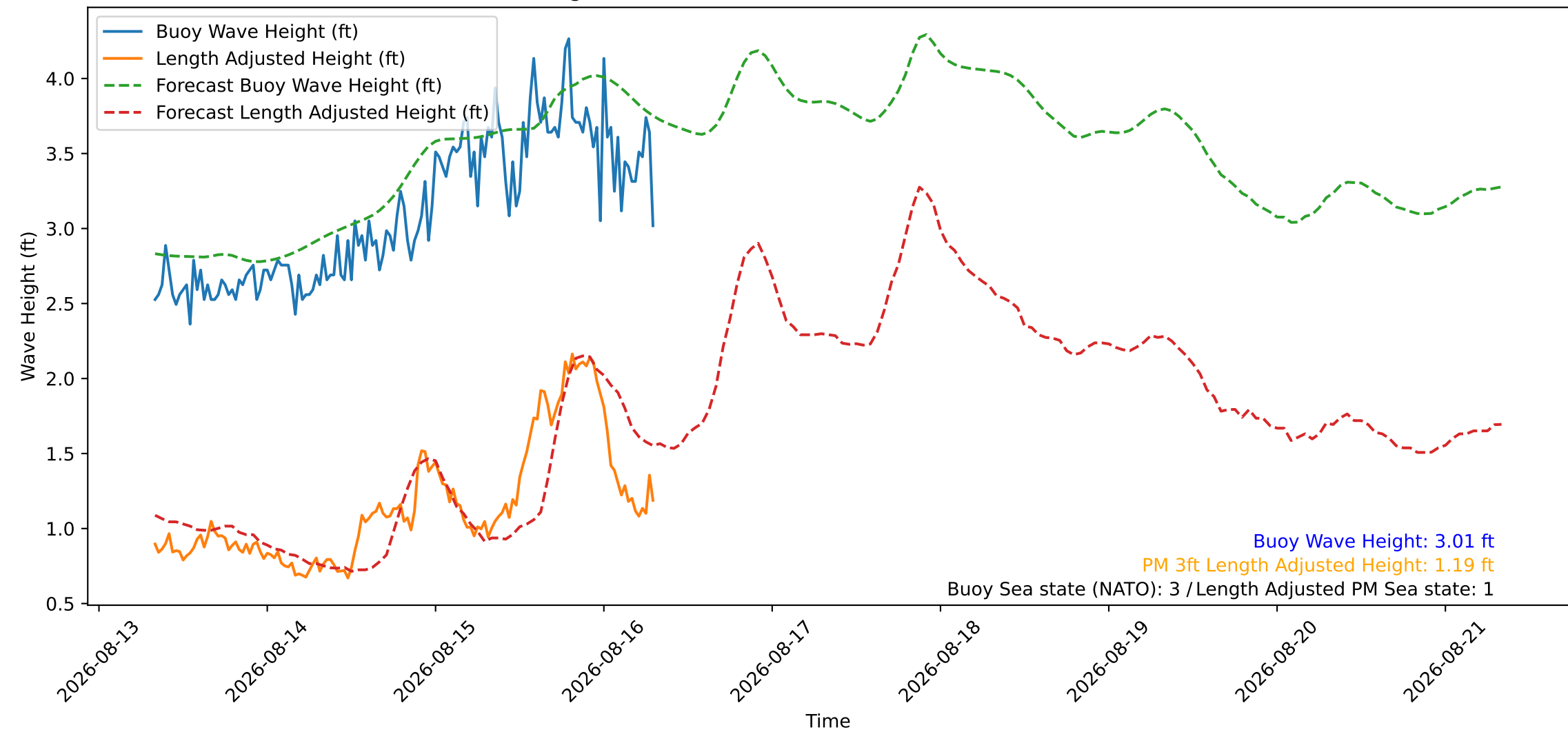
Wave Heights over Time for Green Beach at 2026-08-16 07:41:09
