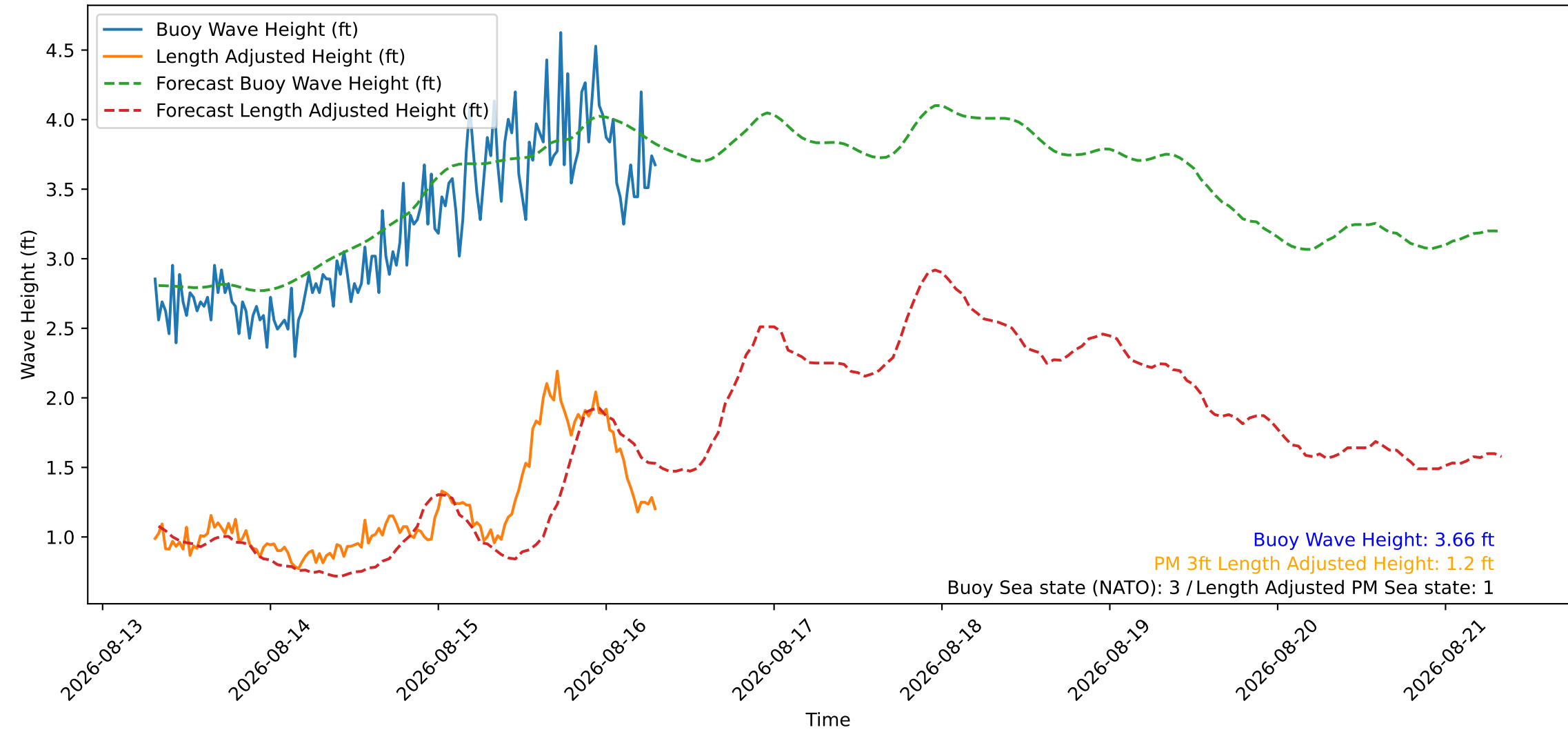
Wave Heights over Time for Oceanside Harbor at 2026-08-16 07:40:27
