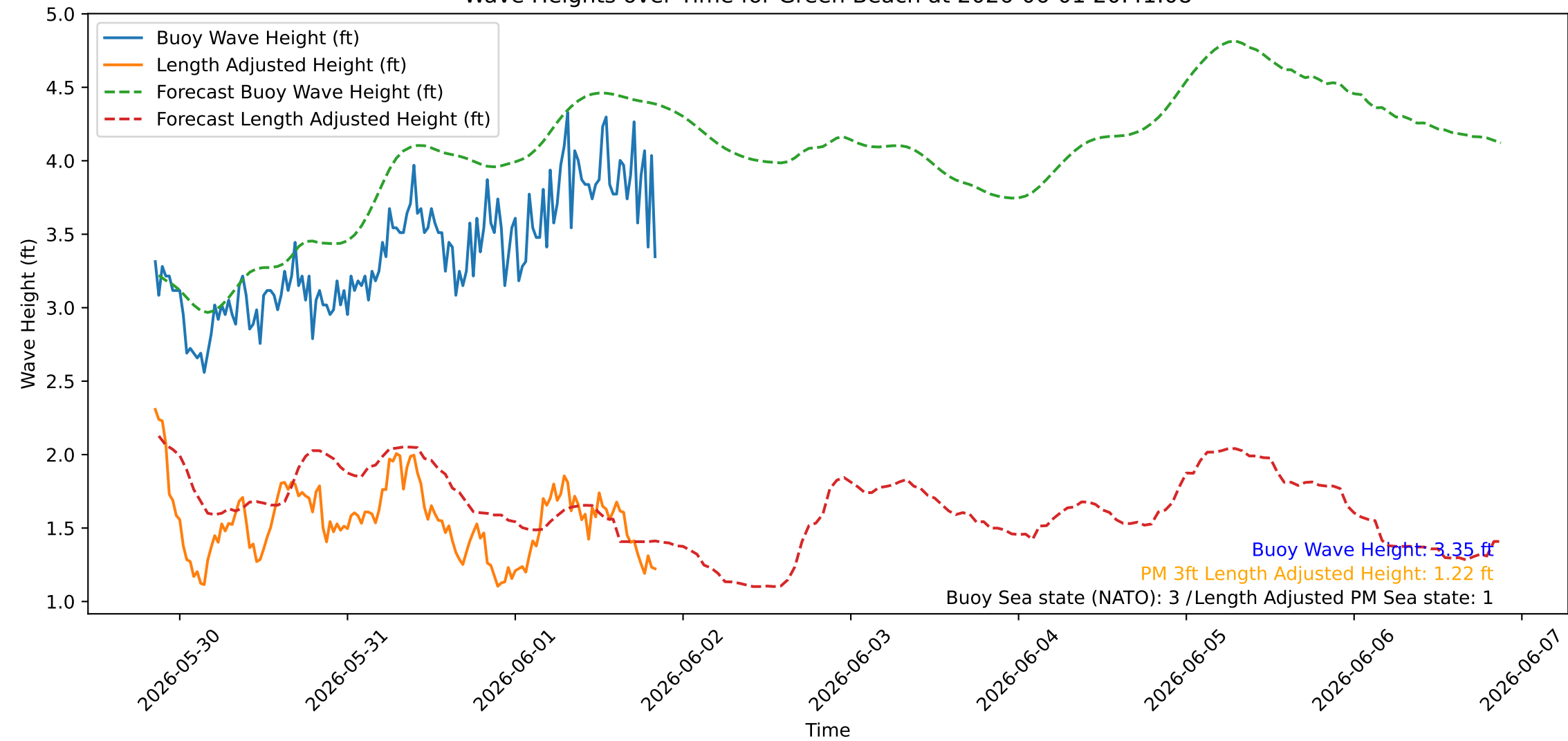
Wave Heights over Time for Green Beach at 2026-06-01 20:41:08
