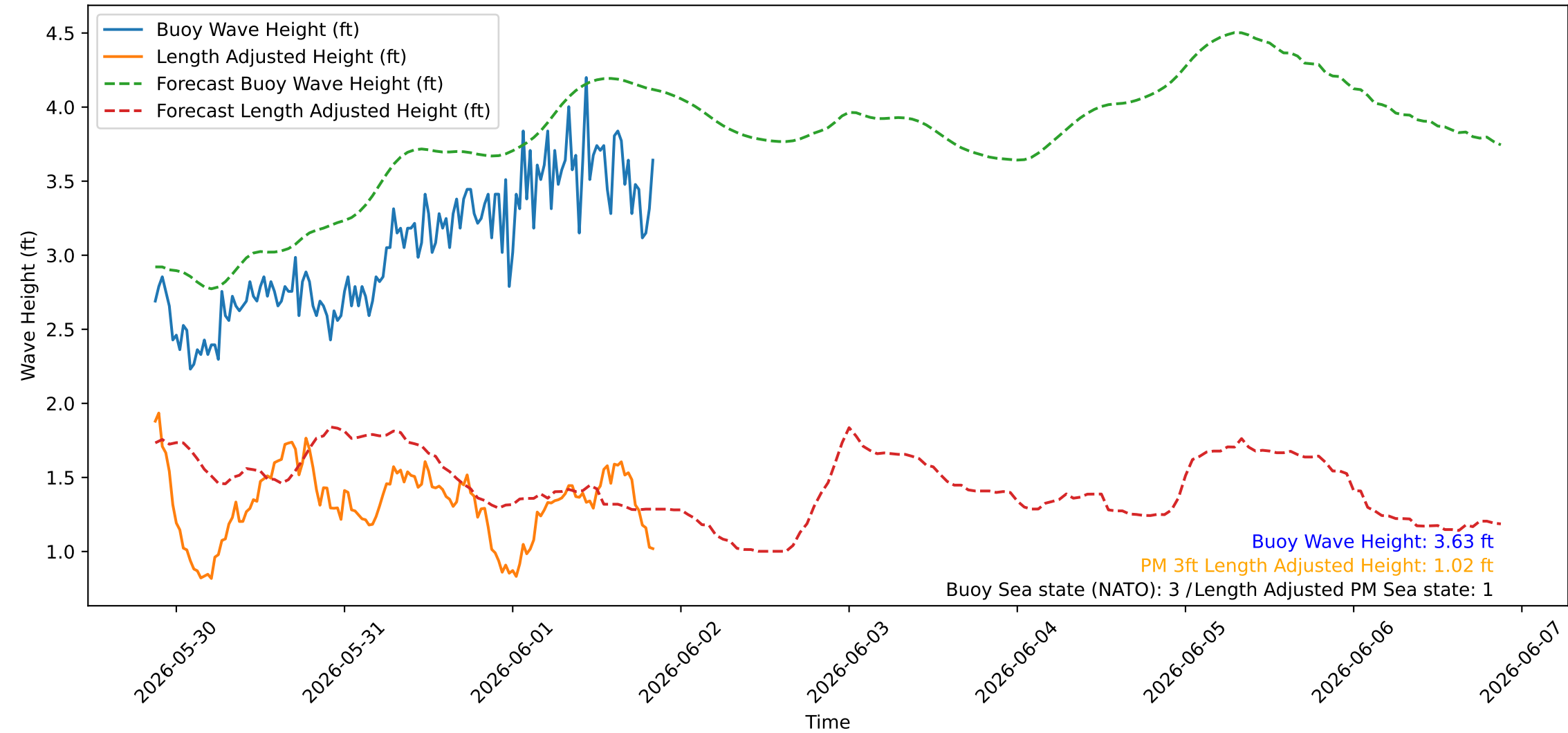
Wave Heights over Time for Red Beach at 2026-06-01 20:40:45
