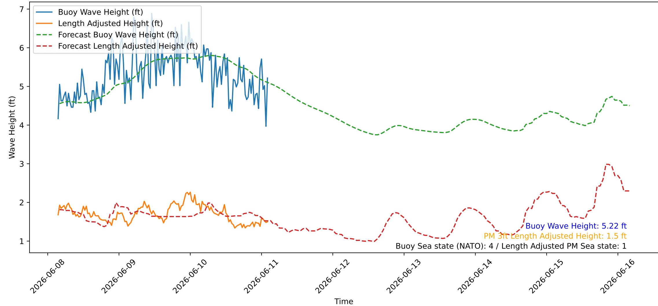
Wave Heights over Time for Green Beach at 2026-06-11 03:31:10
