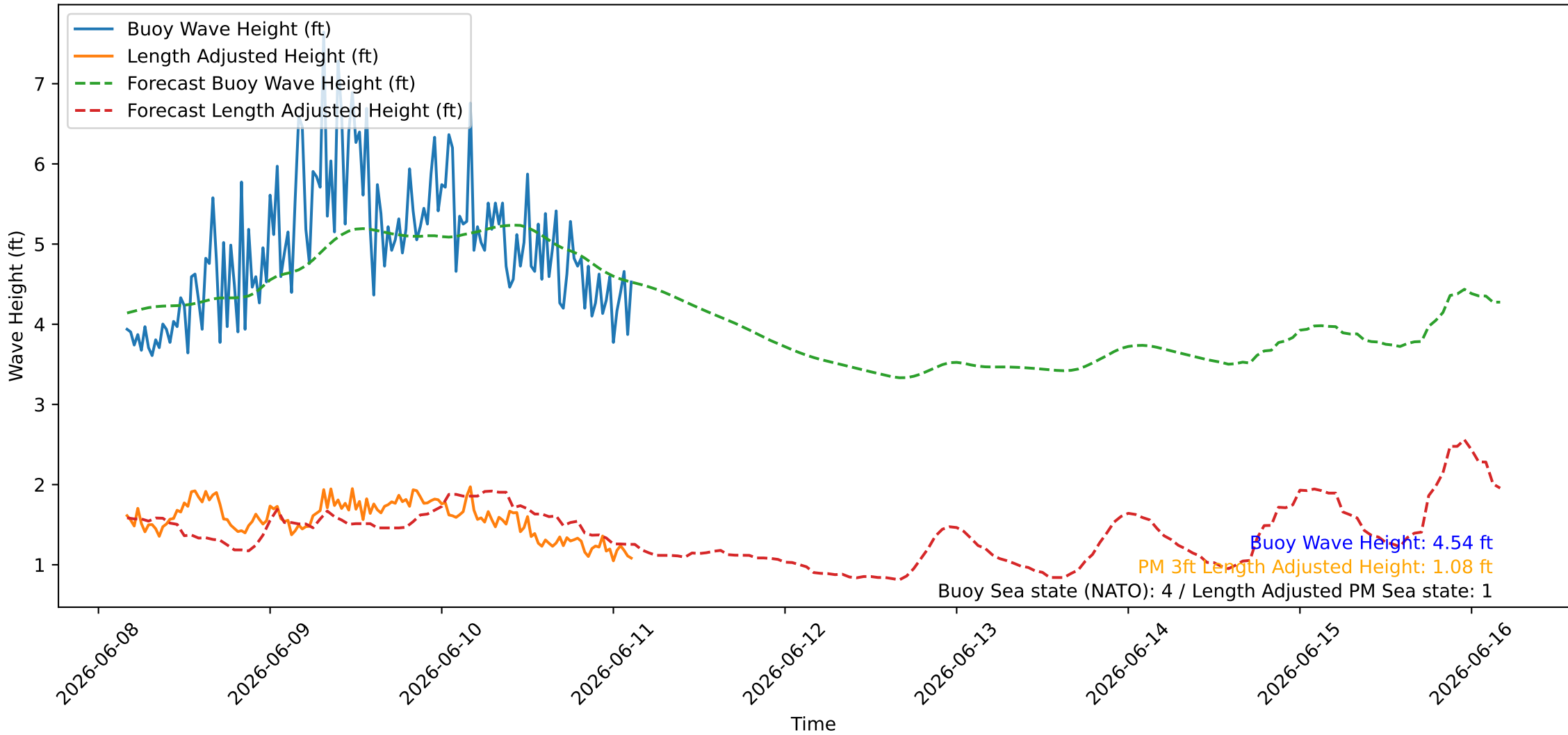
Wave Heights over Time for Red Beach at 2026-06-11 03:30:47
