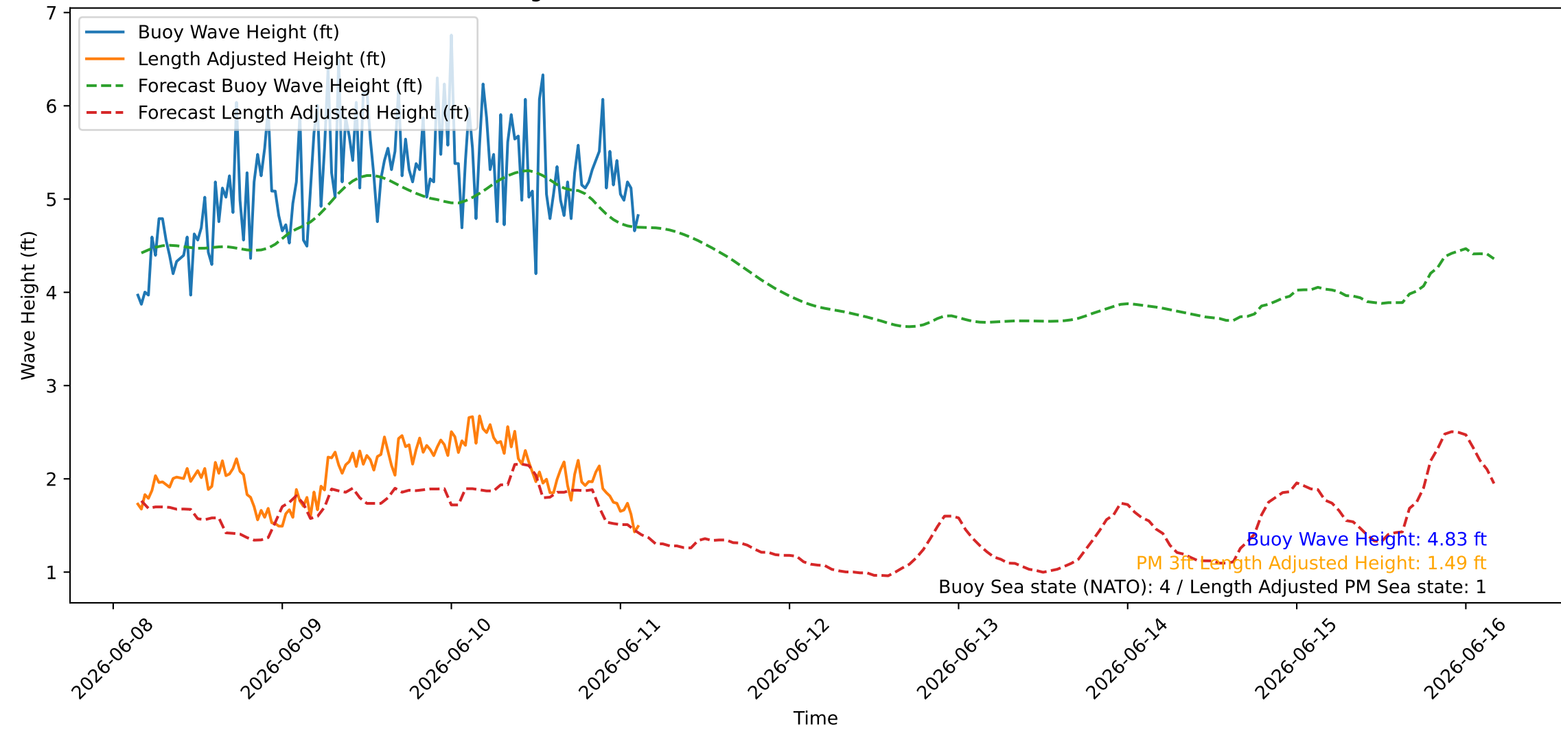
Wave Heights over Time for Oceanside Harbor at 2026-06-11 03:30:26
