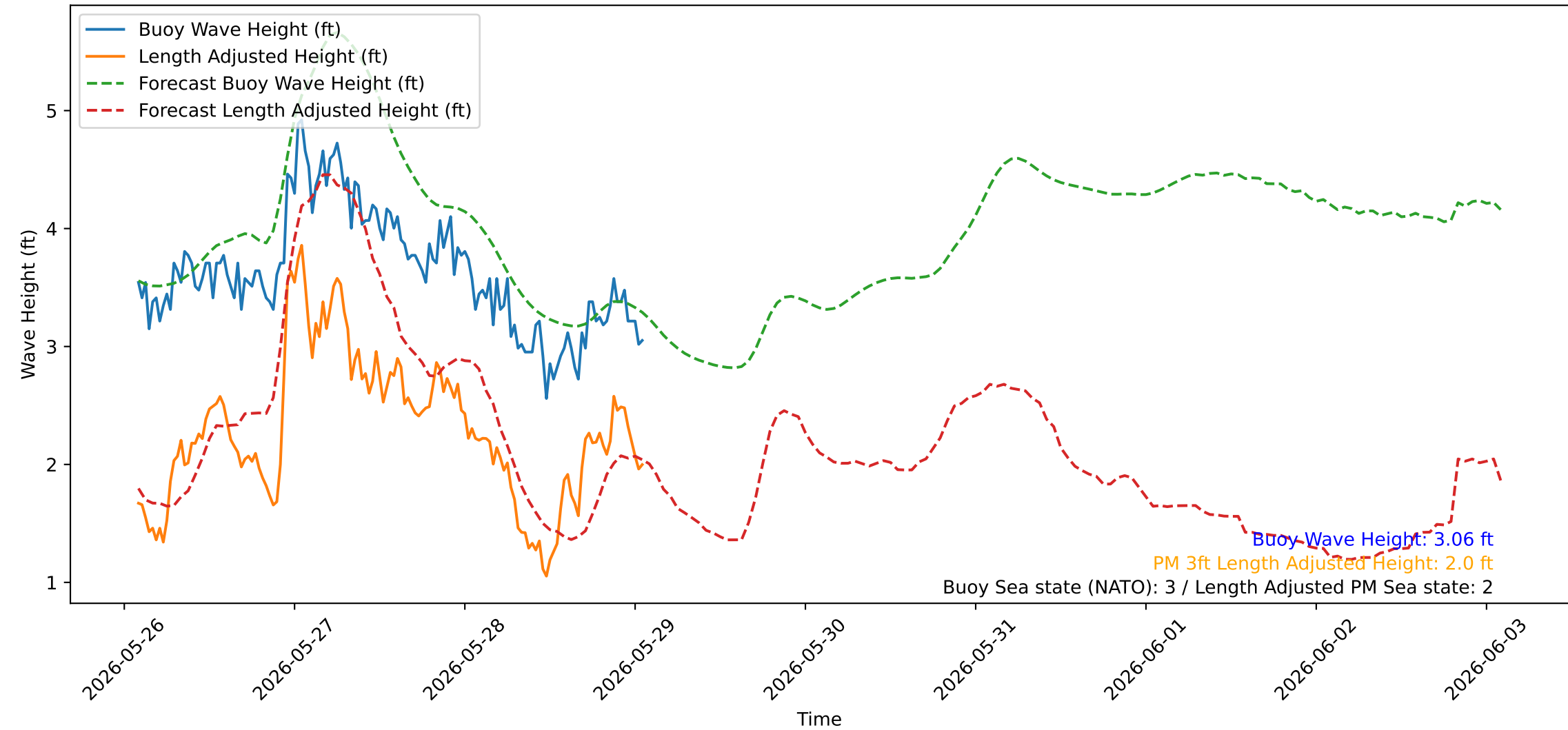
Wave Heights over Time for Green Beach at 2026-05-29 01:51:45
