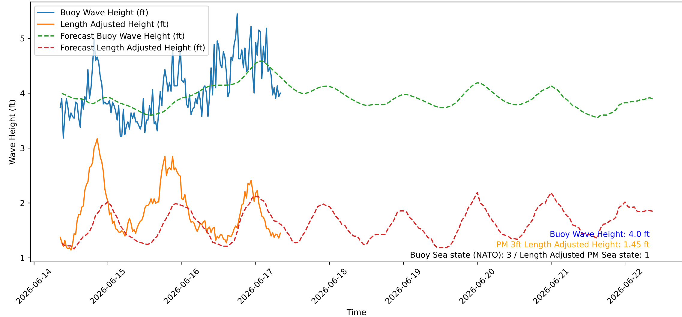
Wave Heights over Time for Oceanside Harbor at 2026-06-17 08:40:27
