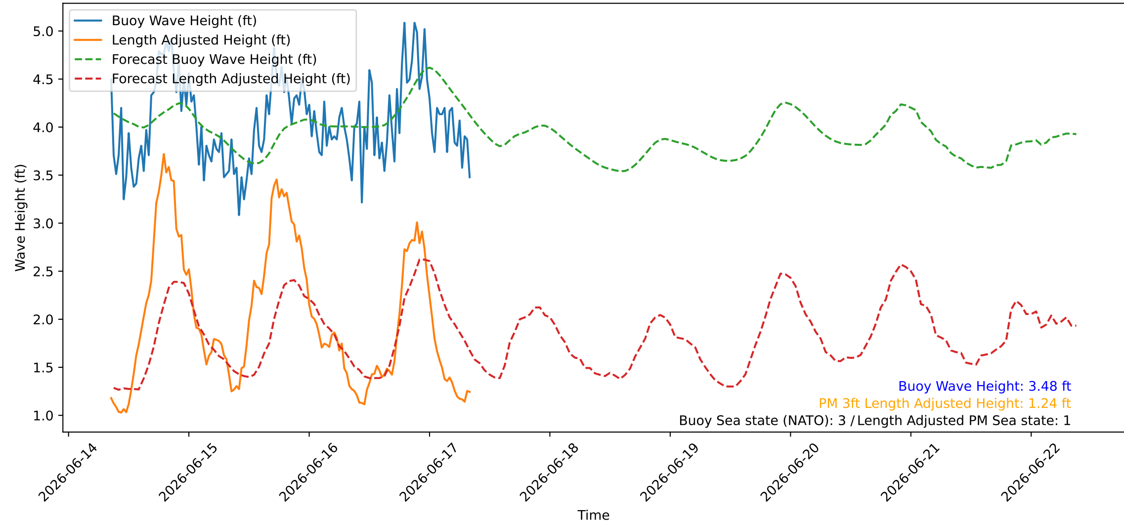
Wave Heights over Time for Green Beach at 2026-06-17 08:41:09
