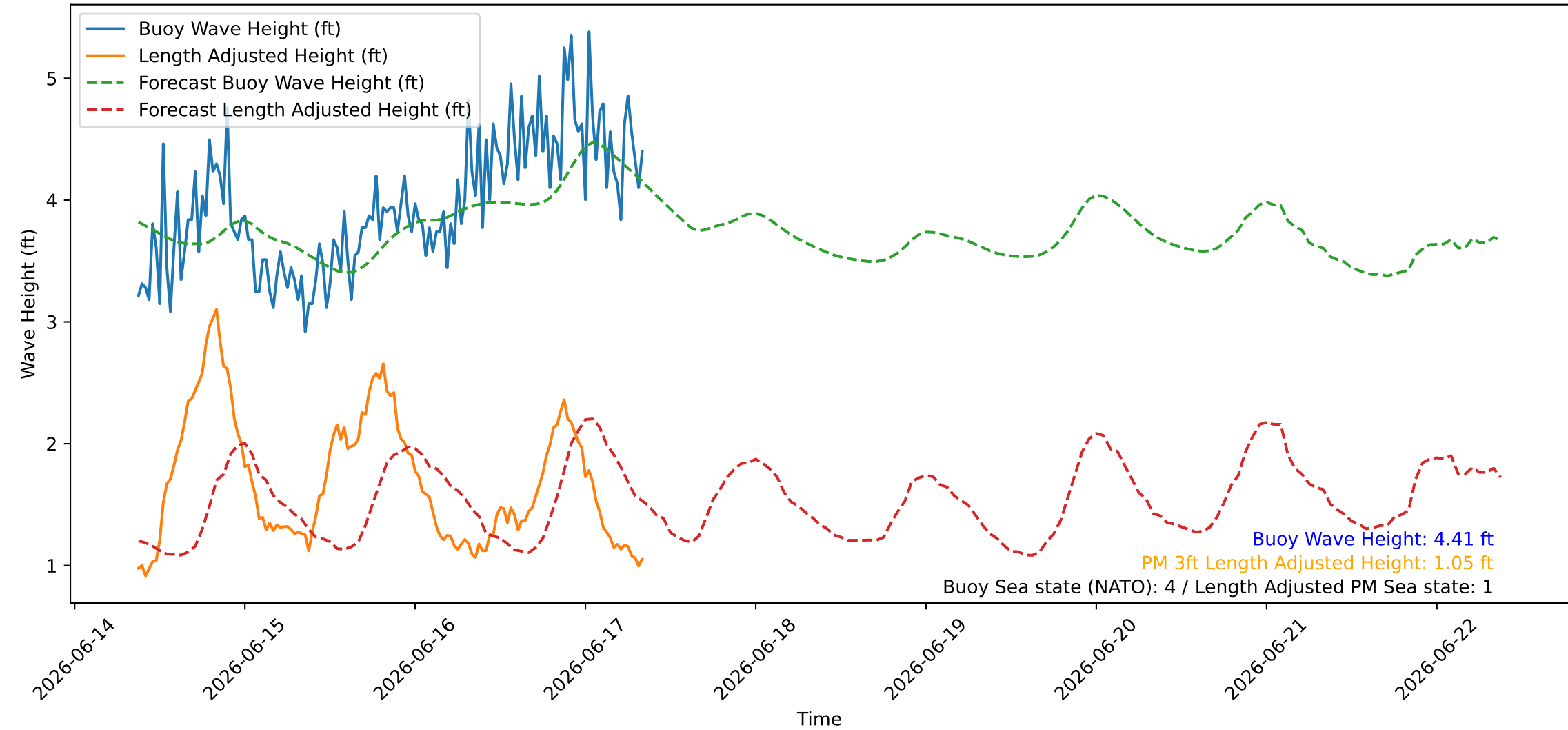
Wave Heights over Time for Red Beach at 2026-06-17 08:40:46
