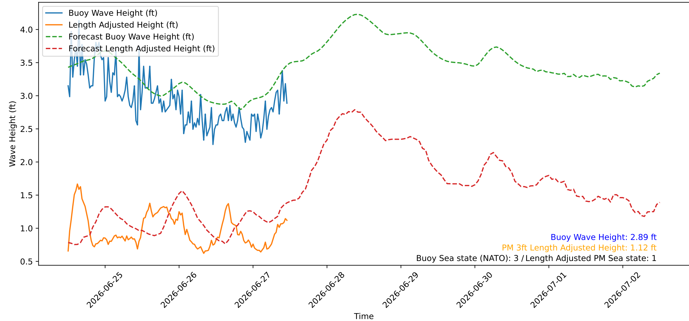
Wave Heights over Time for Red Beach at 2026-06-27 11:50:47
