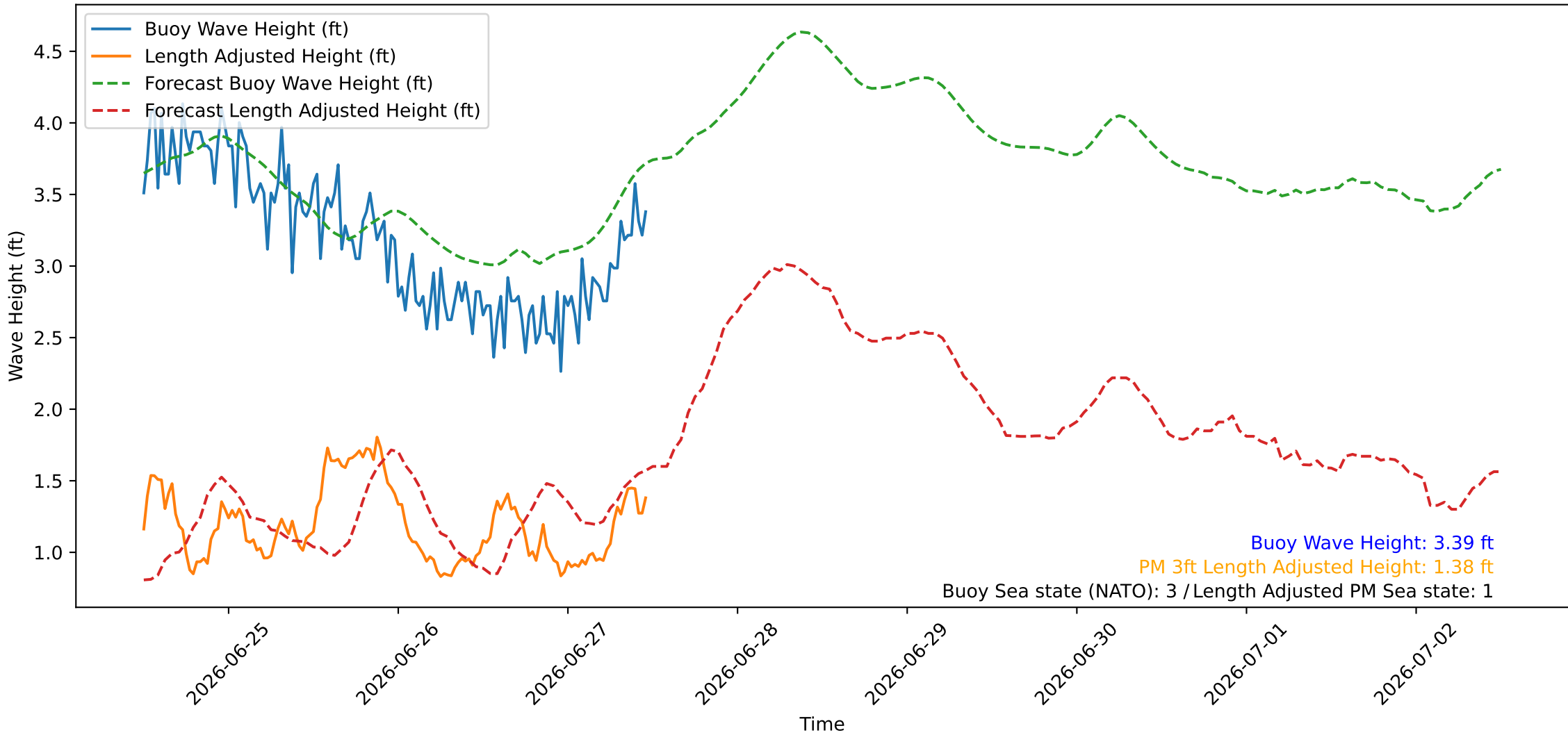
Wave Heights over Time for Green Beach at 2026-06-27 11:51:09
