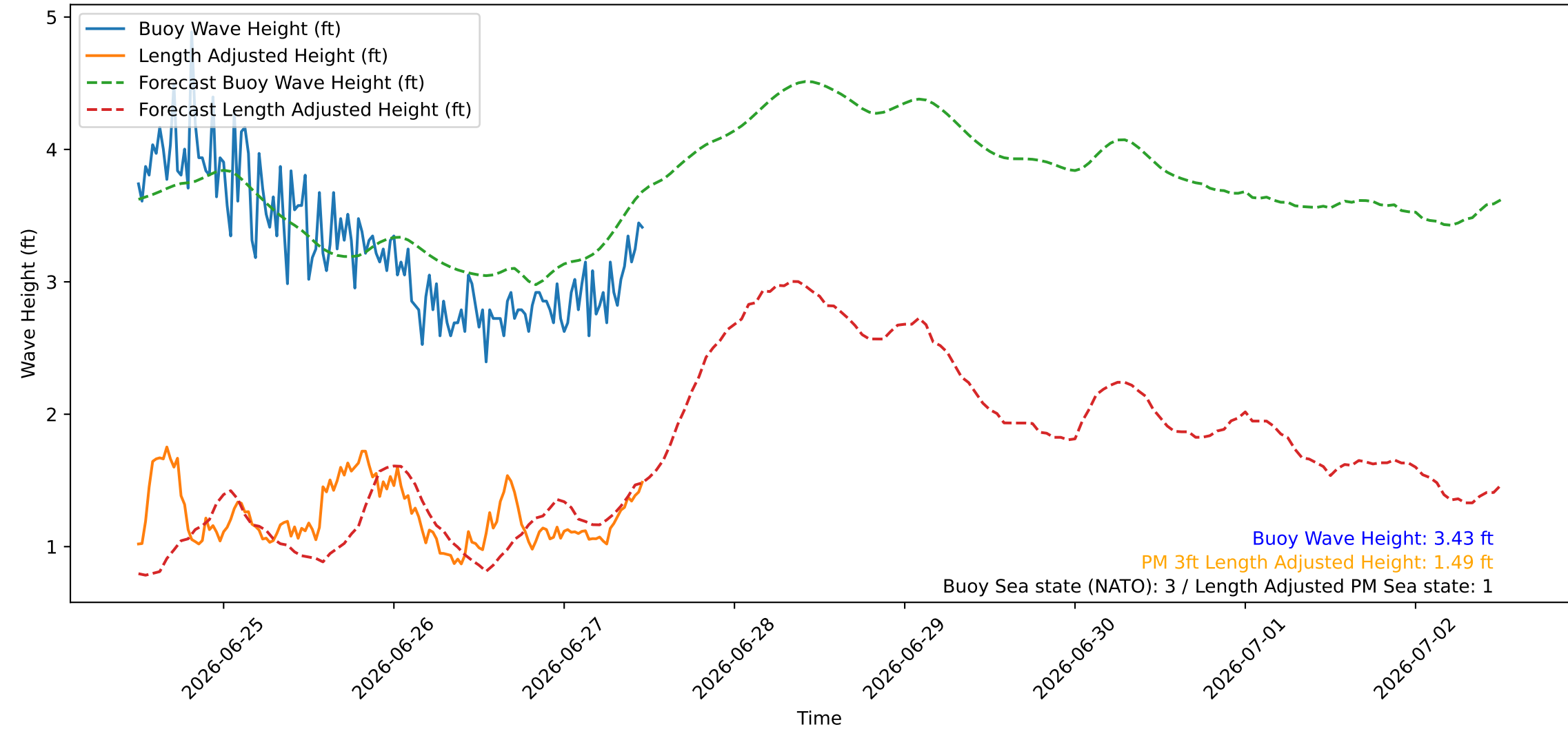
Wave Heights over Time for Oceanside Harbor at 2026-06-27 11:50:26
