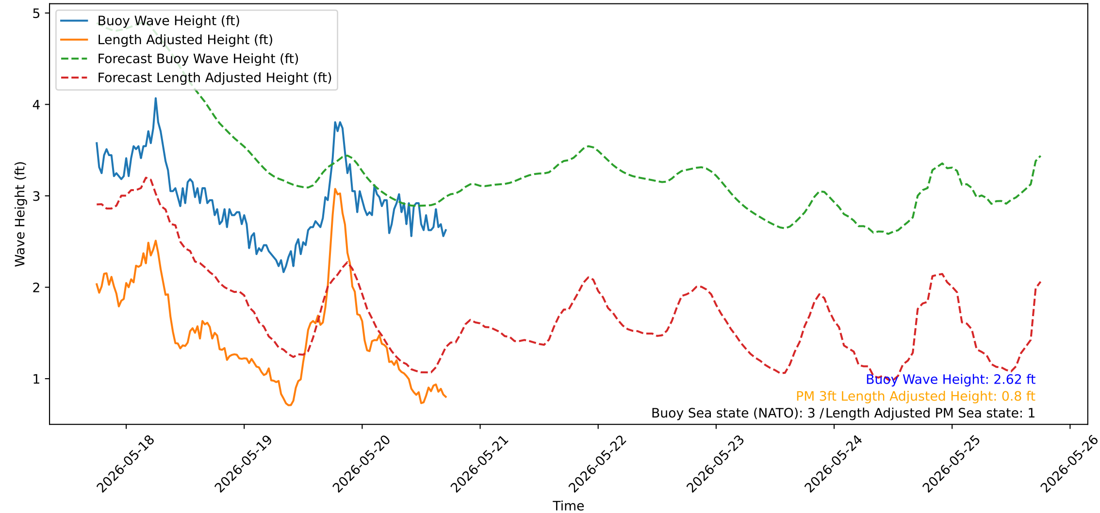
Wave Heights over Time for Green Beach at 2026-05-20 18:01:14
