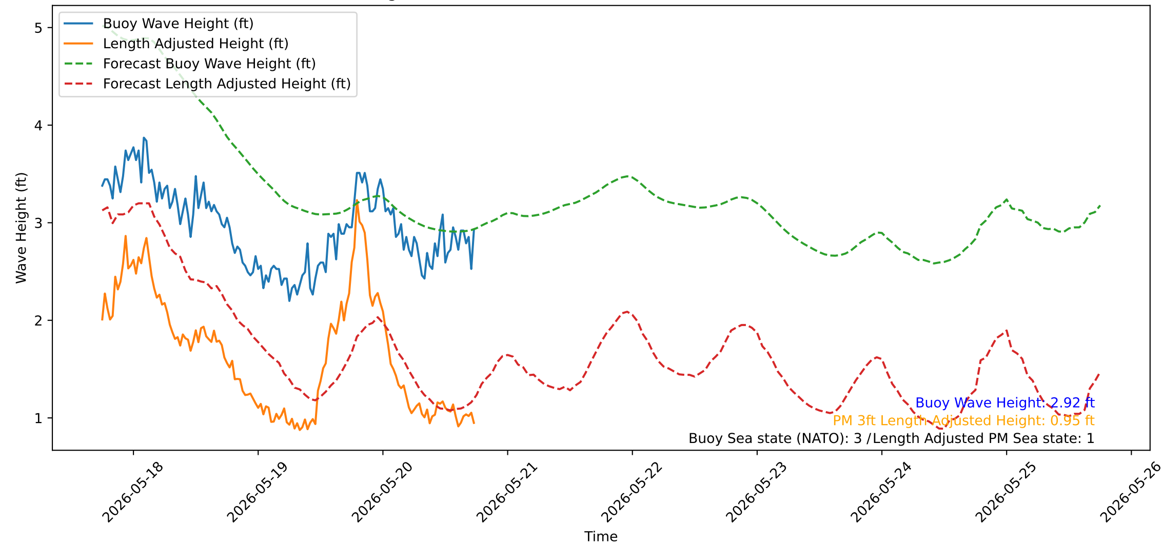
Wave Heights over Time for Oceanside Harbor at 2026-05-20 18:00:31
