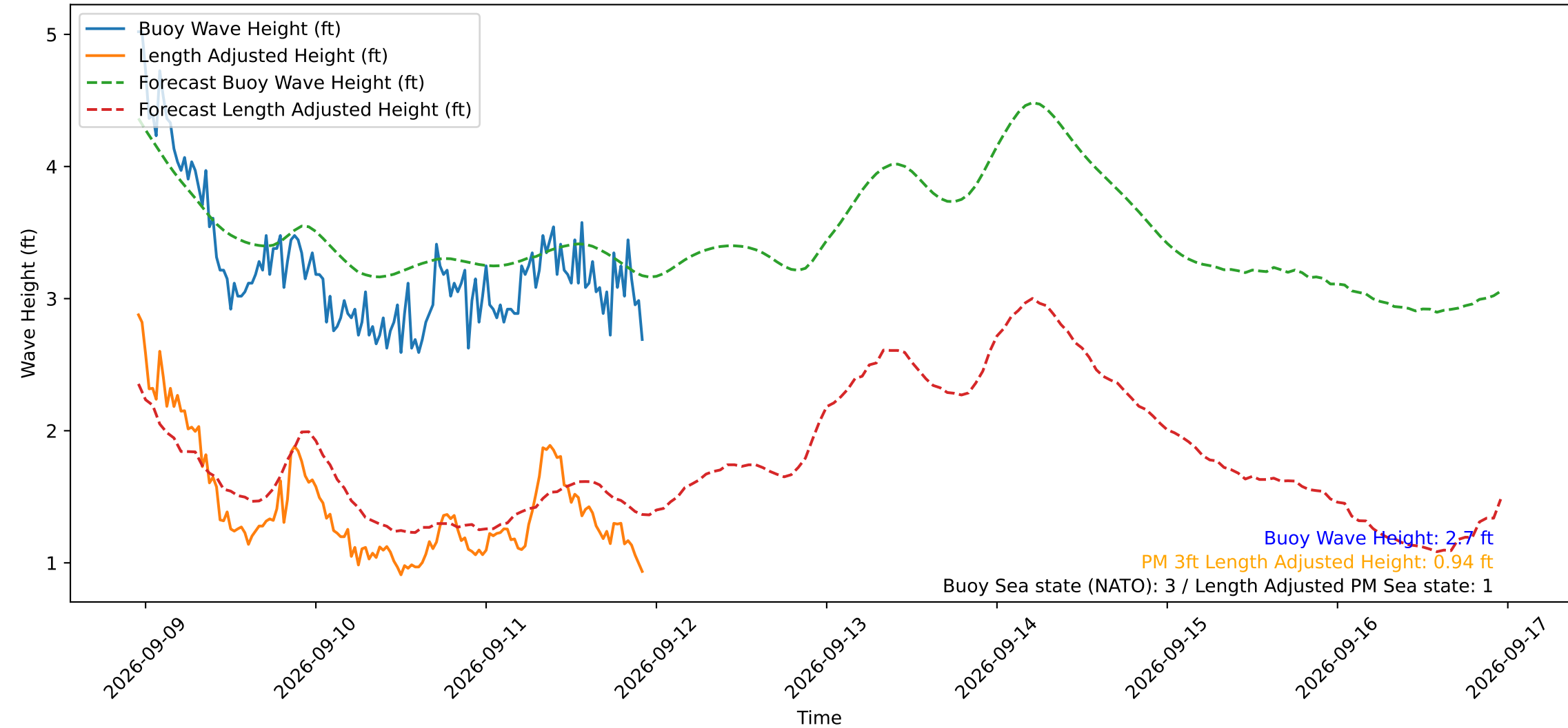
Wave Heights over Time for Green Beach at 2026-09-11 22:41:12
