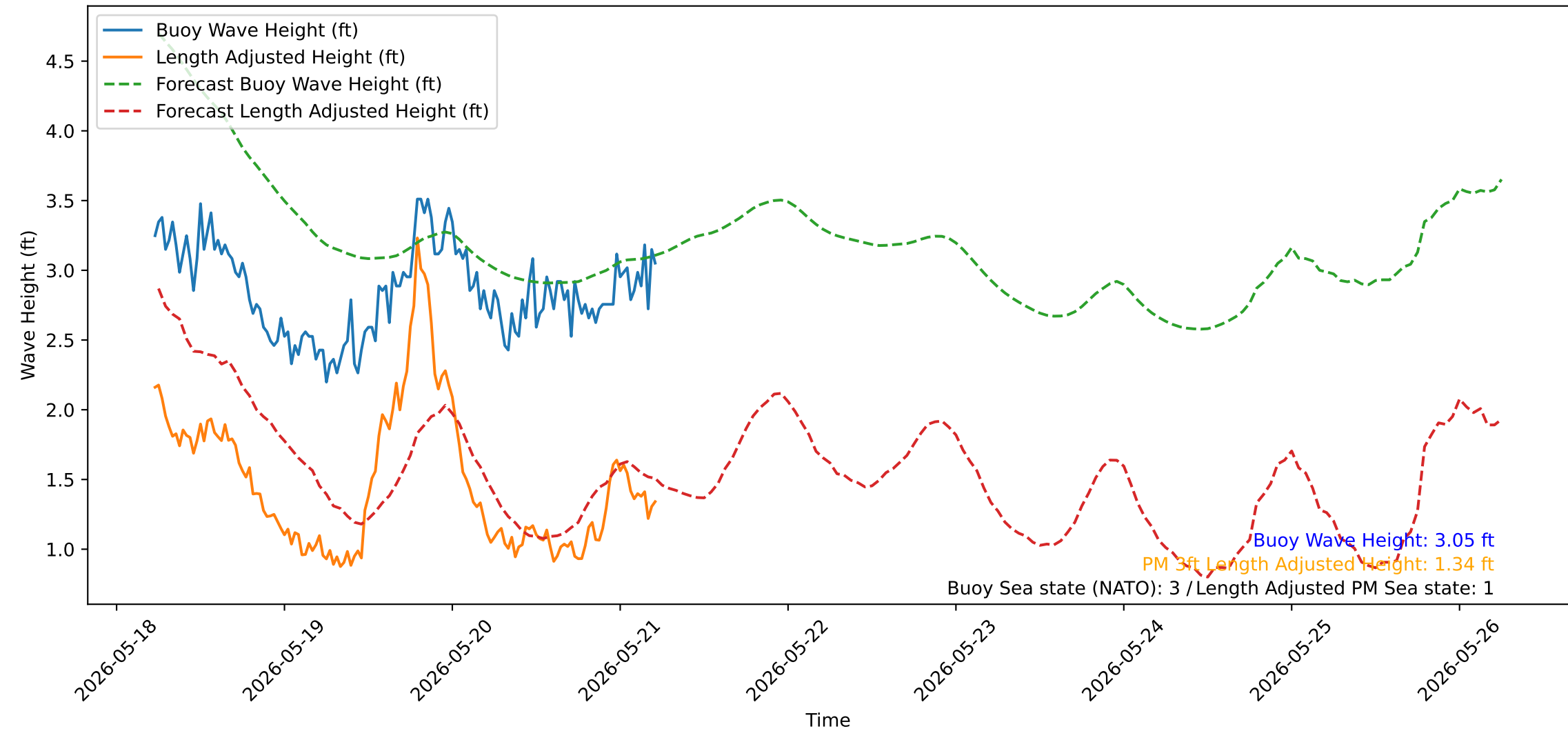
Wave Heights over Time for Oceanside Harbor at 2026-05-21 05:30:31
