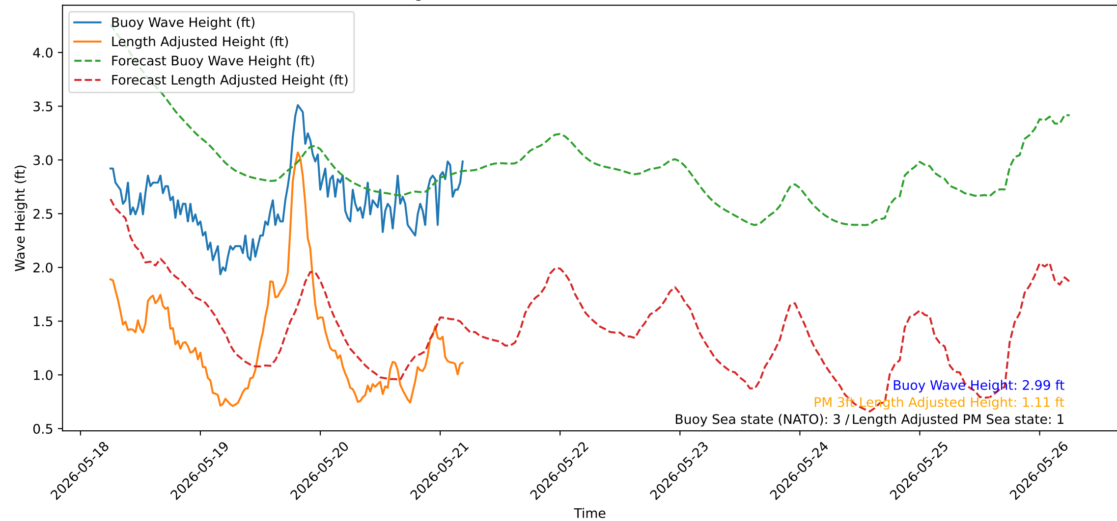
Wave Heights over Time for Red Beach at 2026-05-21 05:30:51
