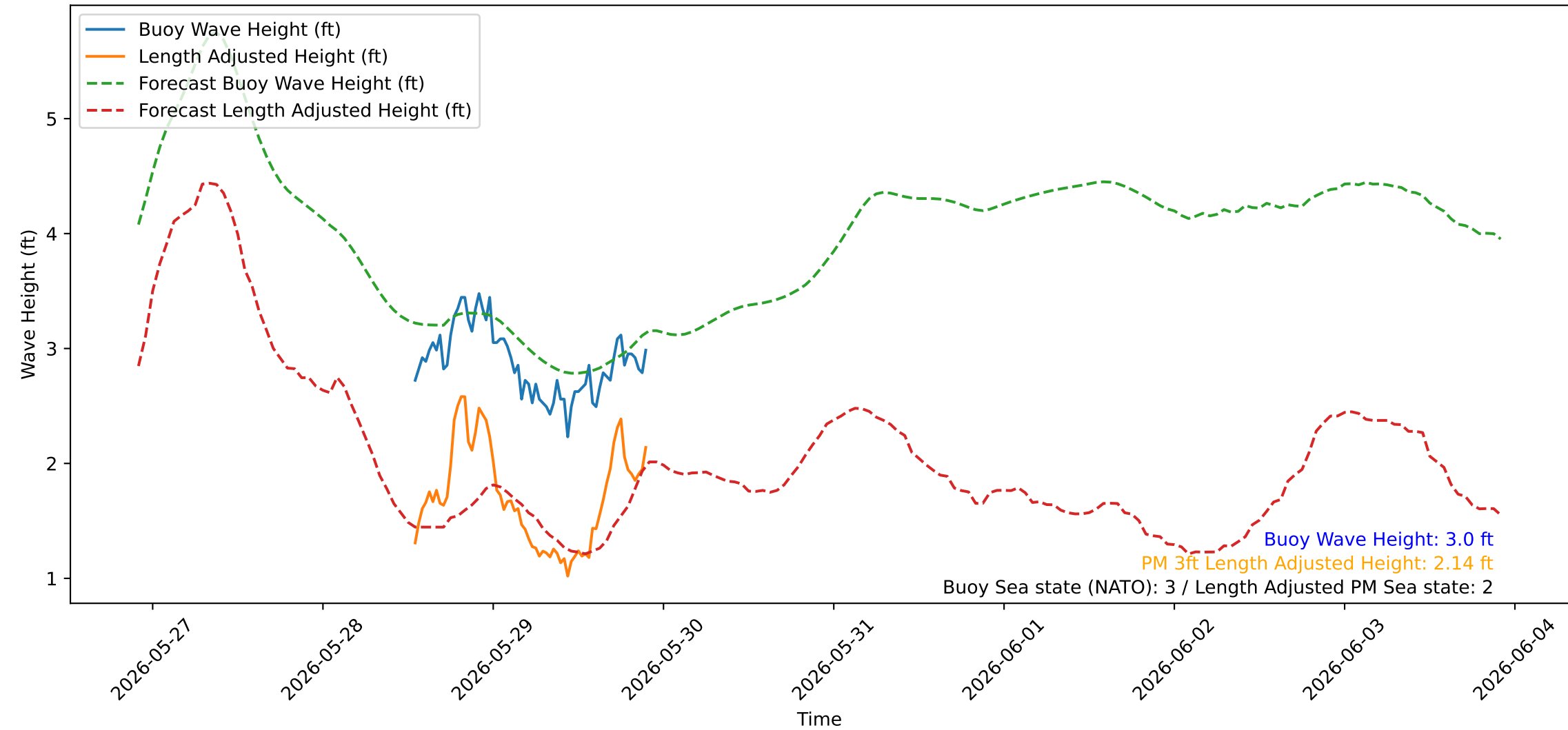
Wave Heights over Time for Oceanside Harbor at 2026-05-29 22:00:22
