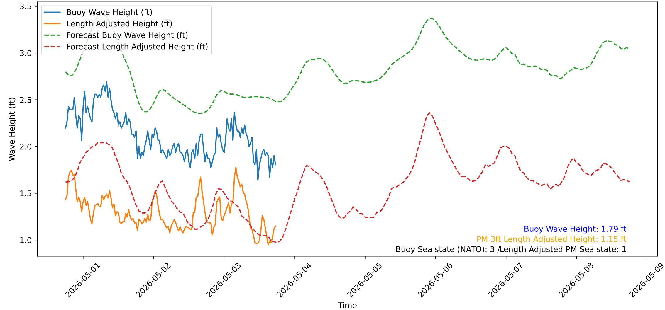
Wave Heights over Time for Oceanside Harbor at 2026-05-03 18:10:31
