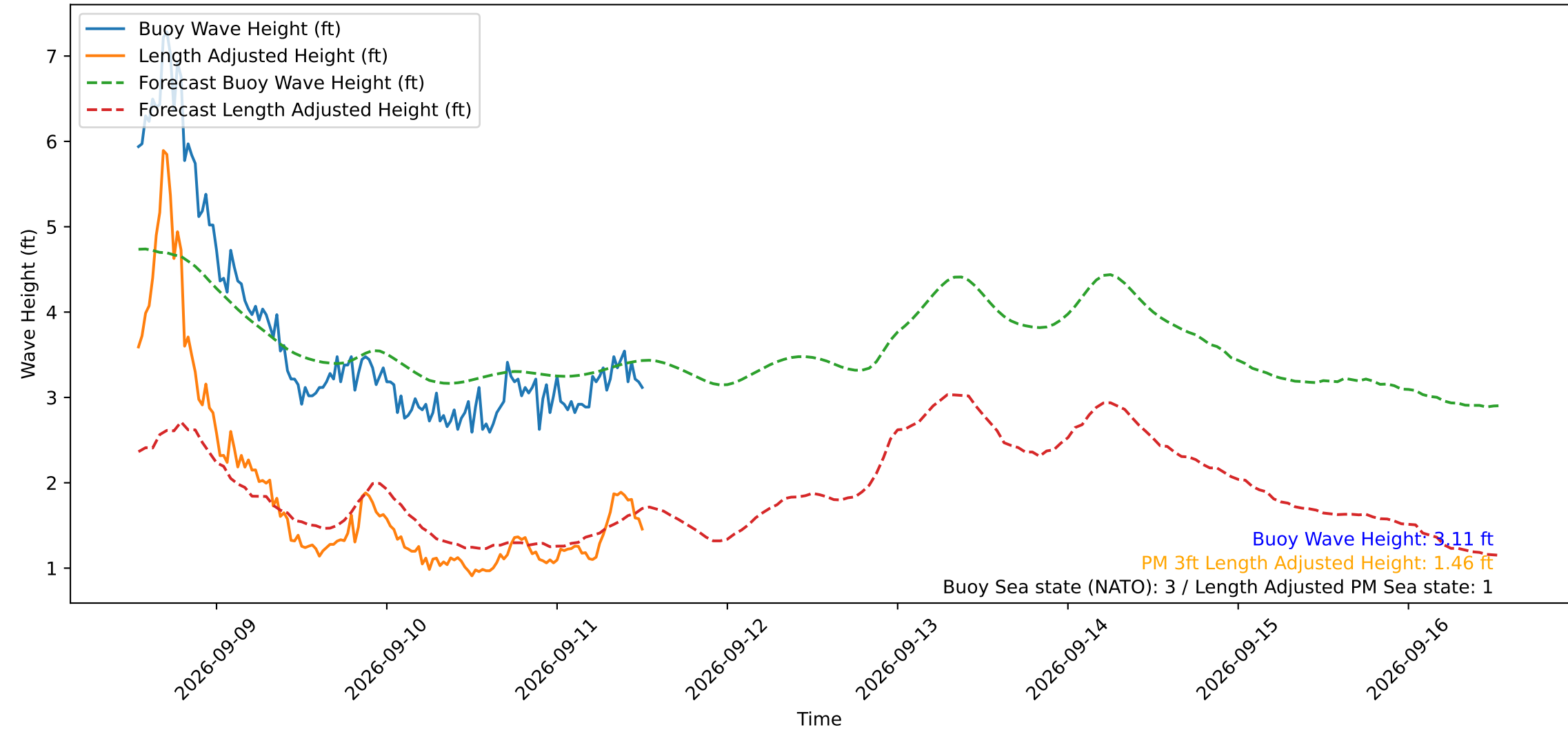
Wave Heights over Time for Green Beach at 2026-09-11 12:41:11
