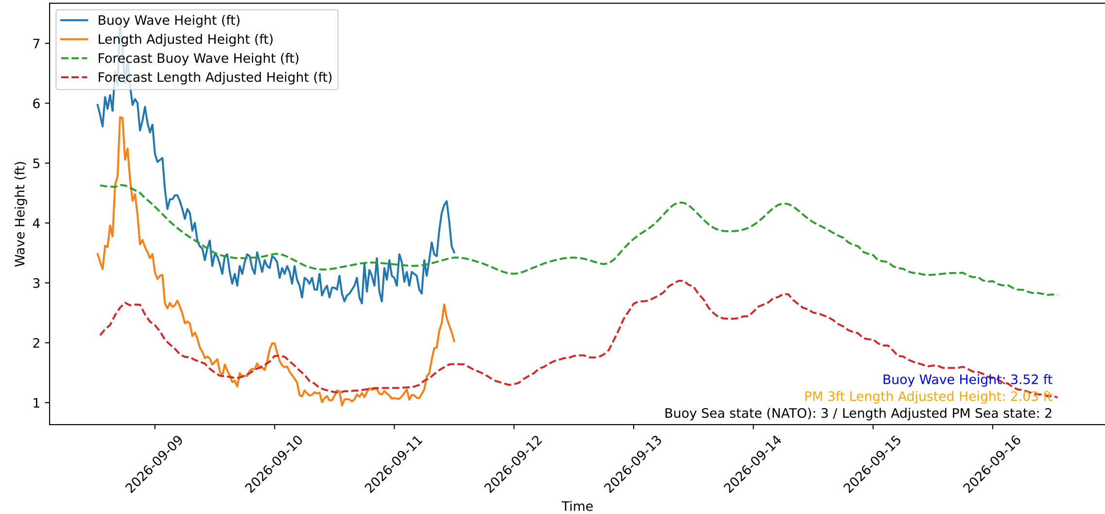
Wave Heights over Time for Oceanside Harbor at 2026-09-11 12:40:30
