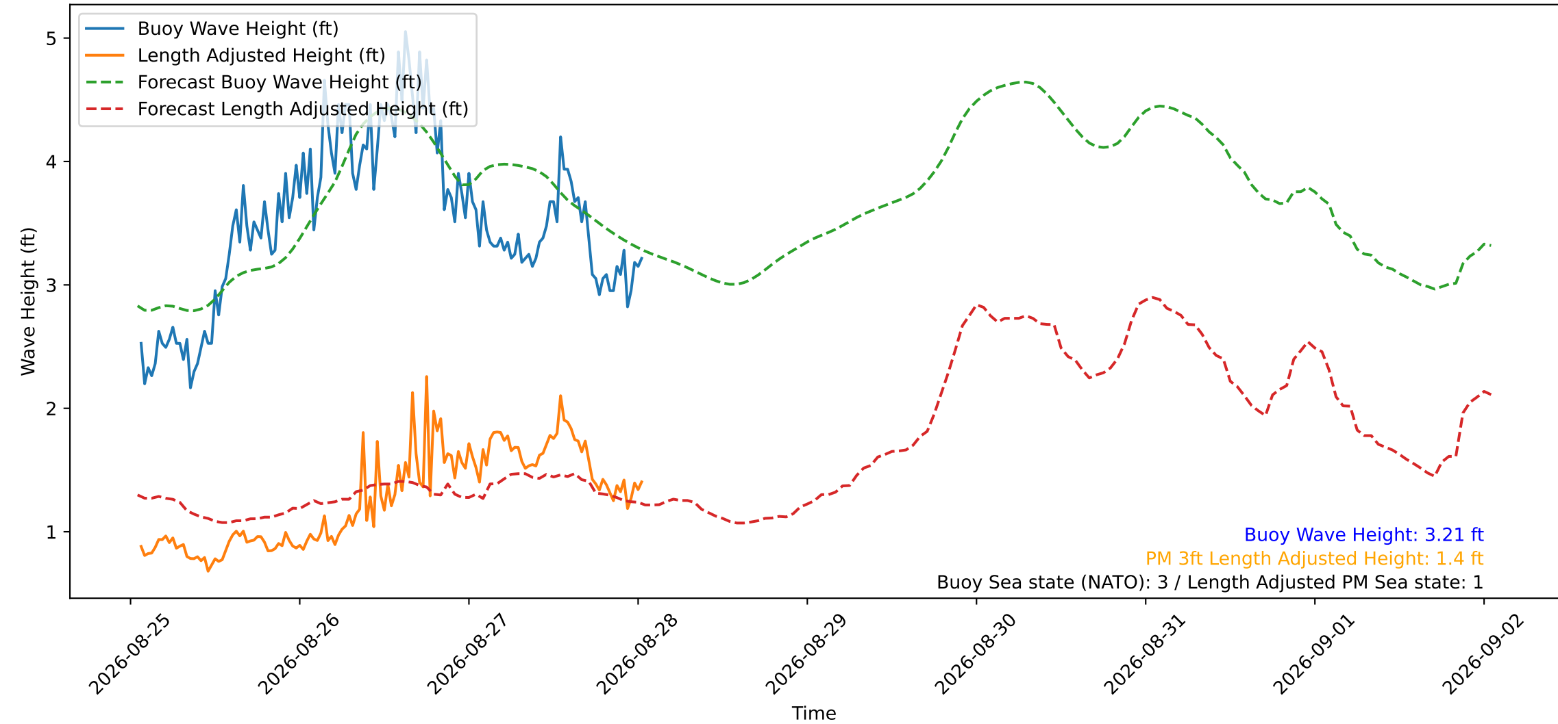
Wave Heights over Time for Red Beach at 2026-08-28 01:20:50
