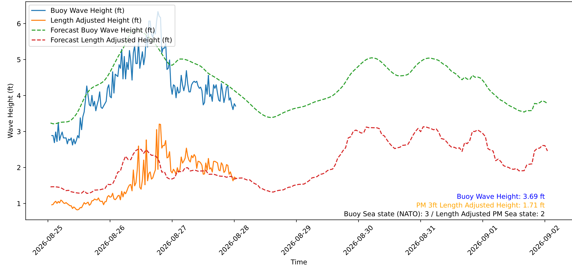
Wave Heights over Time for Green Beach at 2026-08-28 01:21:14
