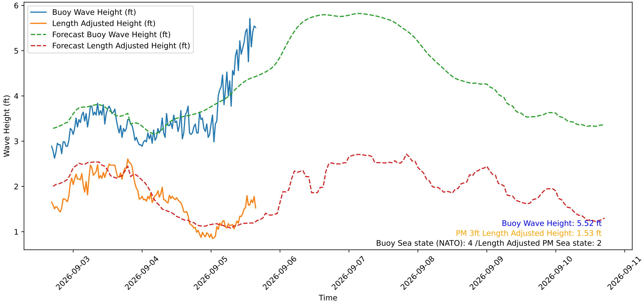
Wave Heights over Time for Oceanside Harbor at 2026-09-05 16:30:30
