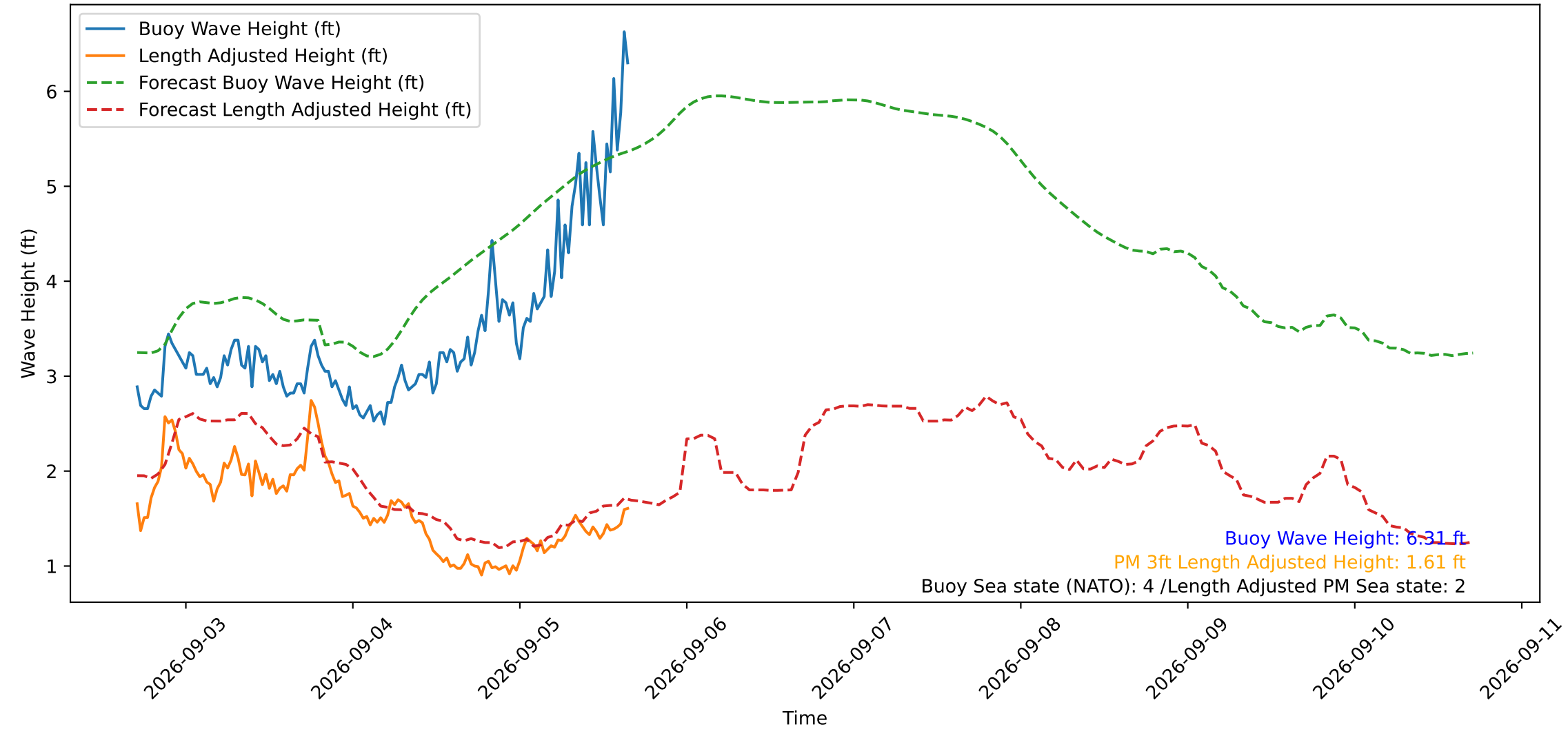
Wave Heights over Time for Green Beach at 2026-09-05 16:31:12
