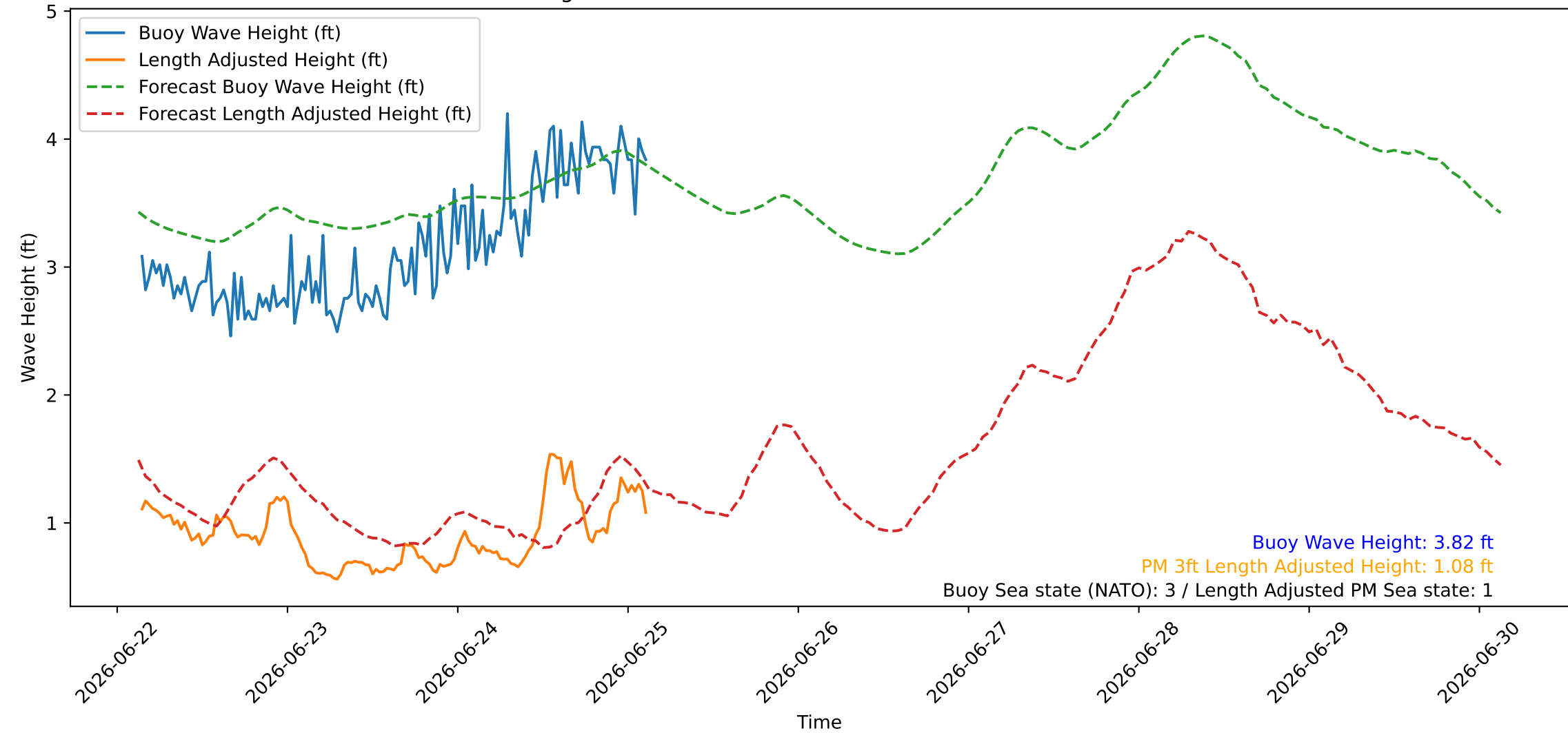
Wave Heights over Time for Green Beach at 2026-06-25 03:21:08
