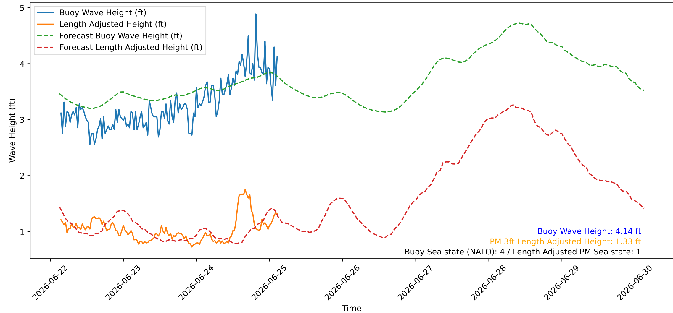
Wave Heights over Time for Oceanside Harbor at 2026-06-25 03:20:25
