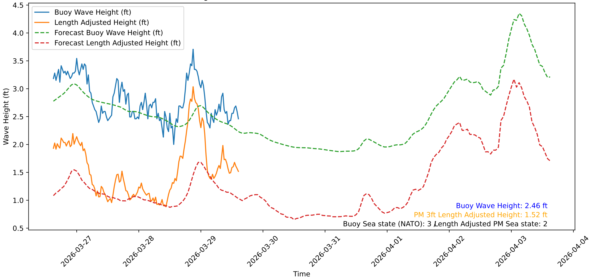
Wave Heights over Time for Green Beach at 2026-03-29 15:11:10
