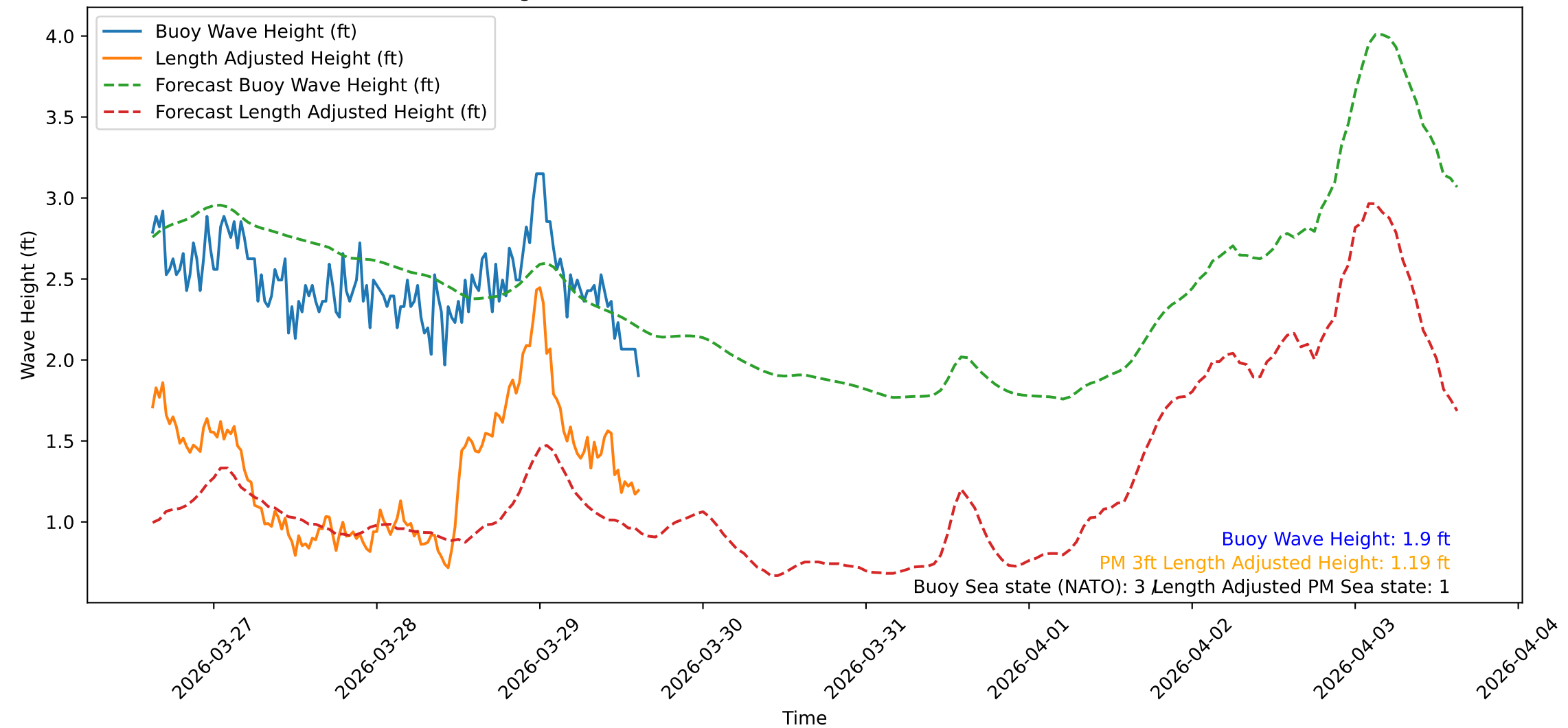
Wave Heights over Time for Oceanside Harbor at 2026-03-29 15:10:31
