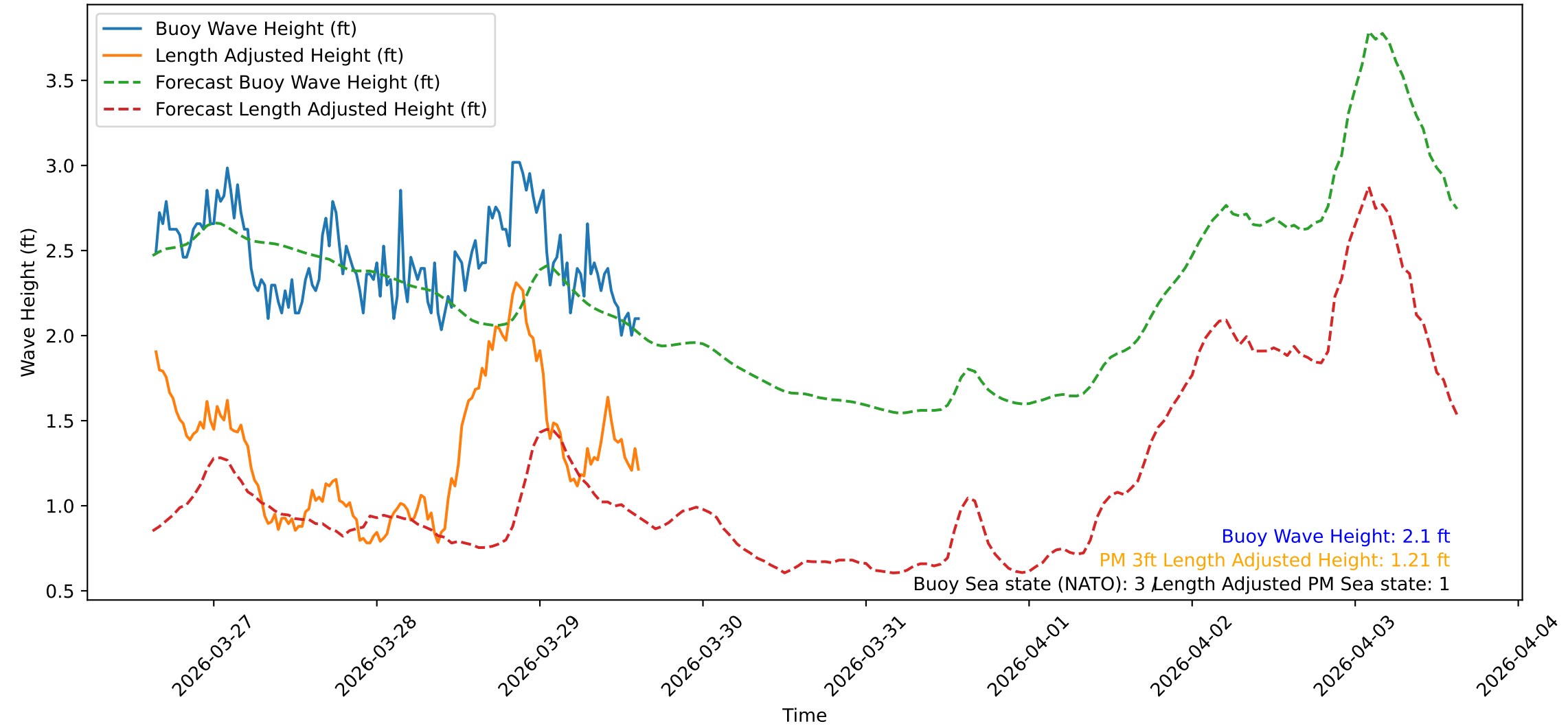
Wave Heights over Time for Red Beach at 2026-03-29 15:10:48
