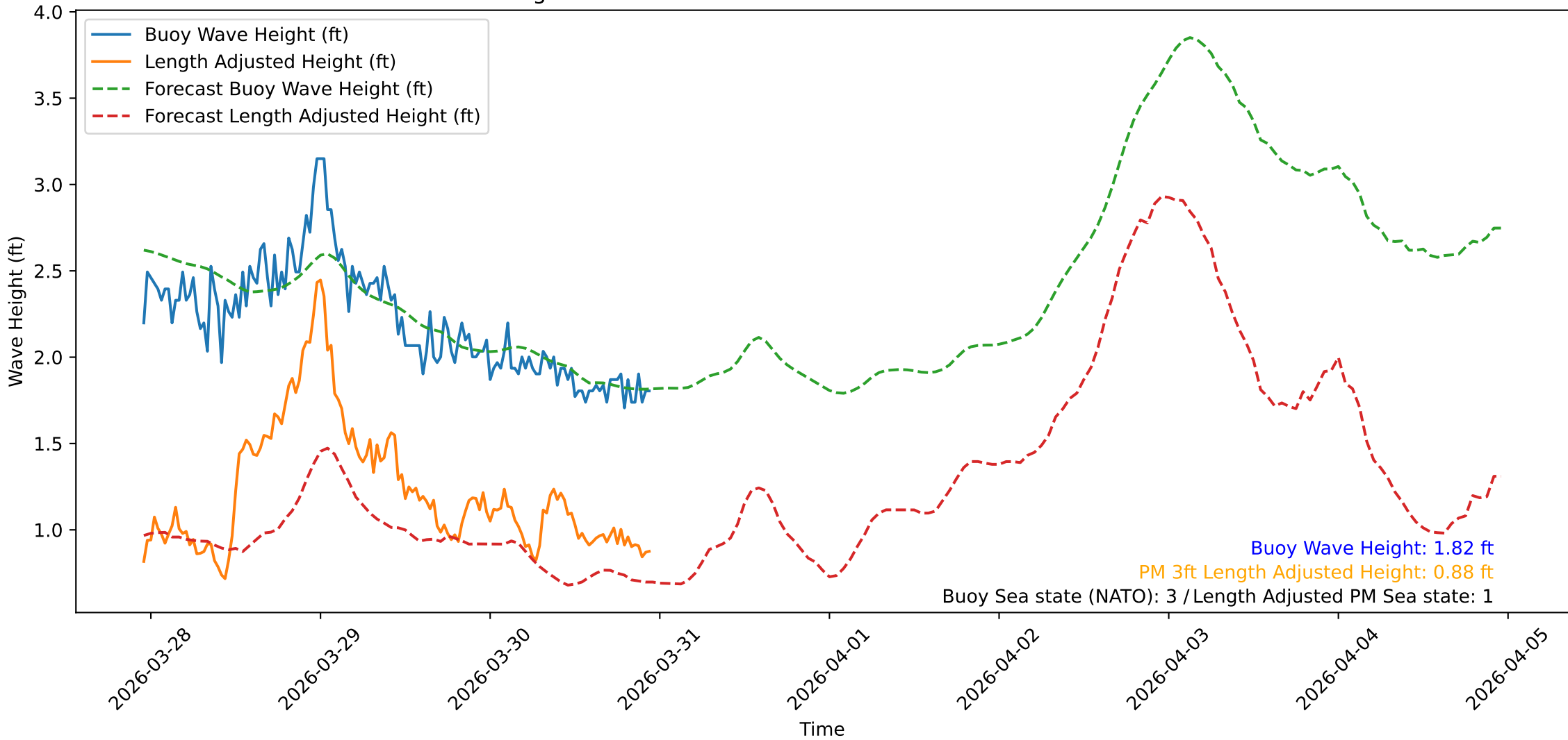
Wave Heights over Time for Oceanside Harbor at 2026-03-30 23:00:31
