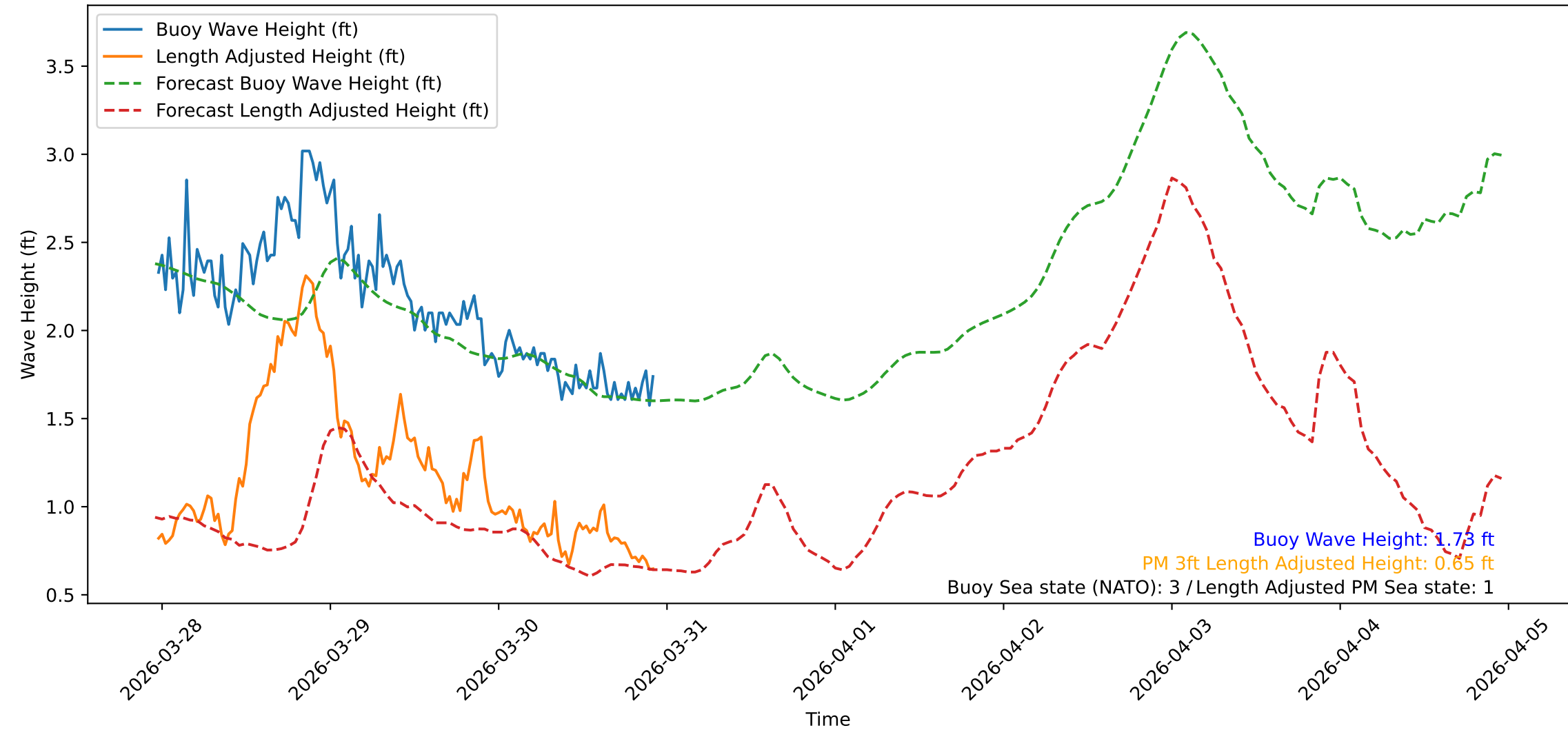
Wave Heights over Time for Red Beach at 2026-03-30 23:00:47
