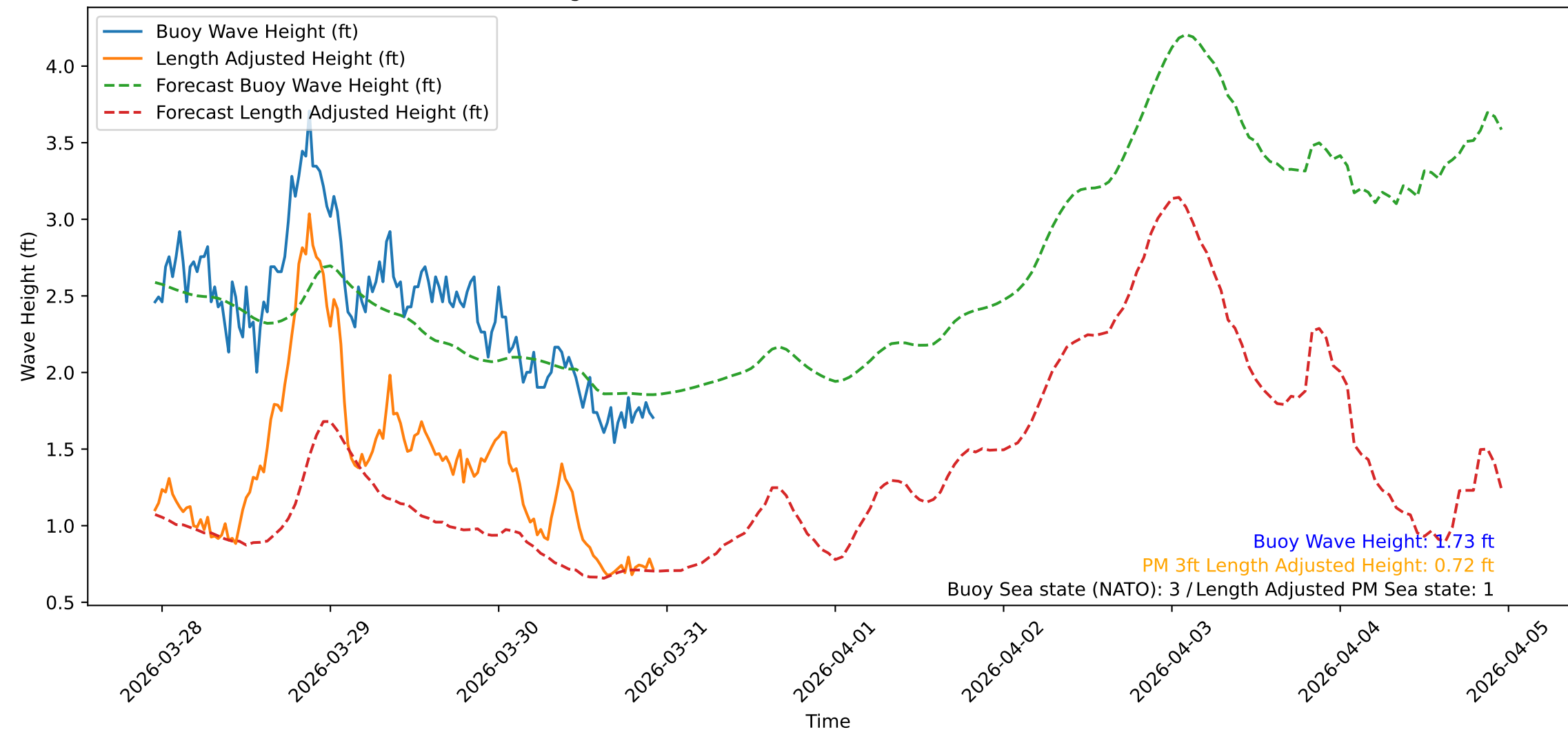
Wave Heights over Time for Green Beach at 2026-03-30 23:01:10
