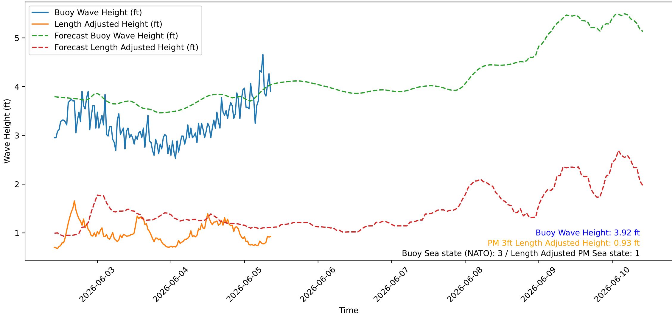
Wave Heights over Time for Red Beach at 2026-06-05 09:30:45
