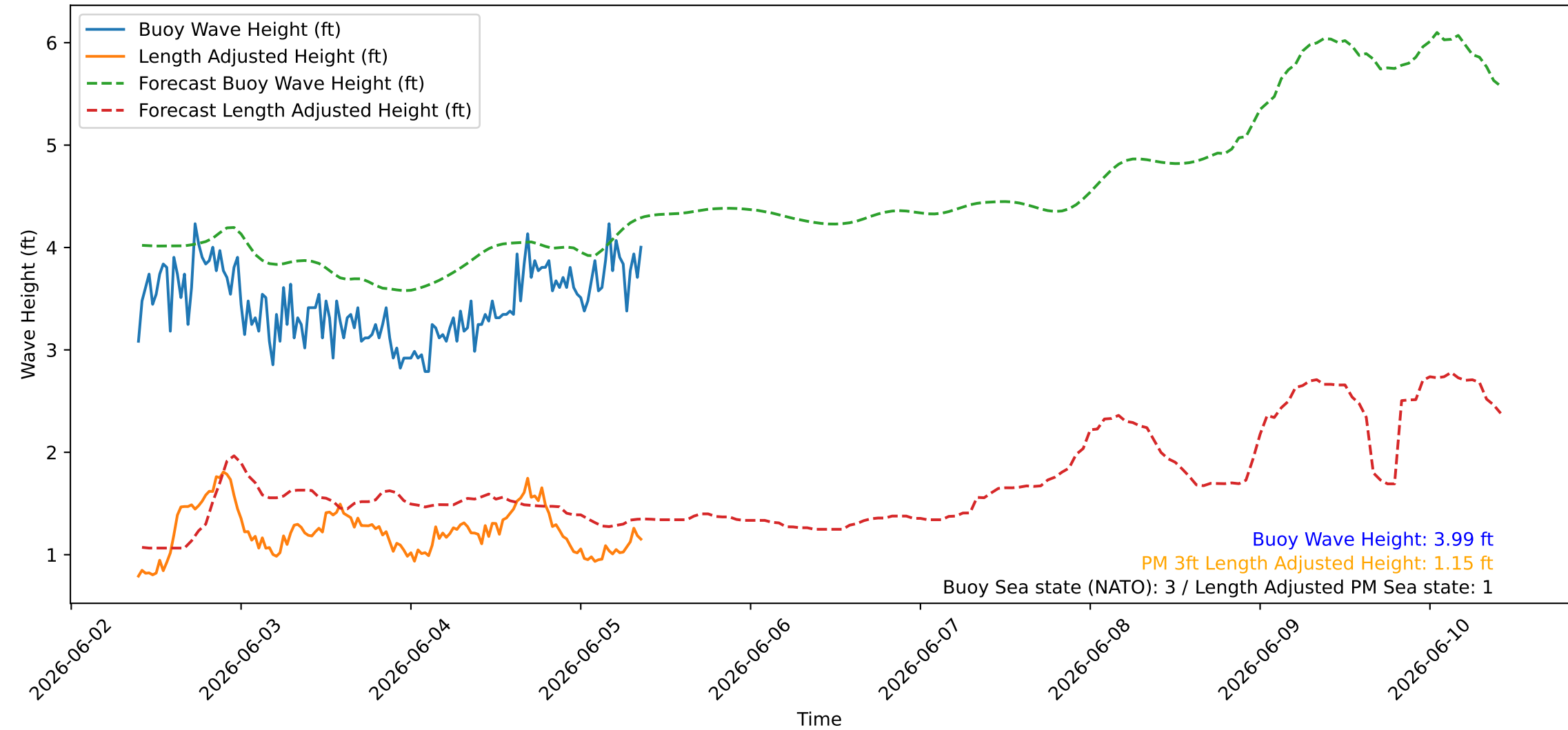
Wave Heights over Time for Green Beach at 2026-06-05 09:31:07
