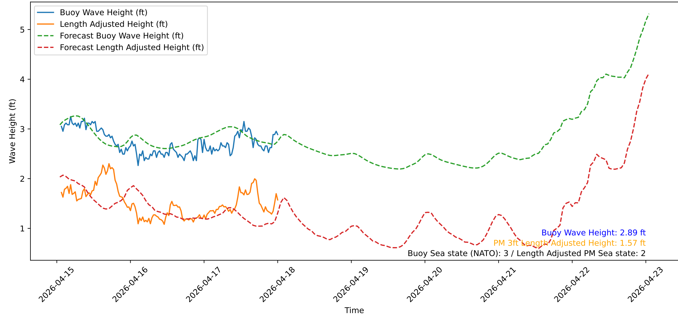
Wave Heights over Time for Red Beach at 2026-04-18 01:00:50
