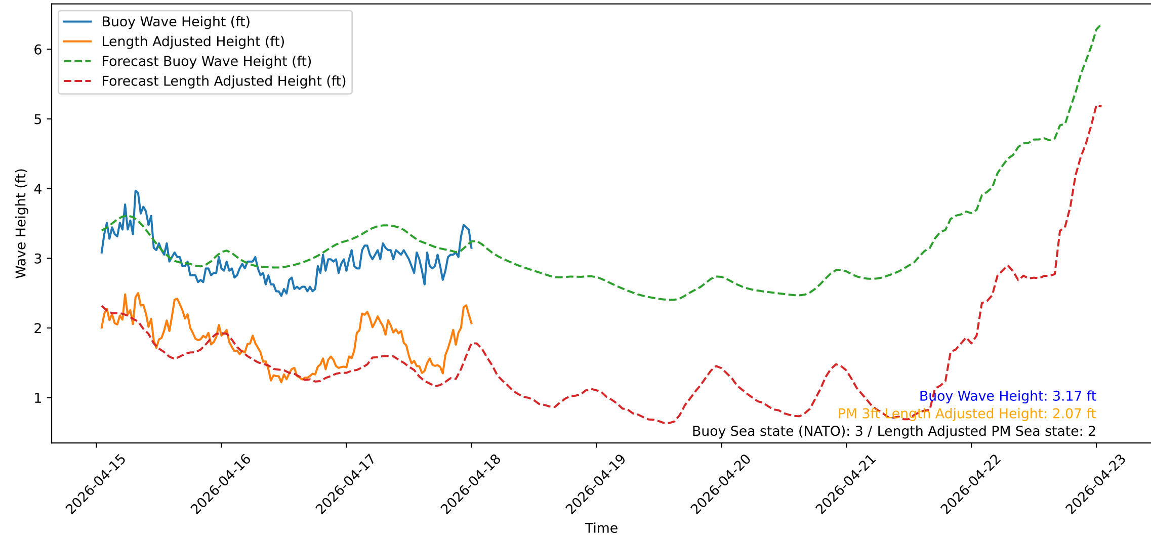
Wave Heights over Time for Green Beach at 2026-04-18 01:01:12
