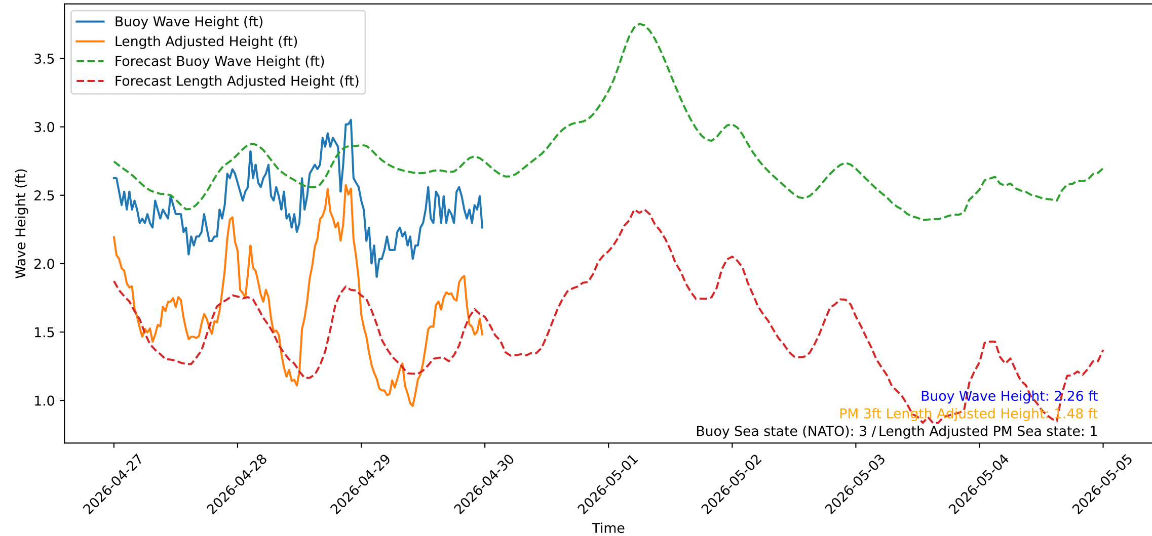
Wave Heights over Time for Oceanside Harbor at 2026-04-30 00:00:31
