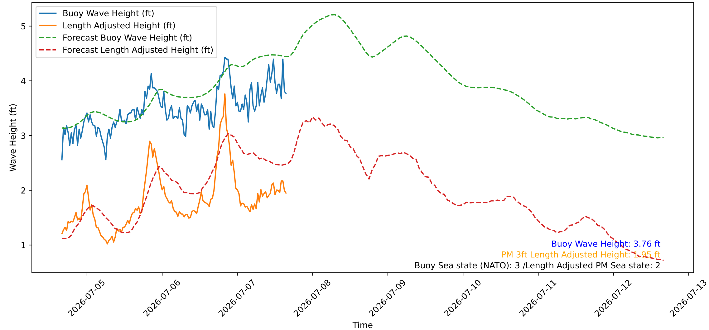
Wave Heights over Time for Green Beach at 2026-07-07 16:11:09
