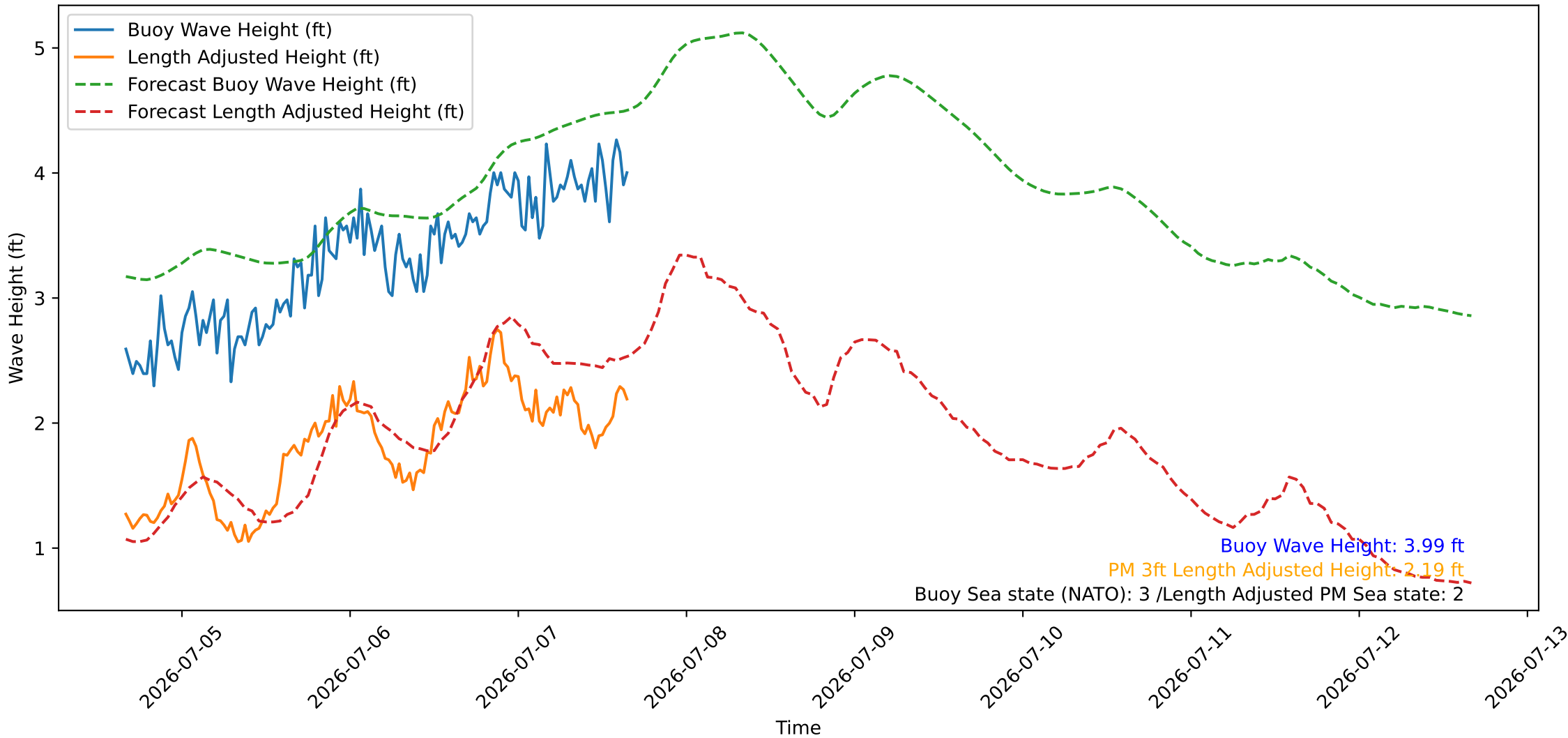
Wave Heights over Time for Oceanside Harbor at 2026-07-07 16:10:26
