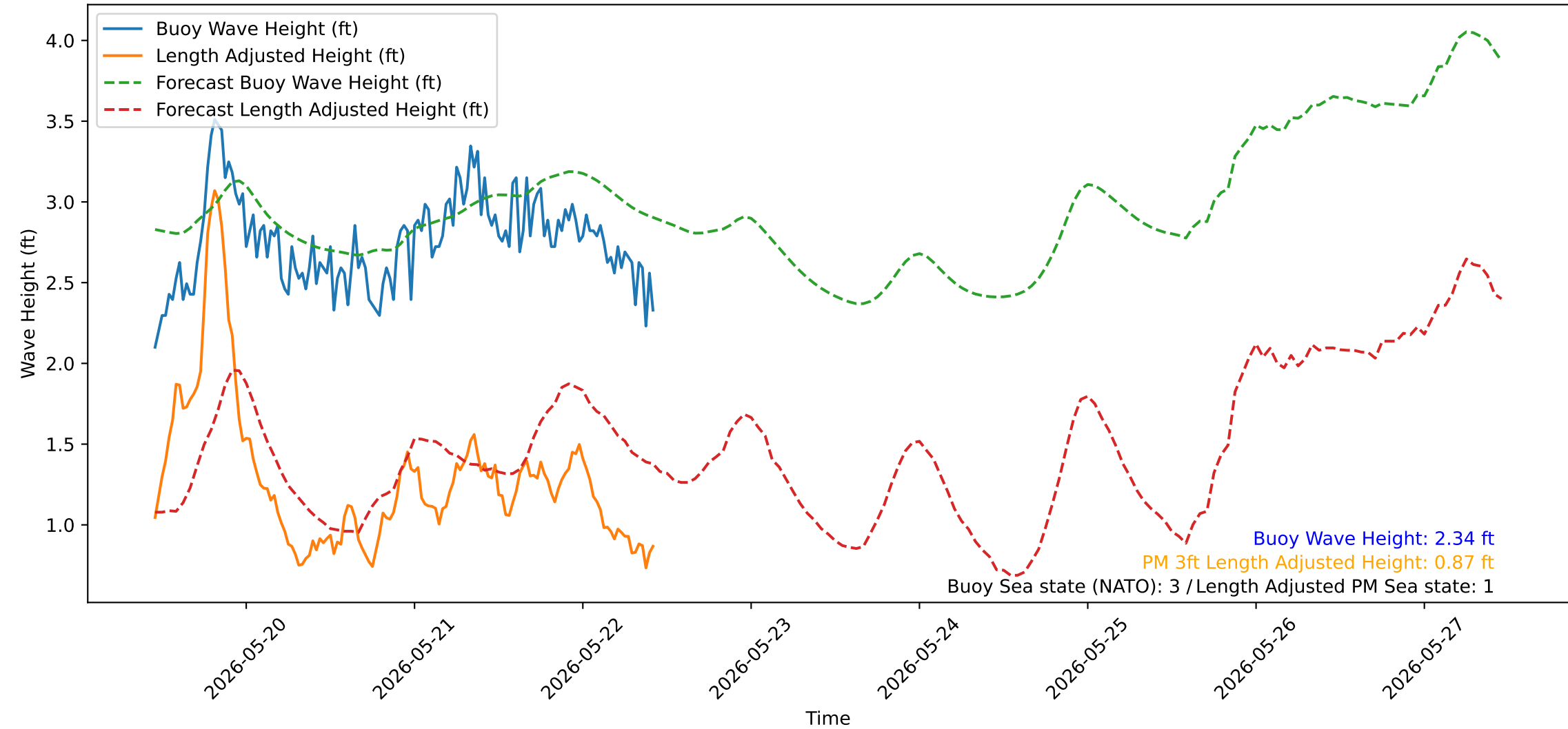
Wave Heights over Time for Red Beach at 2026-05-22 10:50:51
