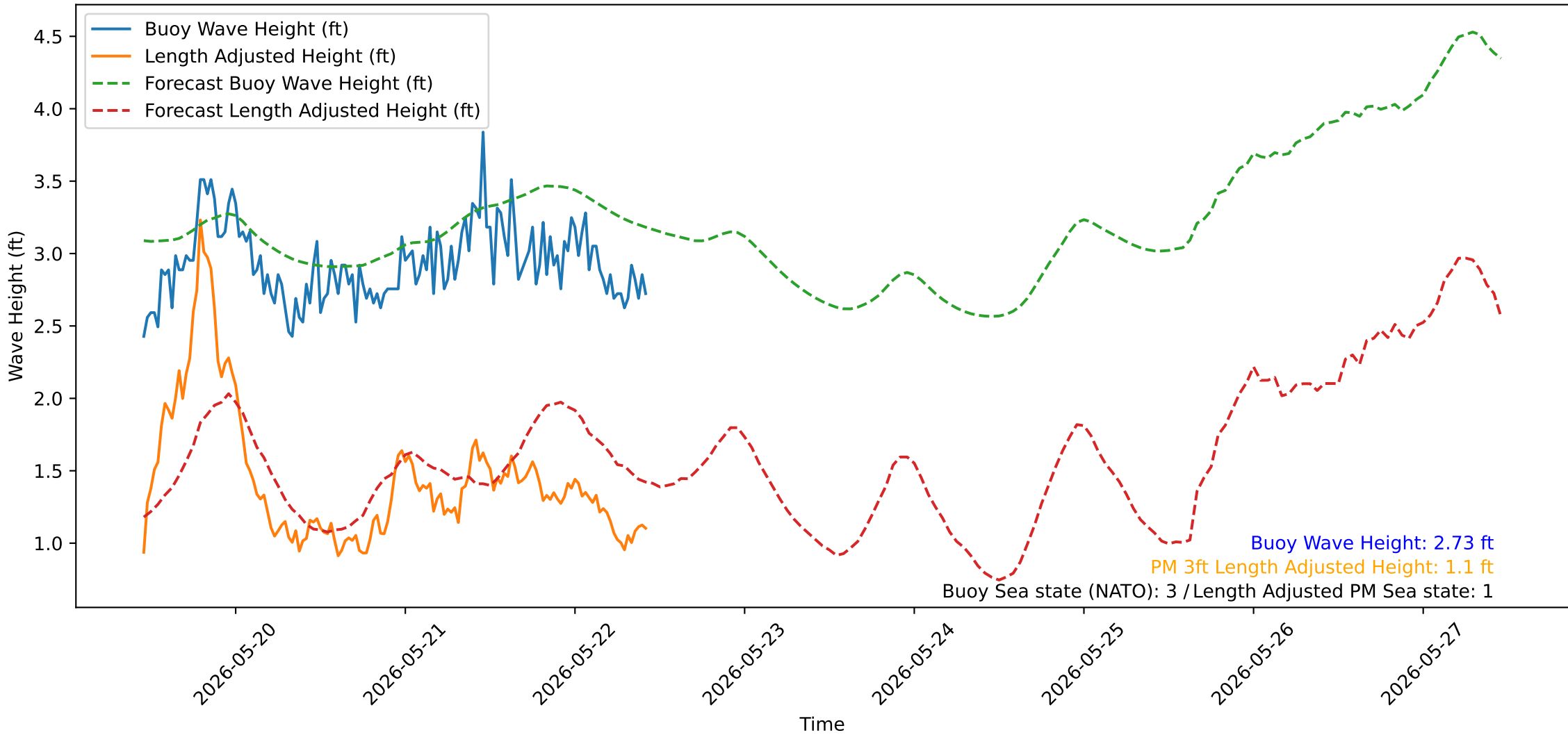
Wave Heights over Time for Oceanside Harbor at 2026-05-22 10:50:31
