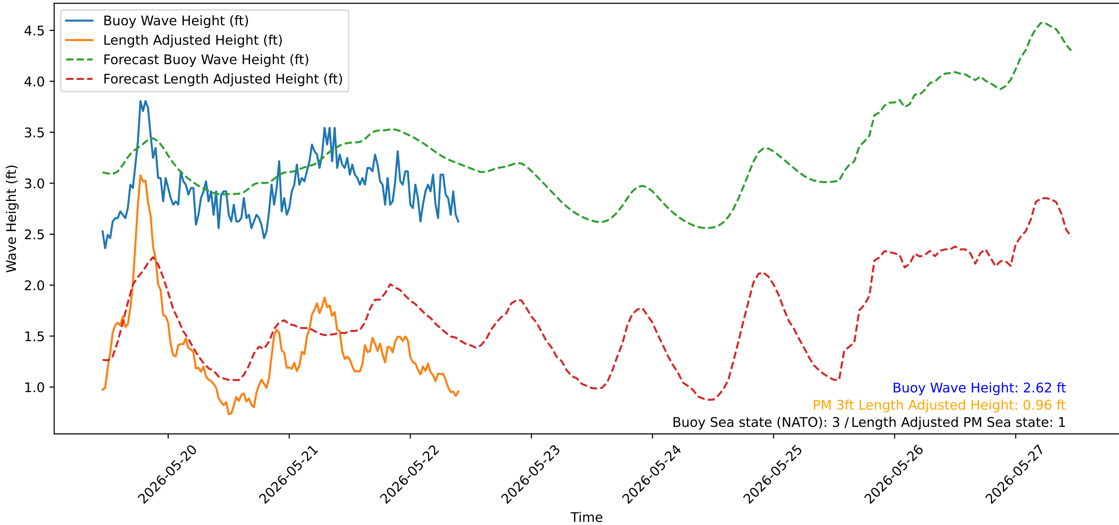
Wave Heights over Time for Green Beach at 2026-05-22 10:51:14
