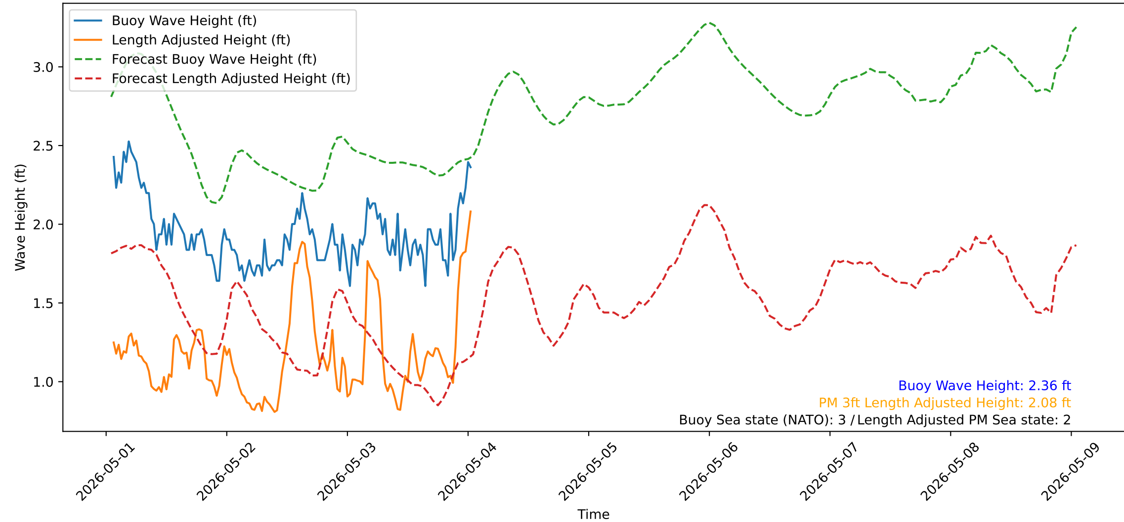
Wave Heights over Time for Red Beach at 2026-05-04 01:10:50
