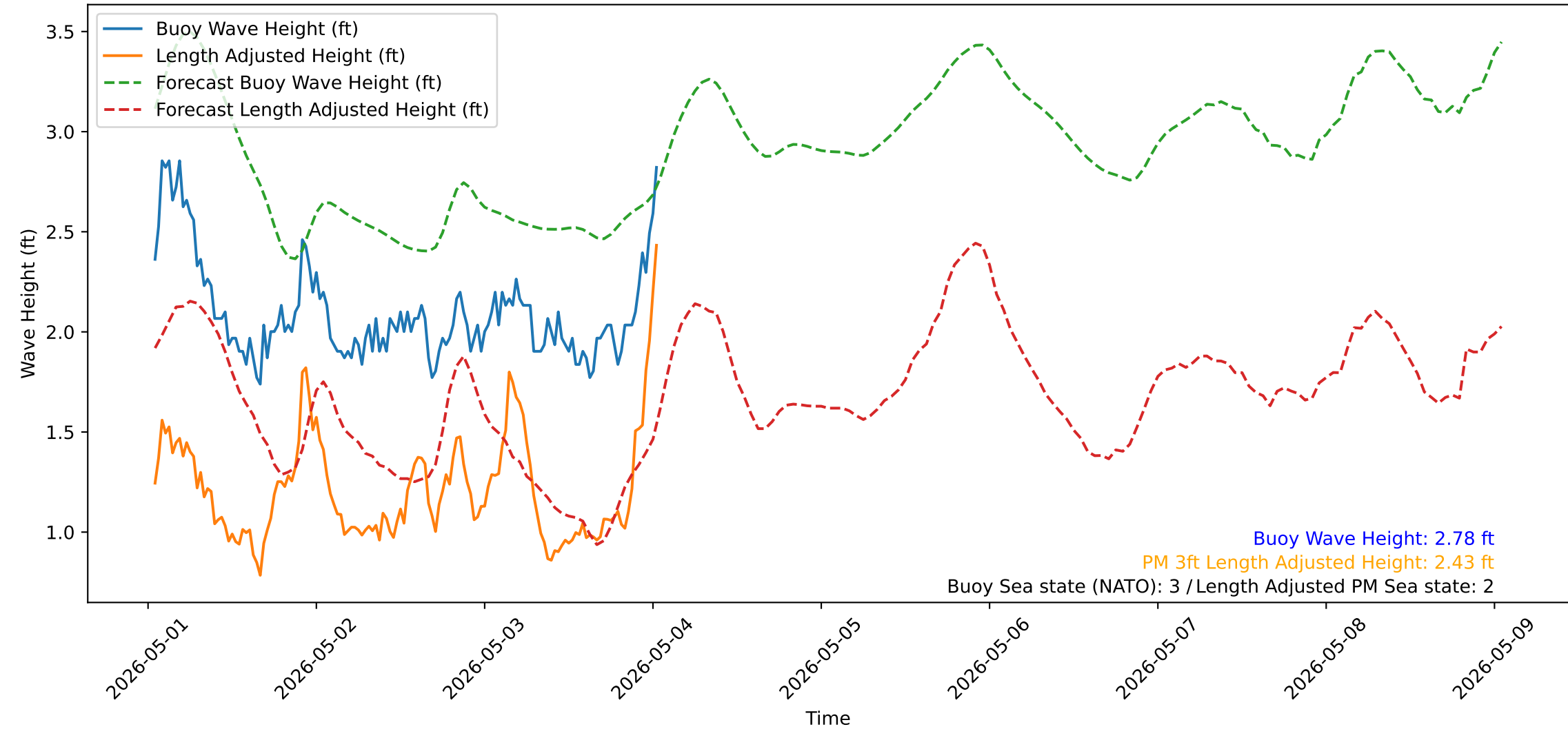
Wave Heights over Time for Green Beach at 2026-05-04 01:11:11
