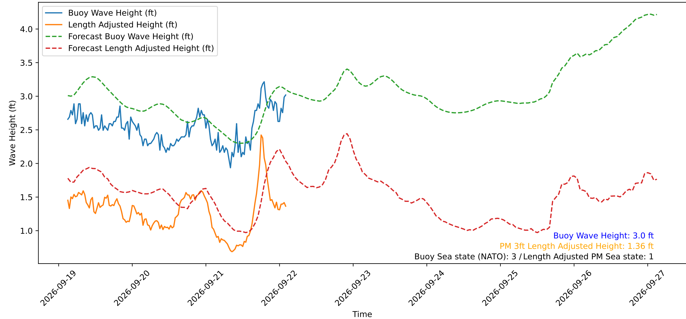
Wave Heights over Time for Green Beach at 2026-09-22 02:41:11
