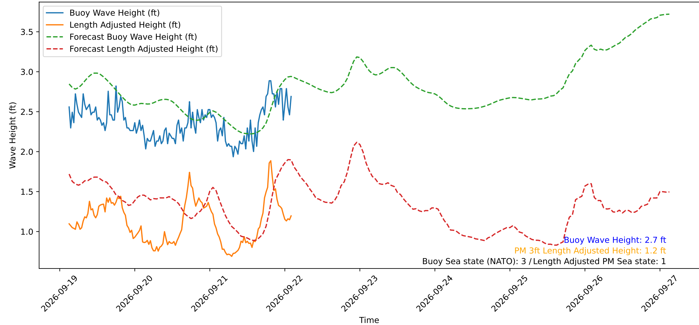
Wave Heights over Time for Red Beach at 2026-09-22 02:40:49
