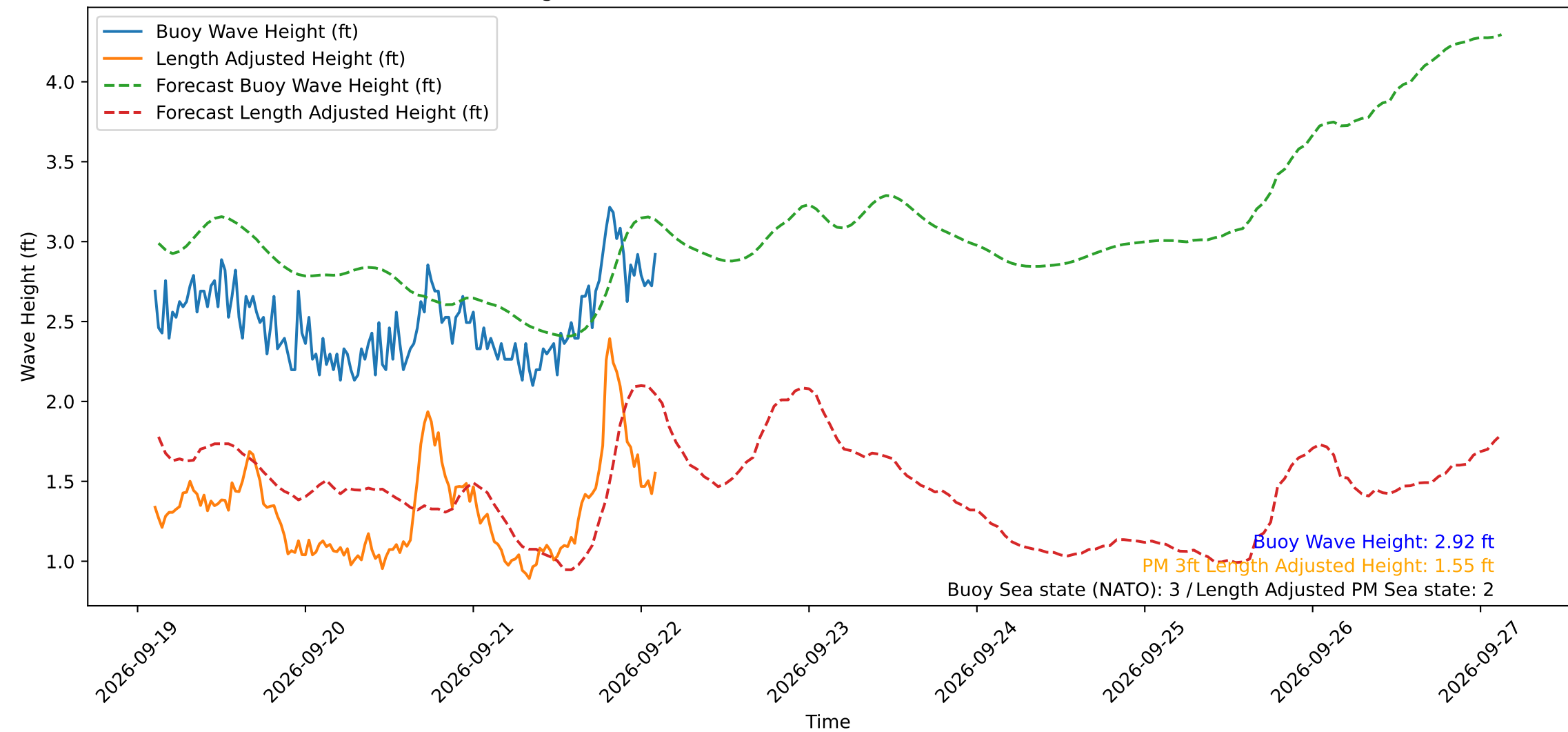
Wave Heights over Time for Oceanside Harbor at 2026-09-22 02:40:29
