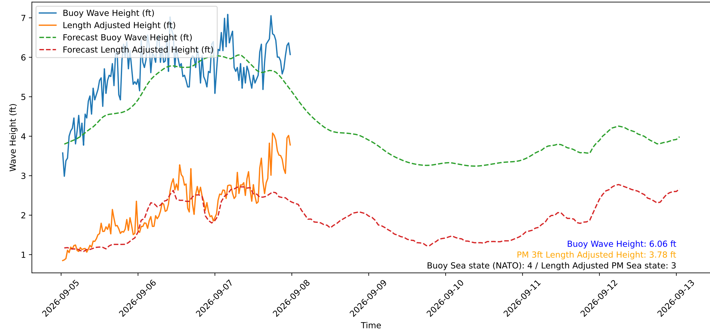
Wave Heights over Time for Oceanside Harbor at 2026-09-08 00:30:29
