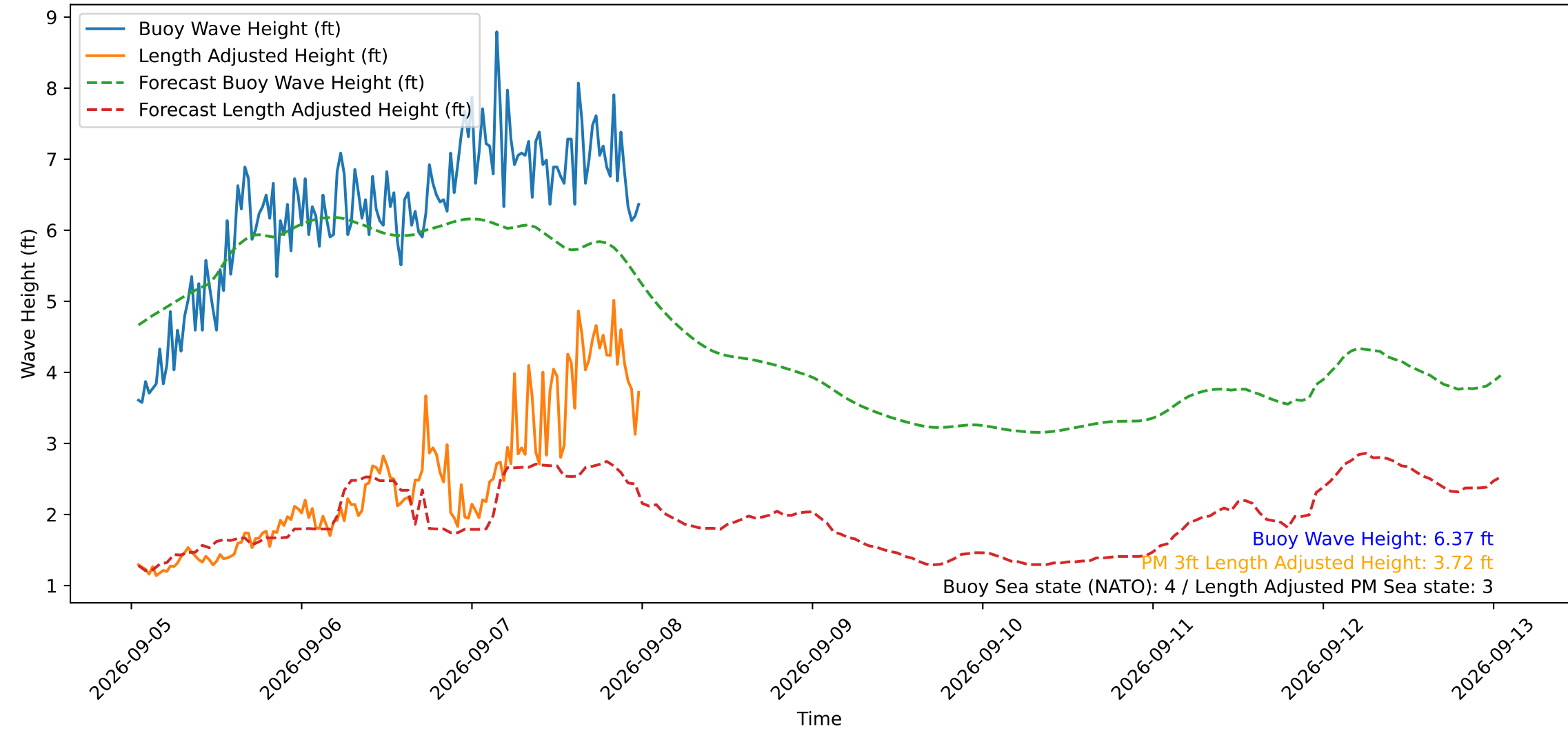
Wave Heights over Time for Green Beach at 2026-09-08 00:31:12
