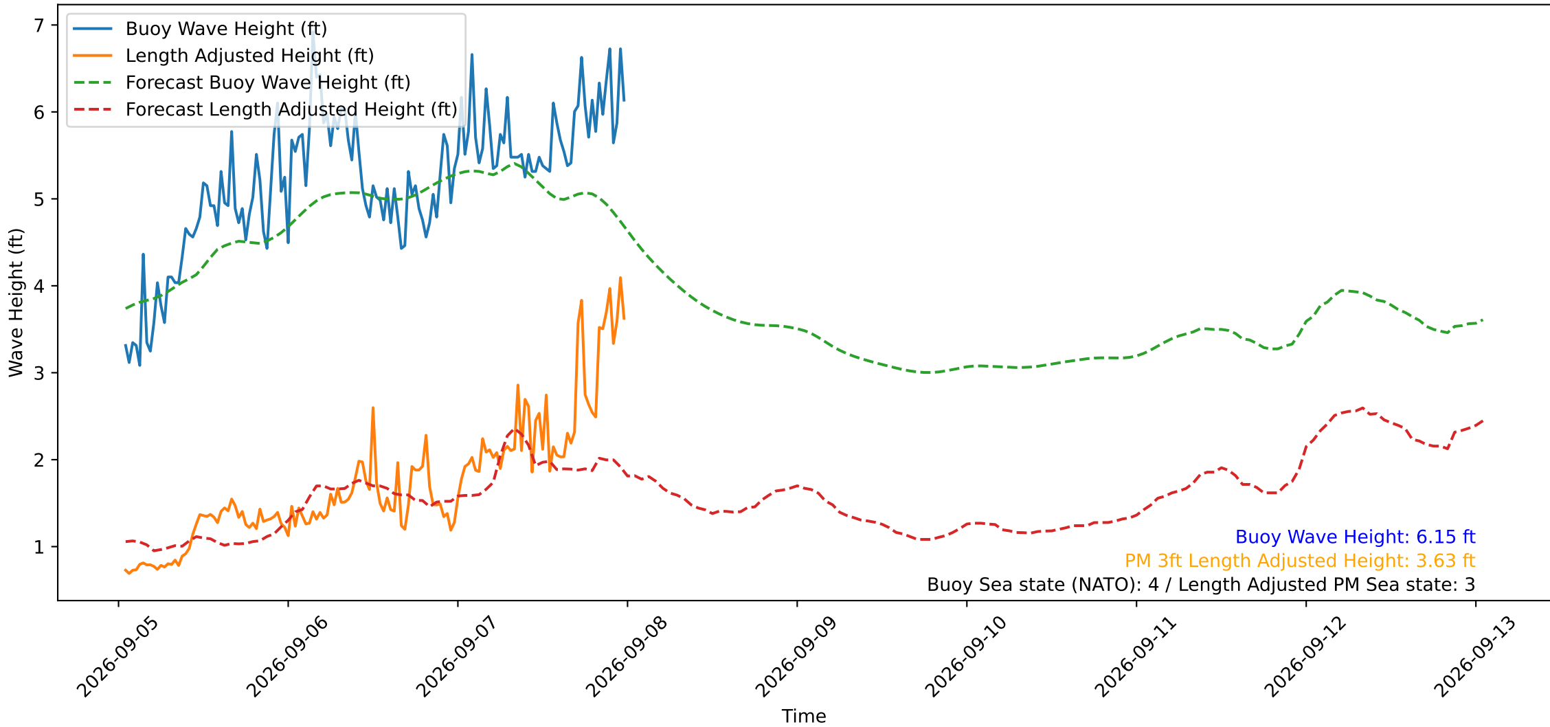
Wave Heights over Time for Red Beach at 2026-09-08 00:30:49
