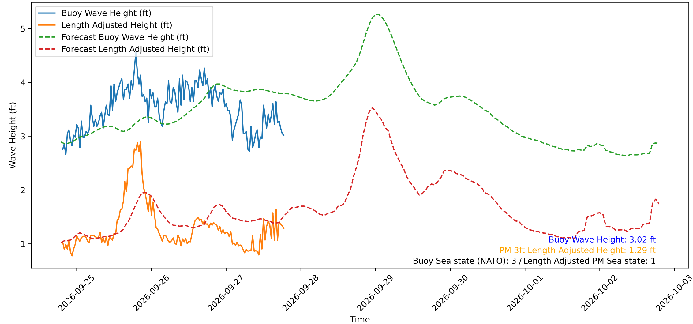
Wave Heights over Time for Green Beach at 2026-09-27 19:21:22
