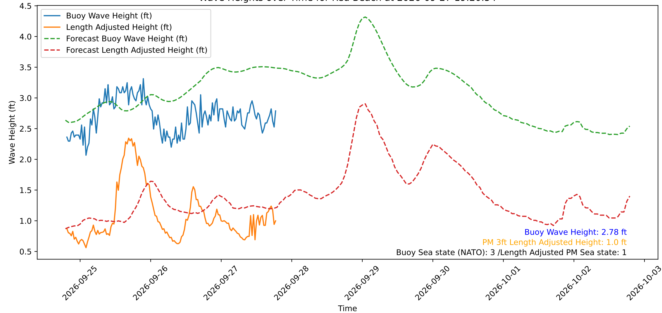
Wave Heights over Time for Red Beach at 2026-09-27 19:20:54
