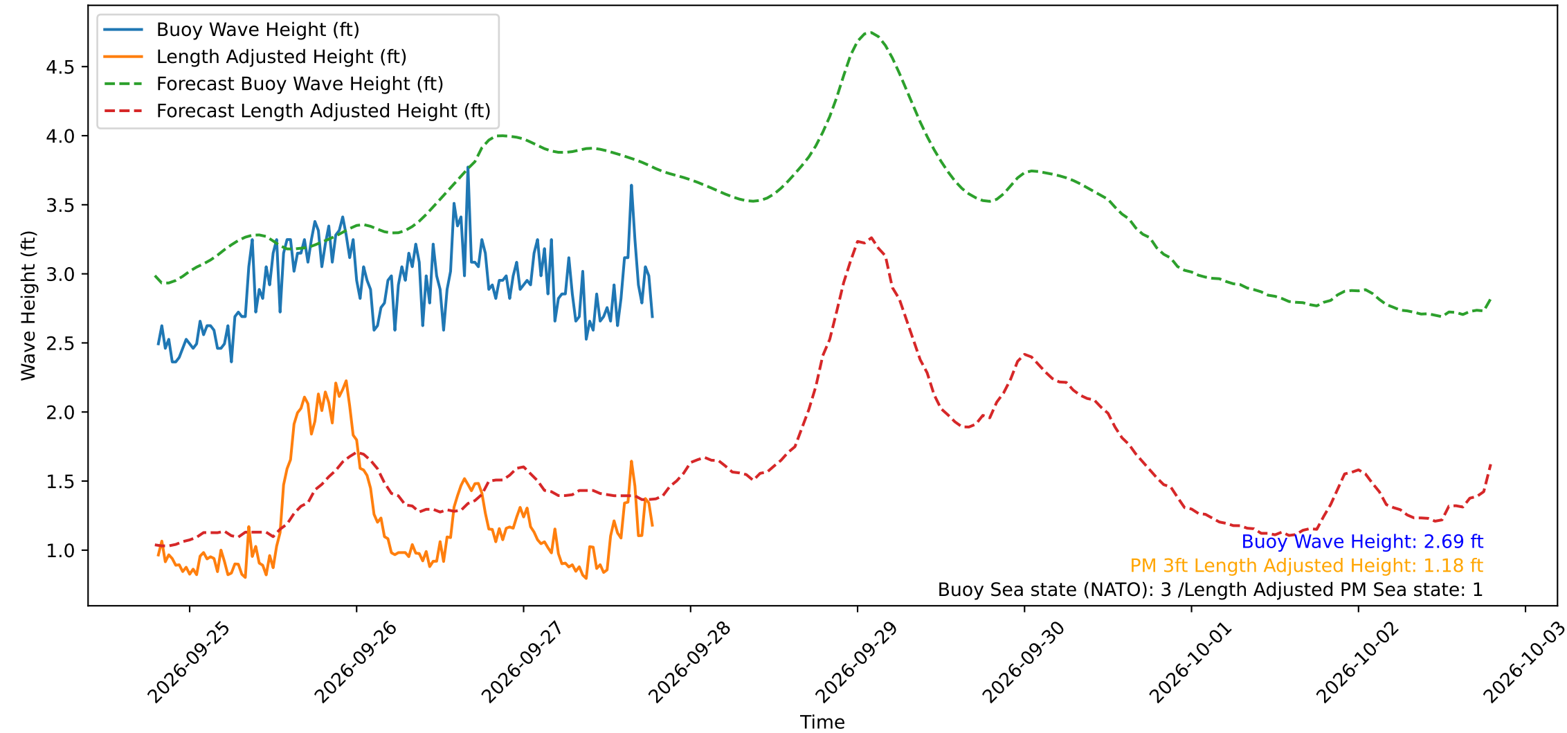
Wave Heights over Time for Oceanside Harbor at 2026-09-27 19:20:31
