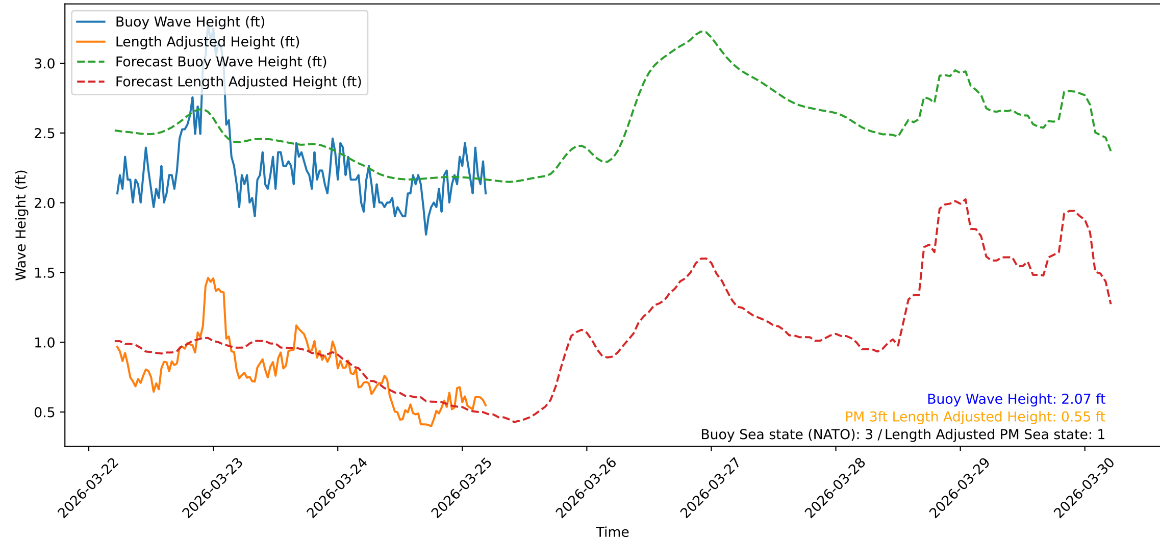
Wave Heights over Time for Green Beach at 2026-03-25 05:21:09
