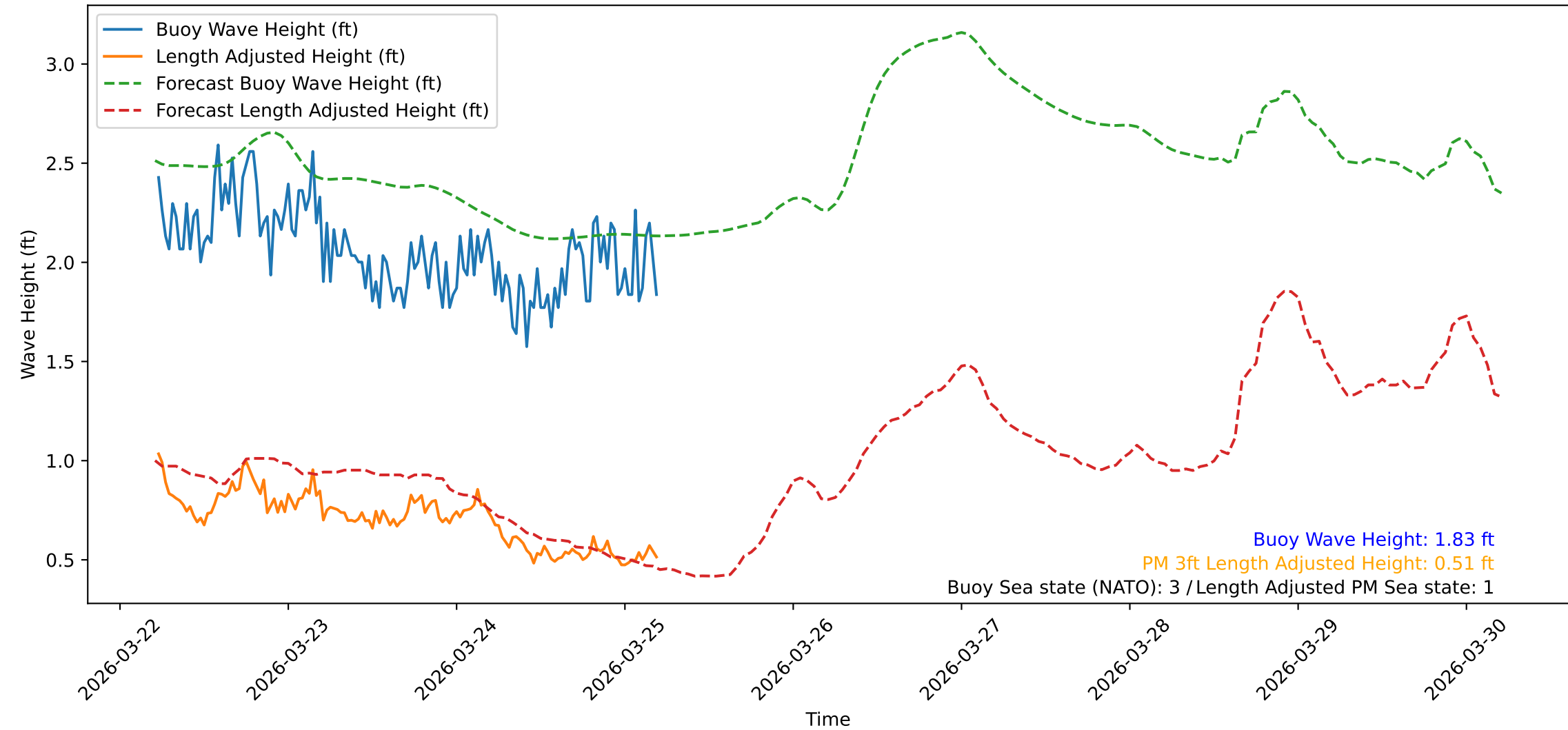
Wave Heights over Time for Oceanside Harbor at 2026-03-25 05:20:31
