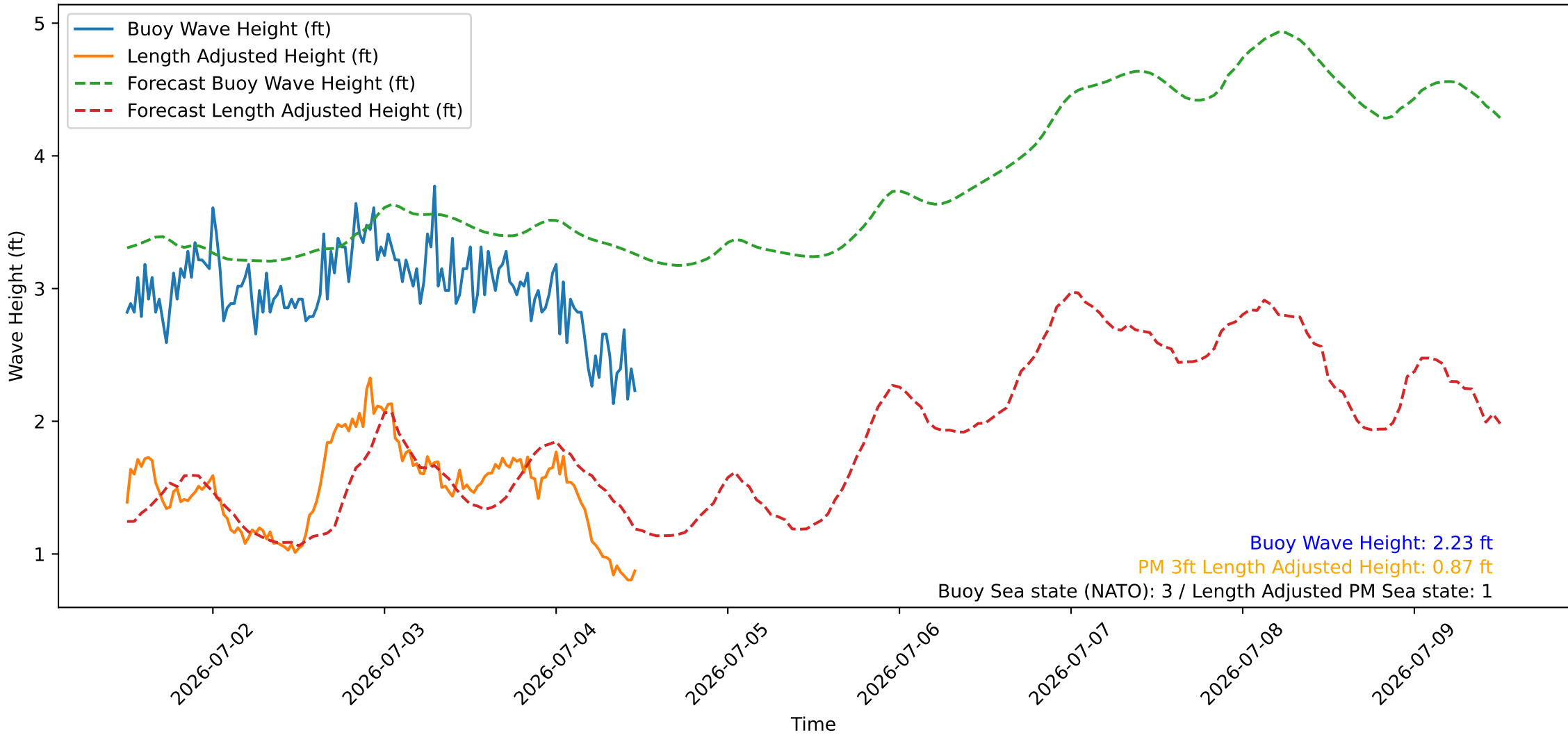
Wave Heights over Time for Oceanside Harbor at 2026-07-04 11:50:26
