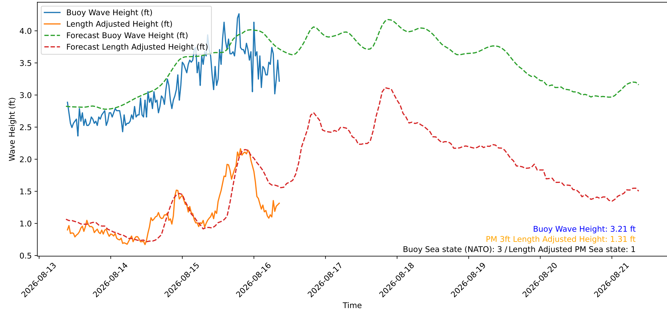
Wave Heights over Time for Green Beach at 2026-08-16 09:11:08
