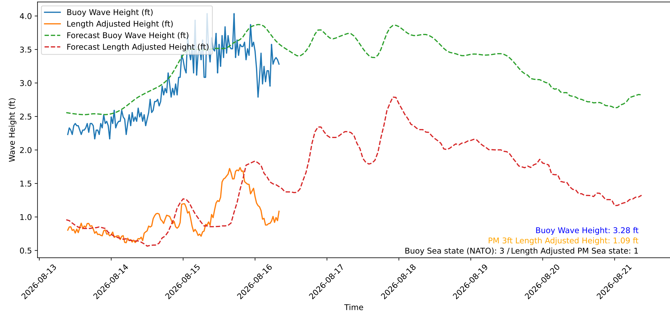
Wave Heights over Time for Red Beach at 2026-08-16 09:10:46
