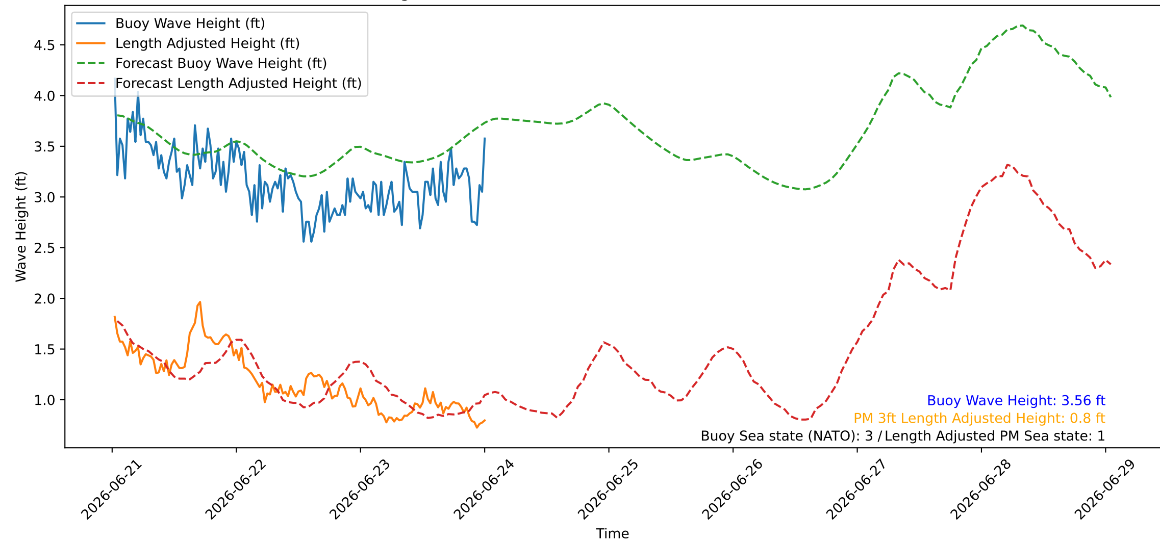
Wave Heights over Time for Oceanside Harbor at 2026-06-24 00:40:26
