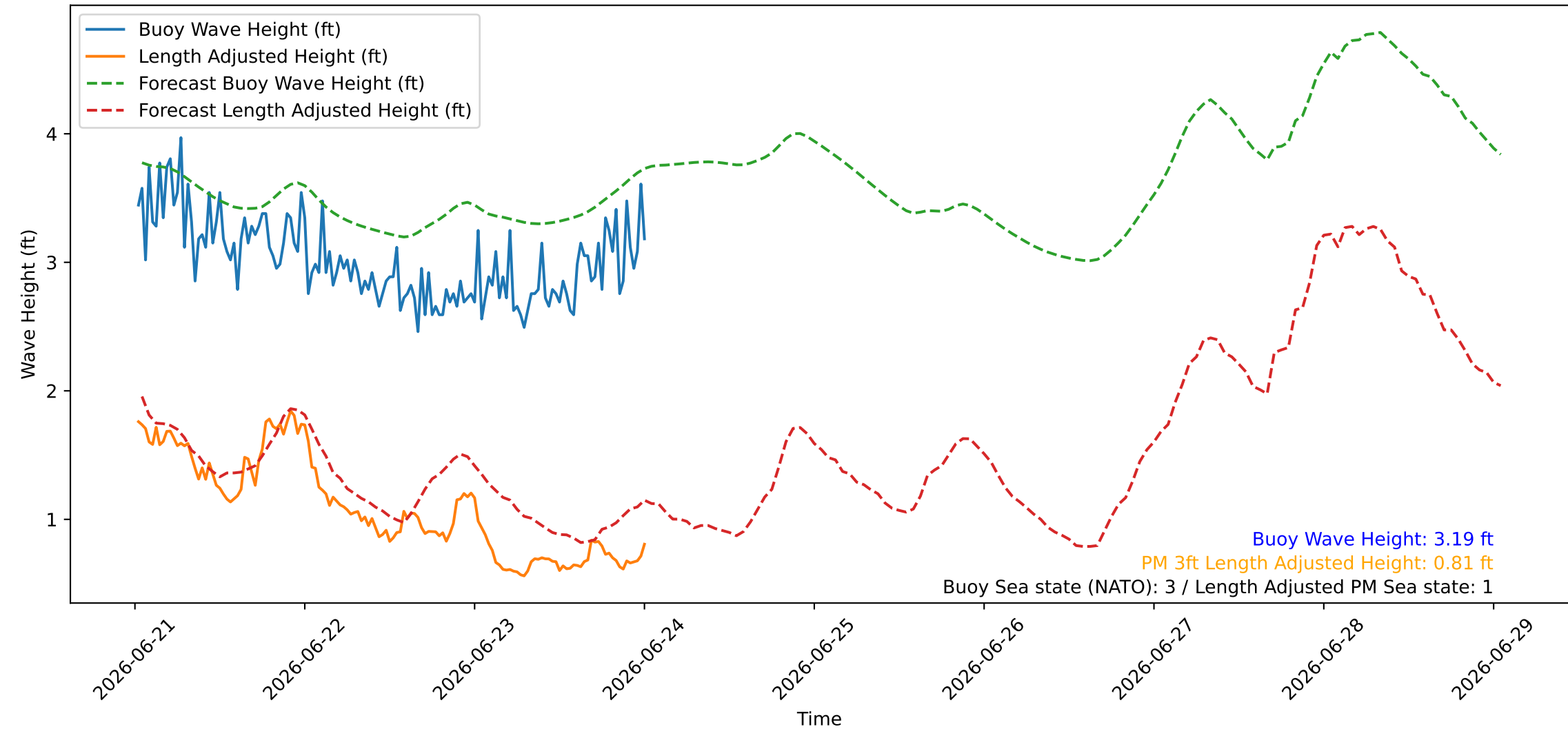
Wave Heights over Time for Green Beach at 2026-06-24 00:41:08
