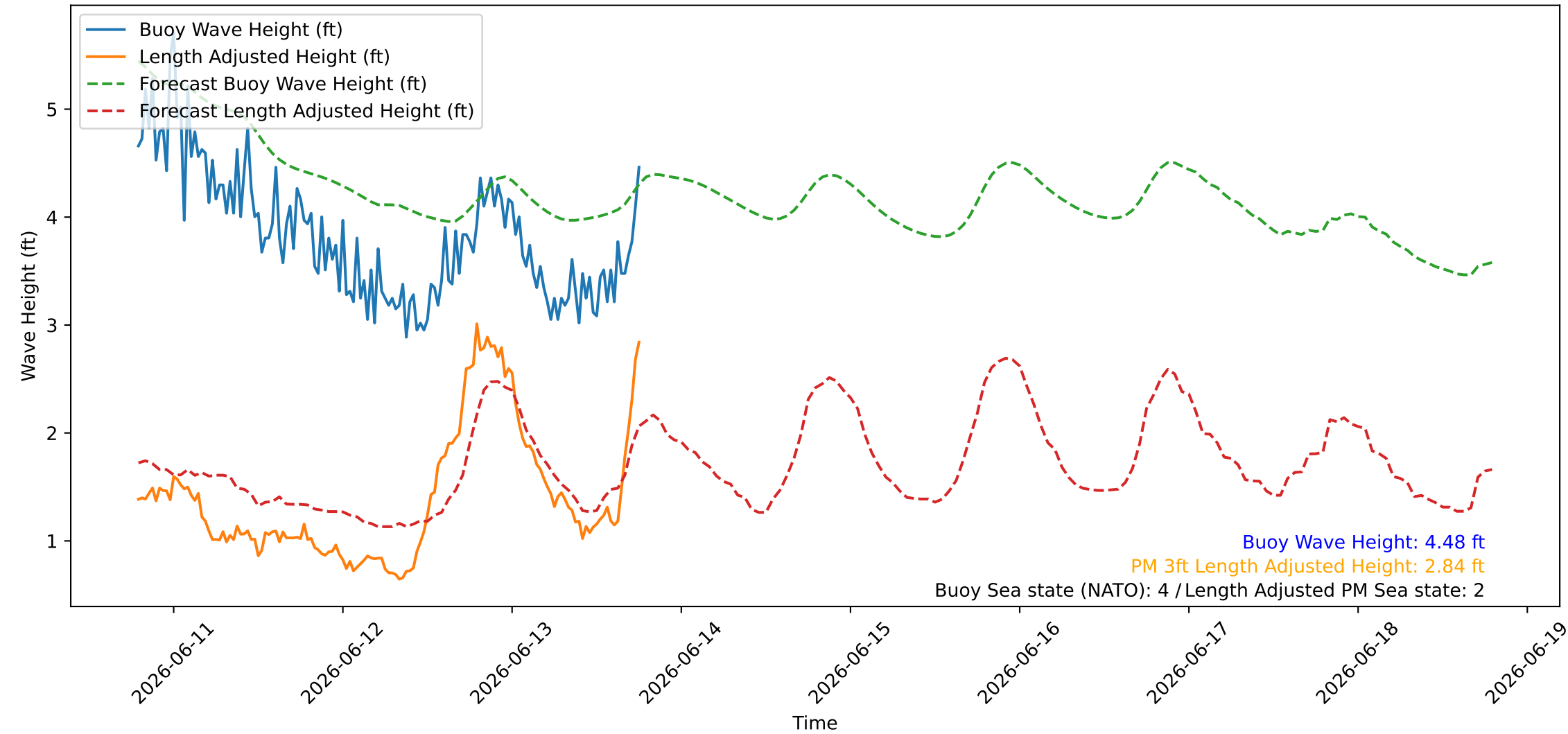
Wave Heights over Time for Green Beach at 2026-06-13 18:51:09
