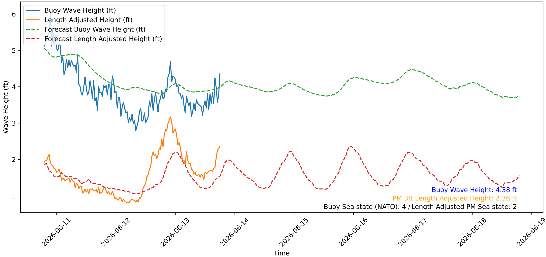
Wave Heights over Time for Oceanside Harbor at 2026-06-13 18:50:26
