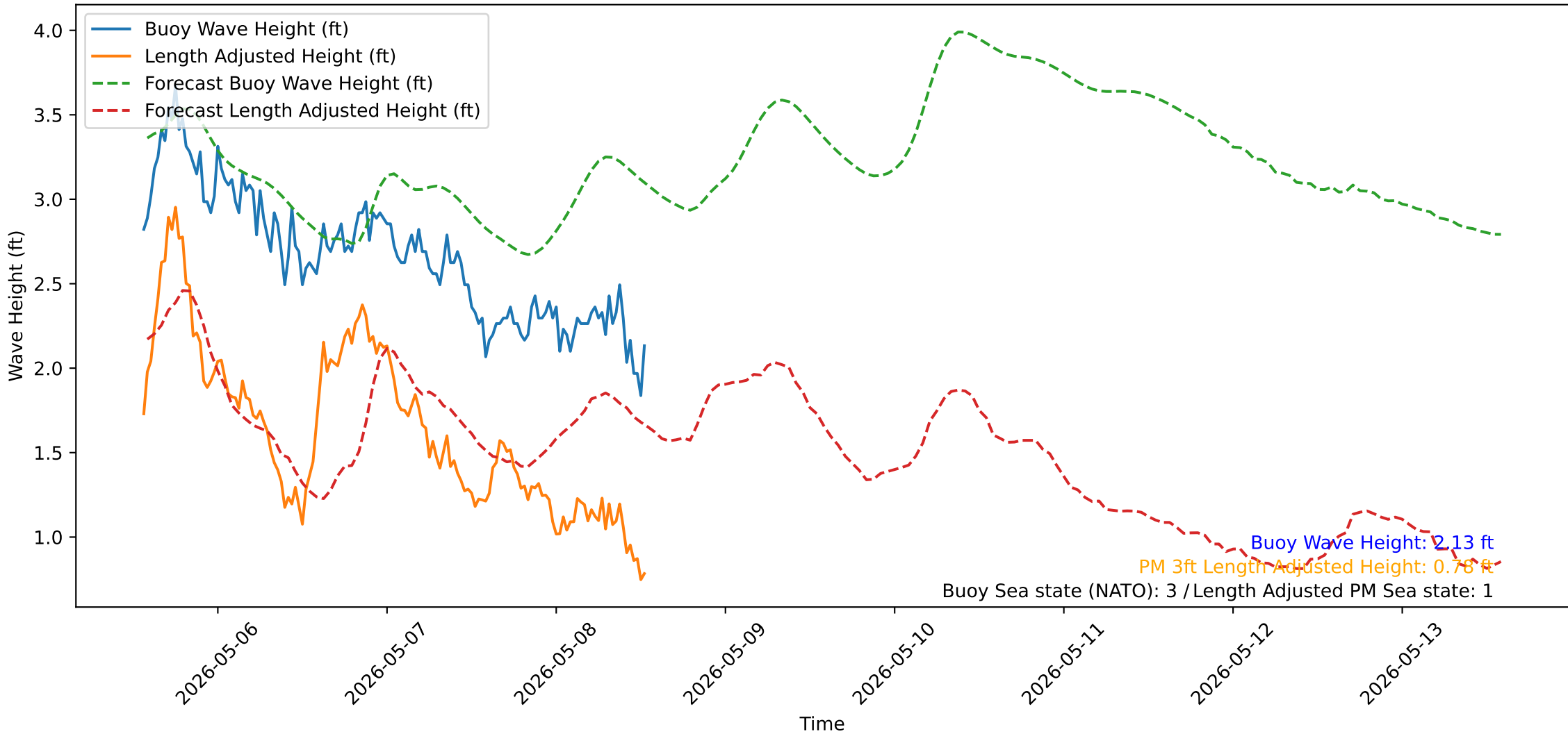
Wave Heights over Time for Green Beach at 2026-05-08 13:31:12
