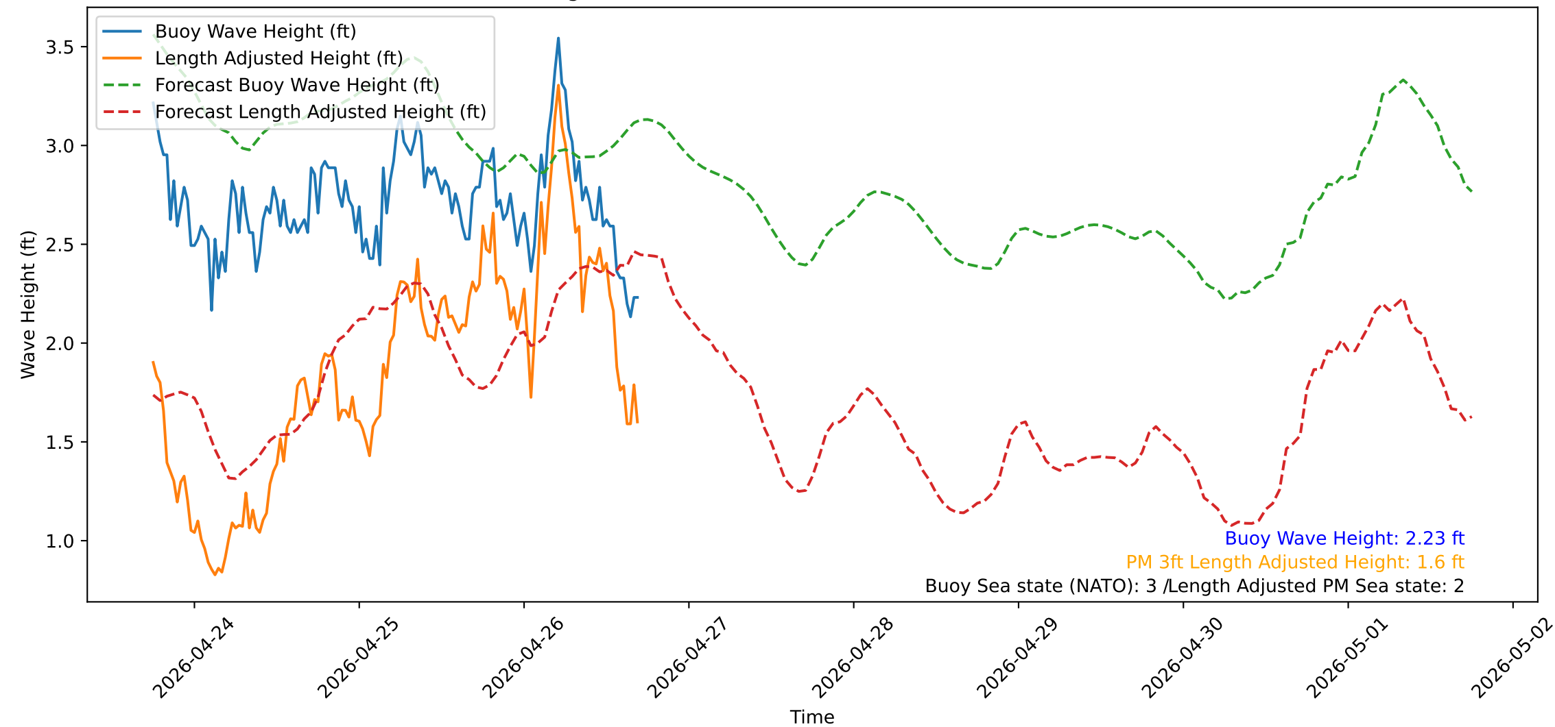
Wave Heights over Time for Red Beach at 2026-04-26 17:30:50
