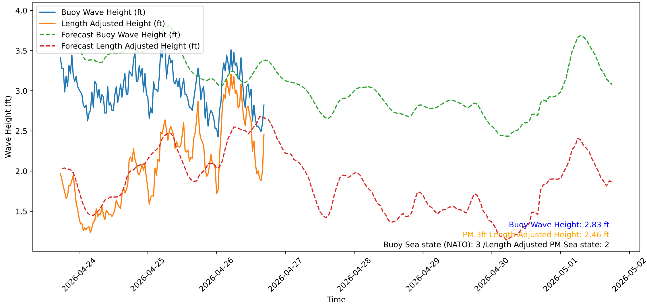
Wave Heights over Time for Green Beach at 2026-04-26 17:31:13
