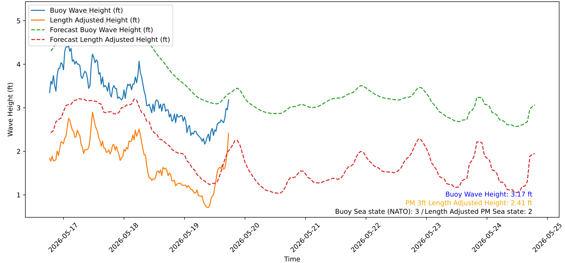
Wave Heights over Time for Green Beach at 2026-05-19 18:31:14
